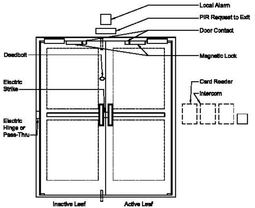
Door Type C - Pair of Opaque or Framed Glass Doors
