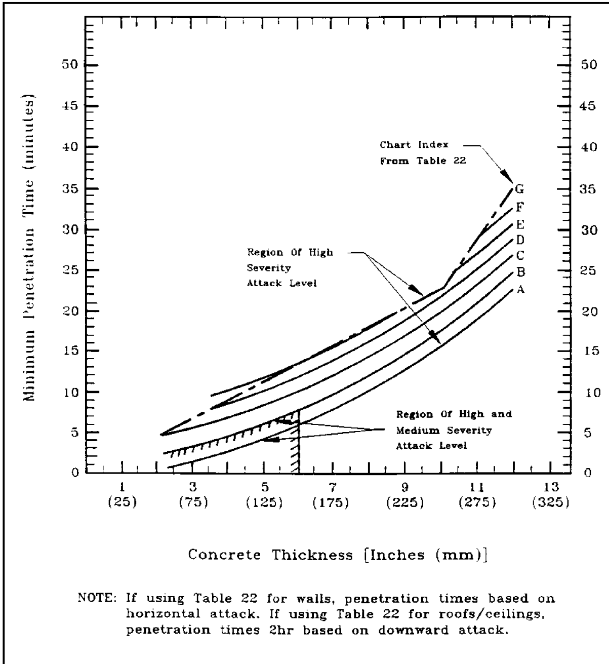
Figure 33 Penetration Times For Conventional Reinforced Concrete Walls/Roofs
