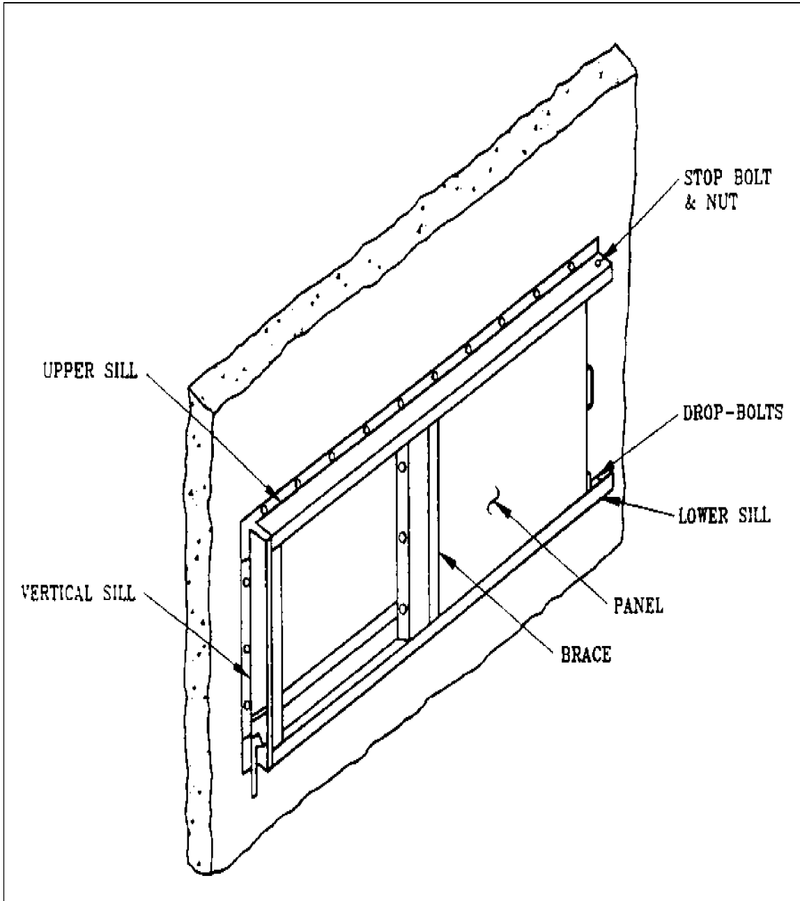
Figure 43 Window Barrier System For High-Severity Threat
