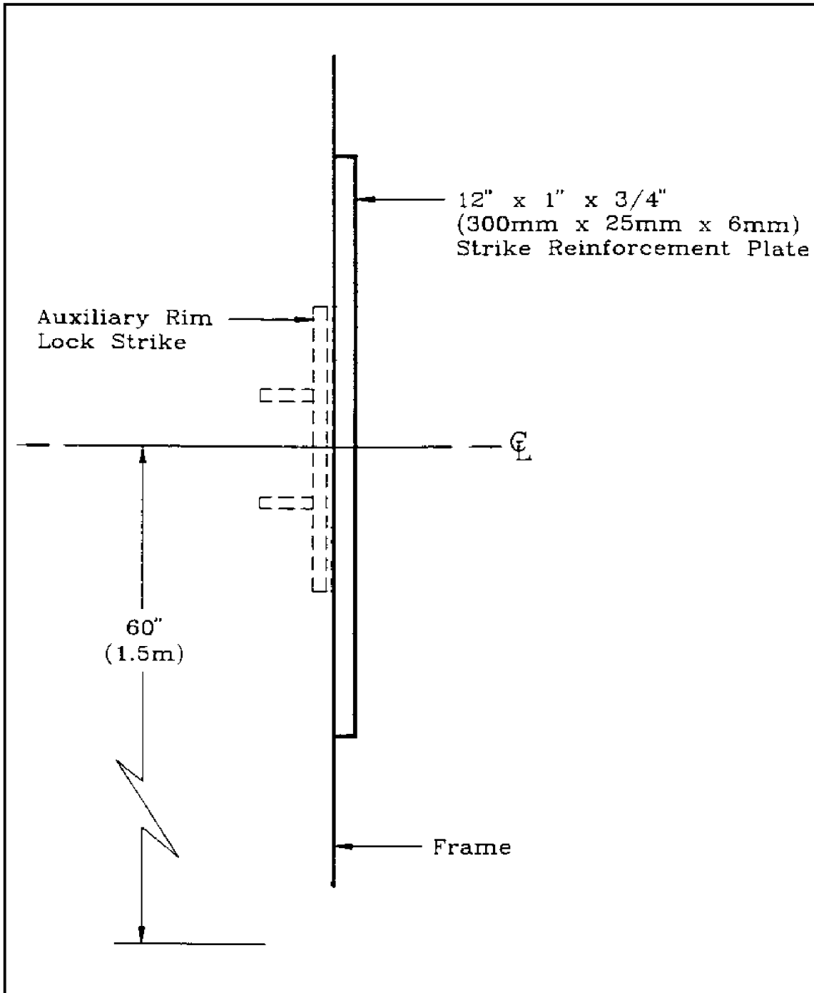
Figure 39 Personnel Door, Auxiliary Rim-Lock Strike Reinforcement
