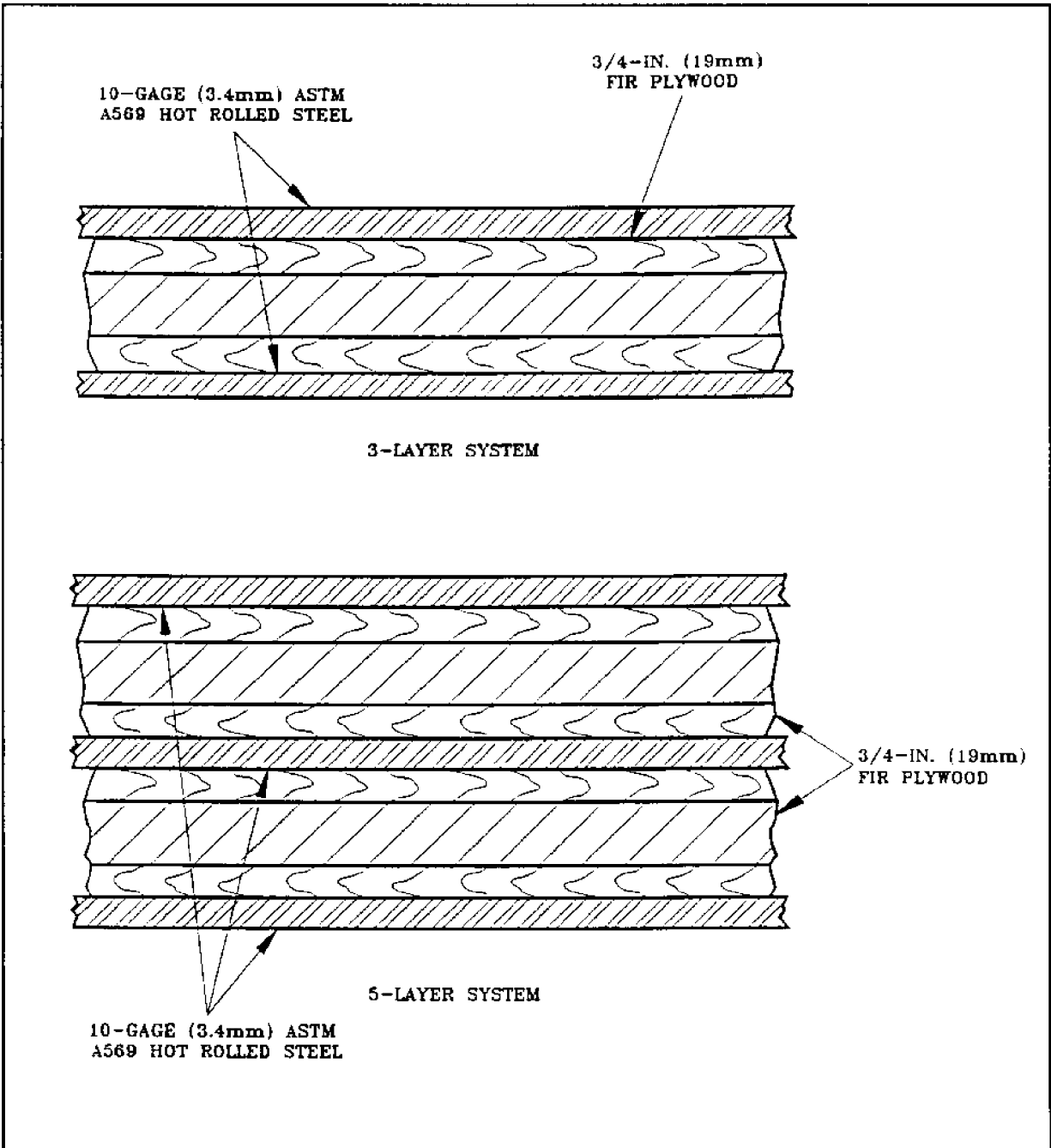
Figure 46 Ten-Gauge (3.4-mm) Hot-Rolled Steel Combinations (MIL-HDBK-1013/5)
