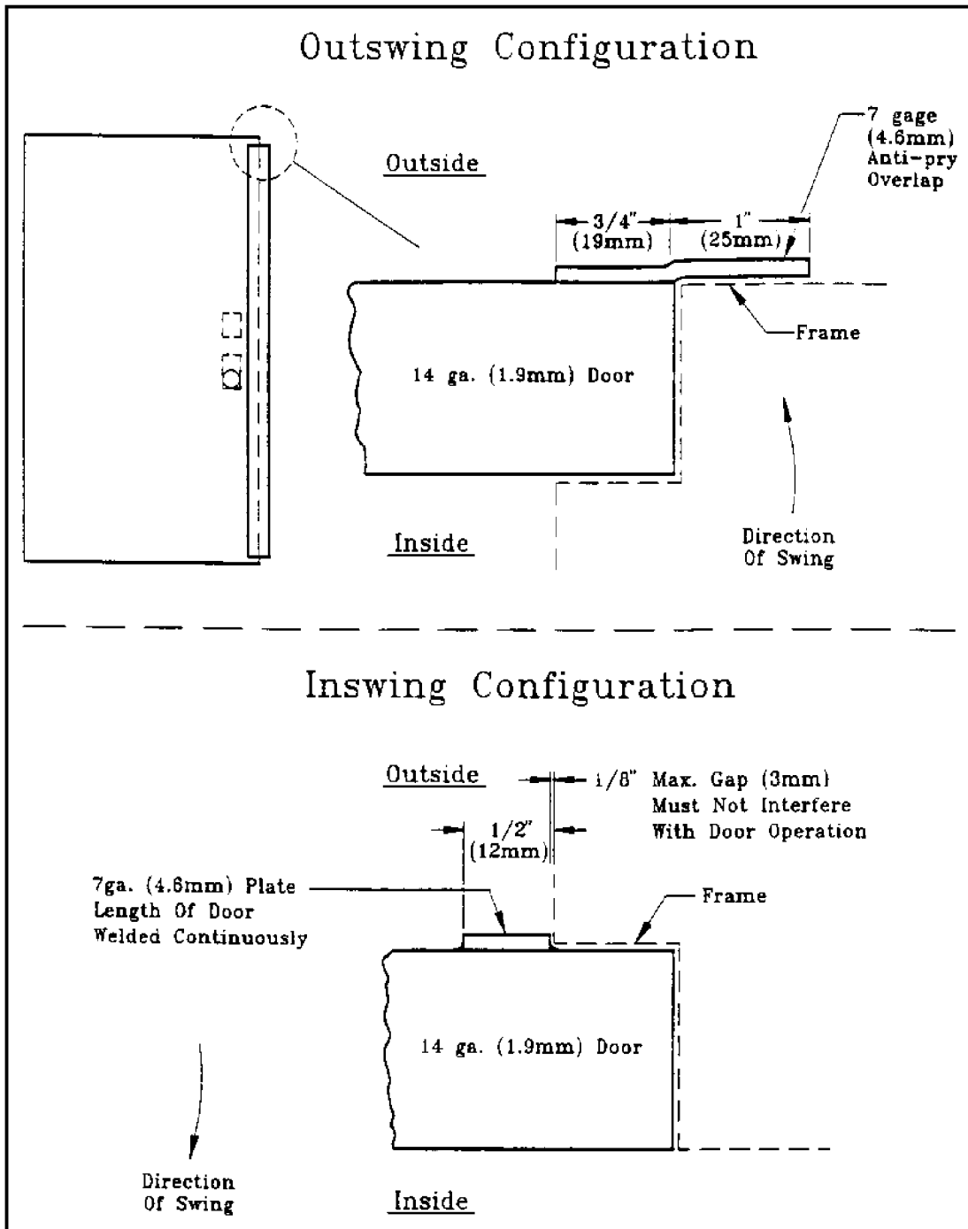
Figure 38 Personnel Door Anti-Pry Strips For Medium-Security Applications
