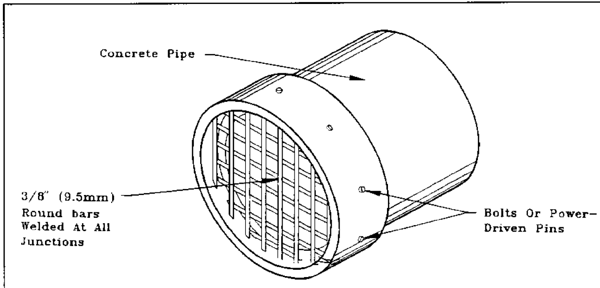
Figure 17 Concrete Culvert Grill (MIL-HDBK 1013/10)
