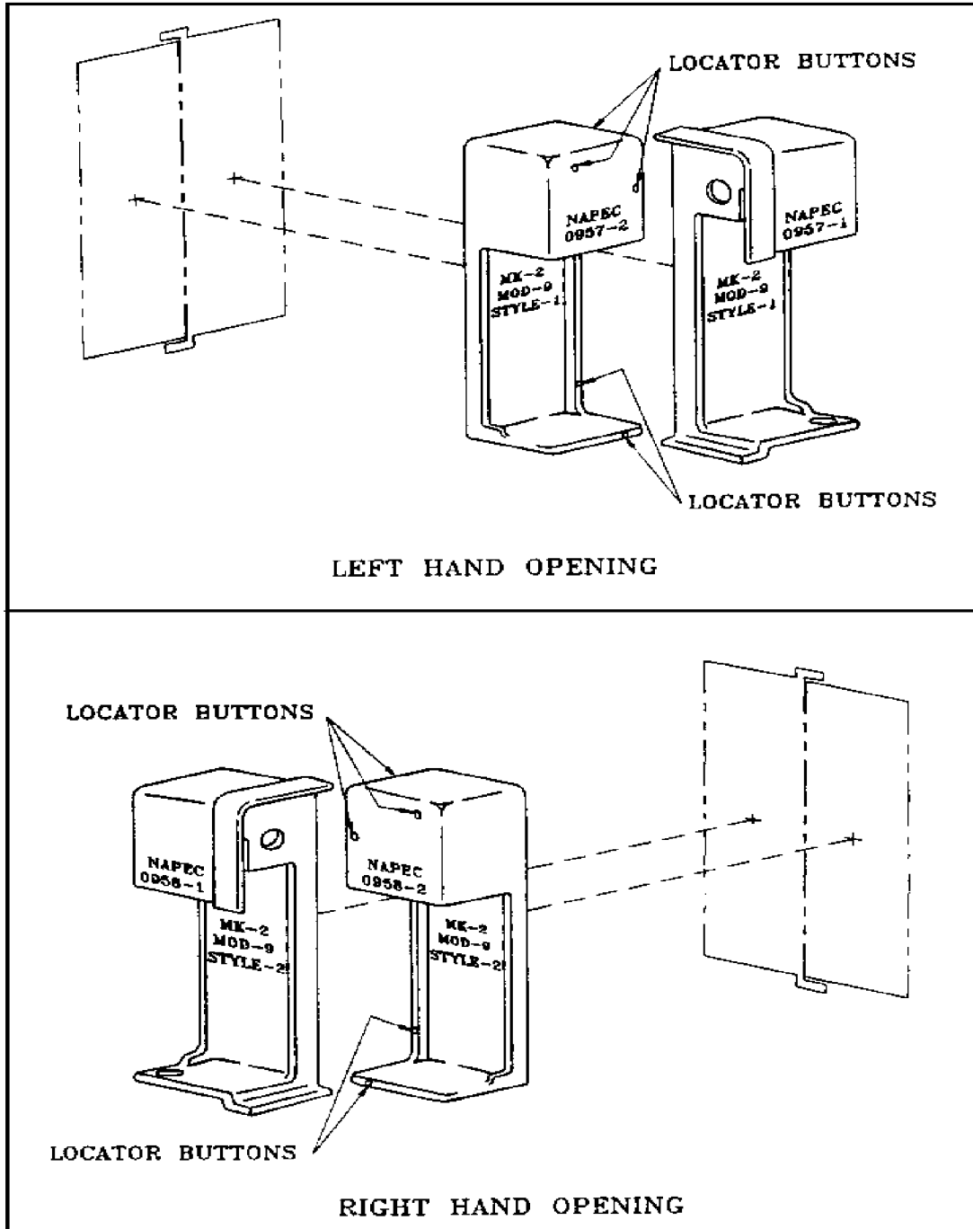
Figure 41 Shrouded Hasp For Padlocks MIL-H-29181
