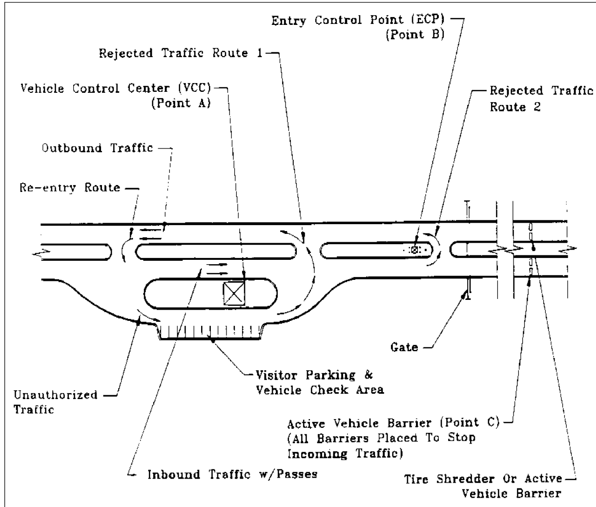
Figure 24 Example Entry Control Point (MIL-HDBK 1013/10)
