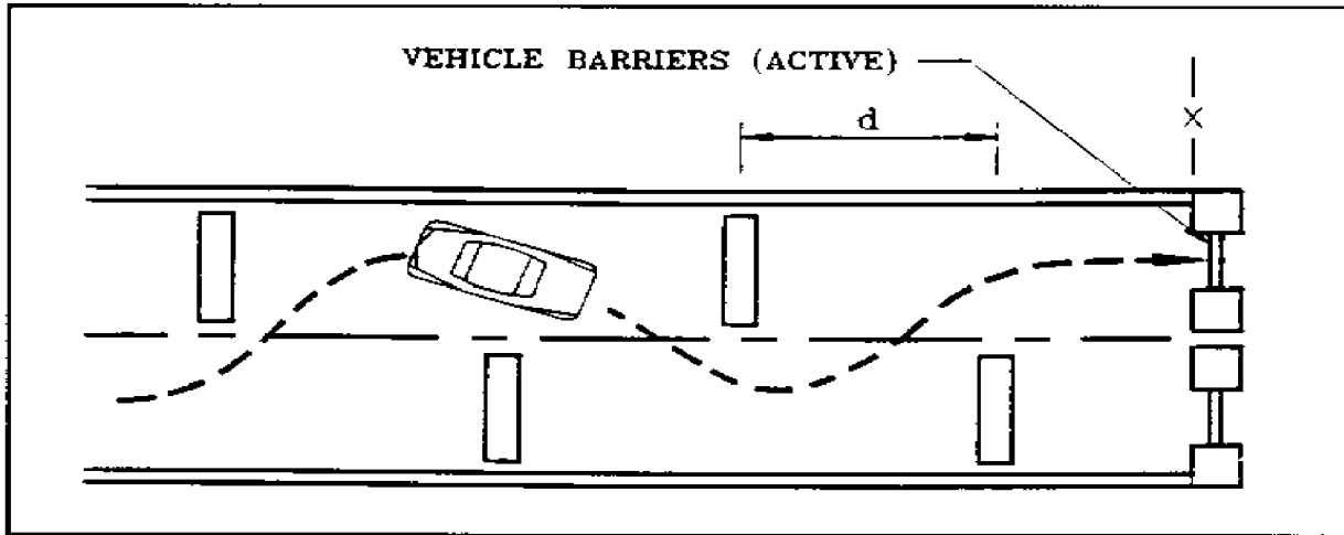
Figure 80 Application of Traffic Obstacles
