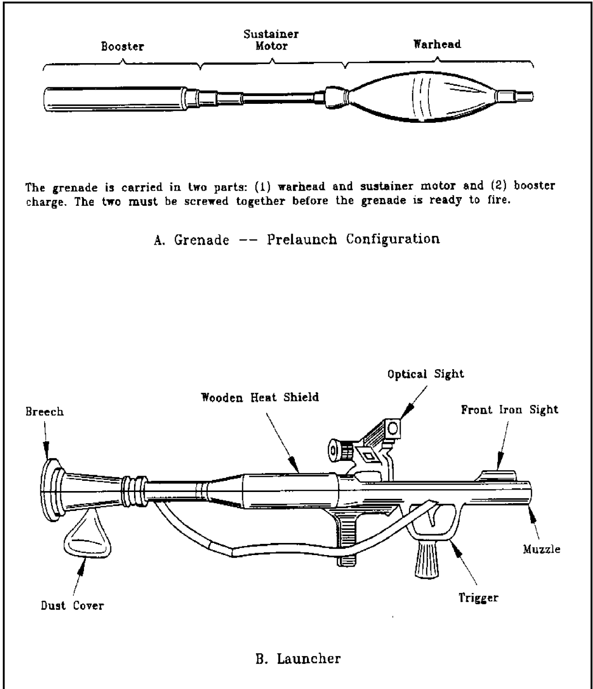
Figure 68 Example Antitank Grenade Launcher Weapon—the Soviet RPG-7
