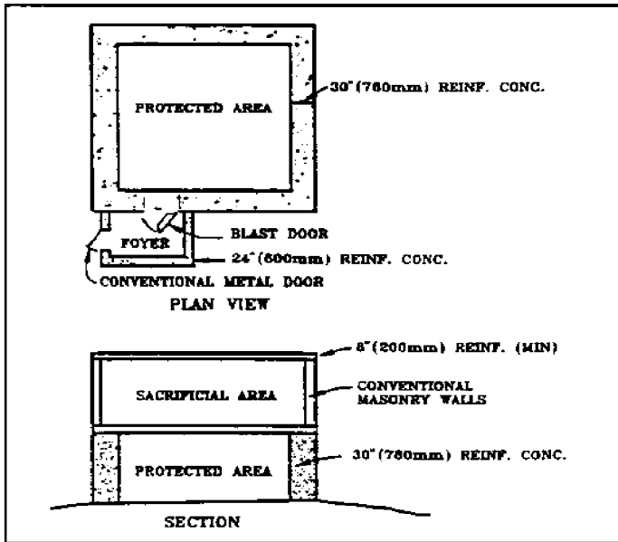
Figure 73 Building Layout Example
