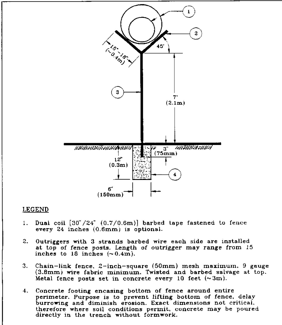
Figure 15 Security Fence Configuration for Nuclear Weapons (DoD 5210.41-M)
