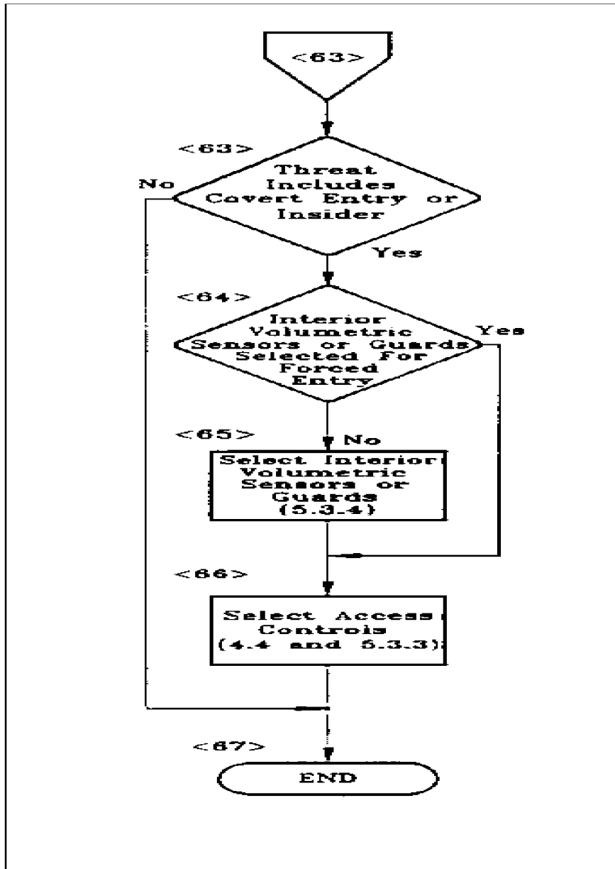
Figure 9 Detailed Design Flowchart (Continued)
