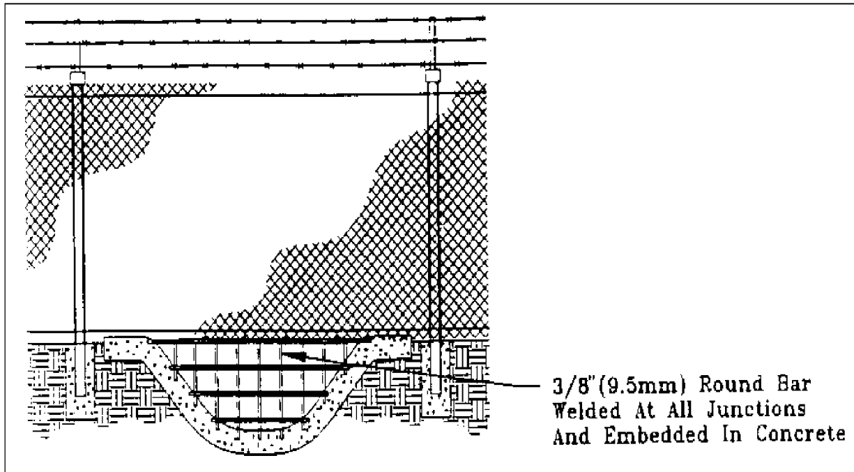
Figure 19 Bar Grill Embedded in Concrete (MIL-HDBK 1013/10)
