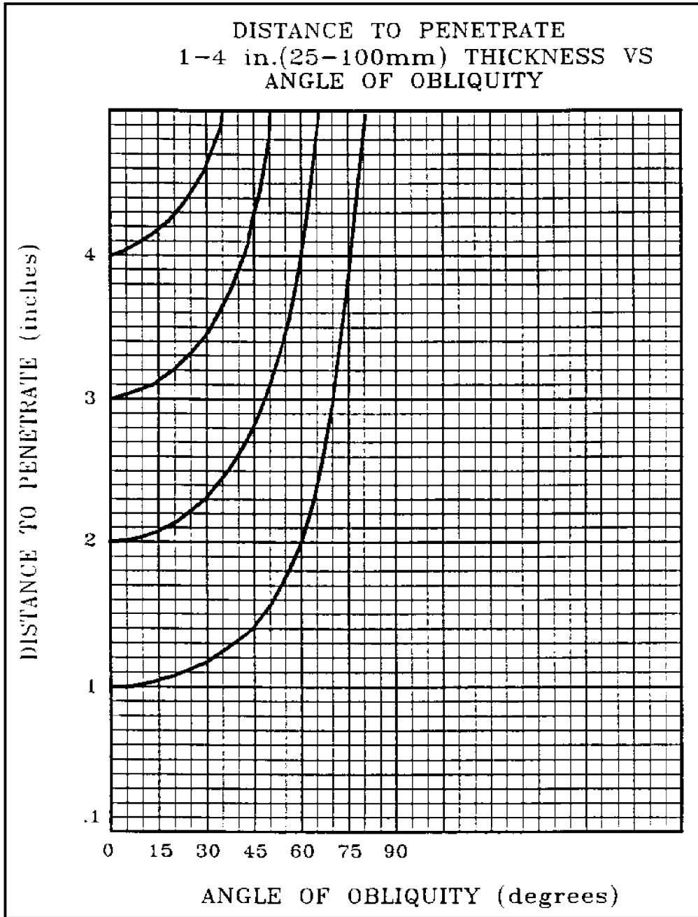
Figure 61 Distance to Penetrate 1 to 4 Inches (25 to 100 mm) Versus Angle of Obliquity
