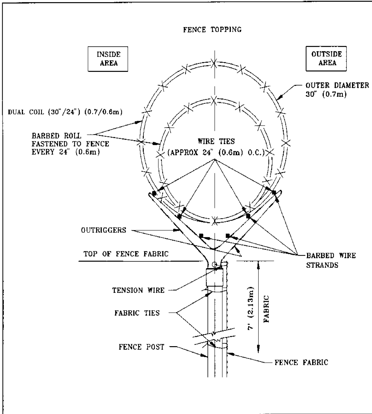
Figure 16 Optional Barbed Roll Topping for Nuclear Weapons (DoD 5210.41-M)
