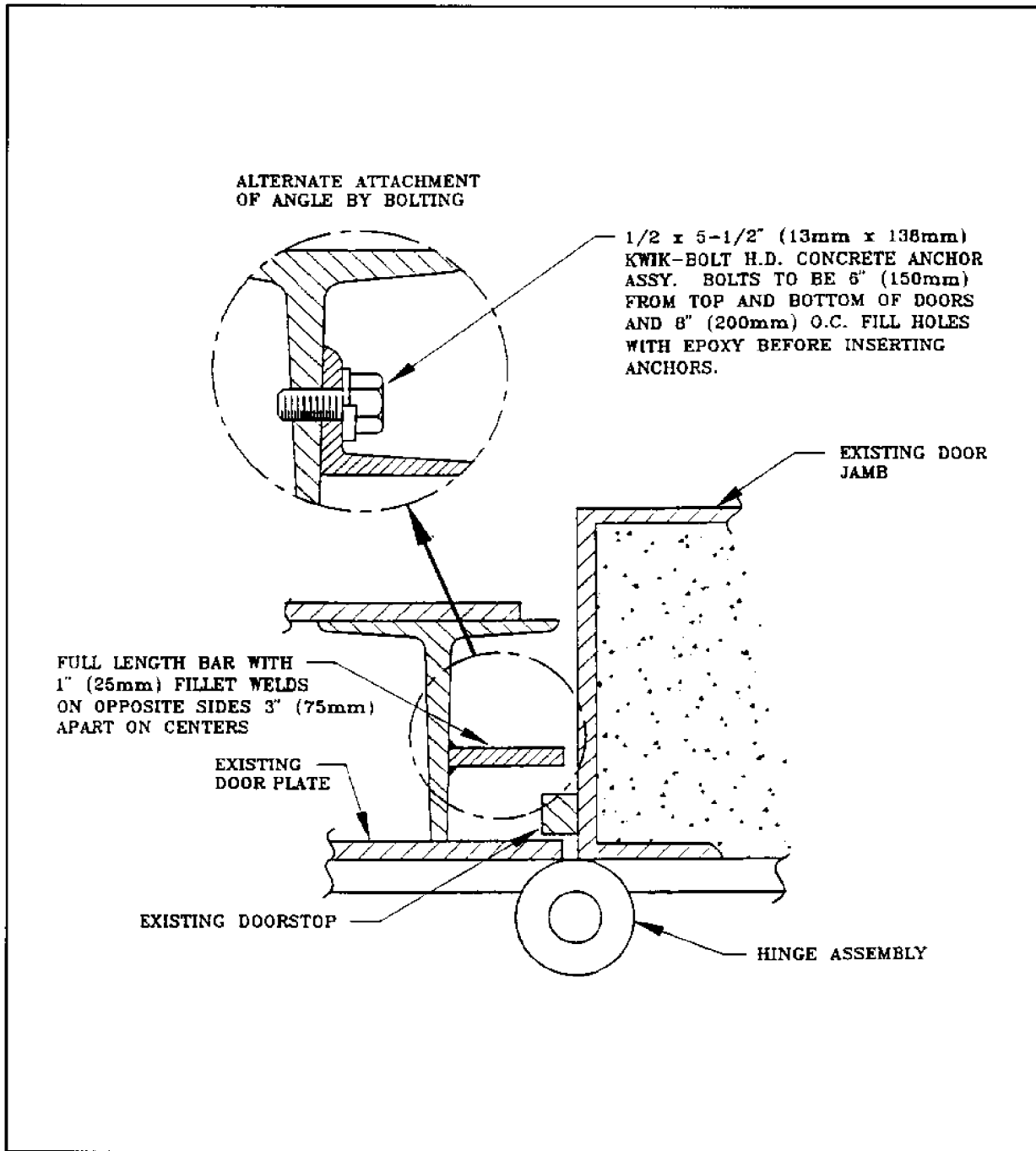
Figure 55 Hinge Side Protection for Hardening Typical Thick Doors by Using an Angle Stop
