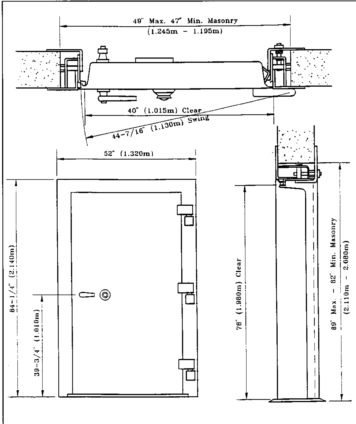
Figure 29 Class 5 Vault Door Dimensions
