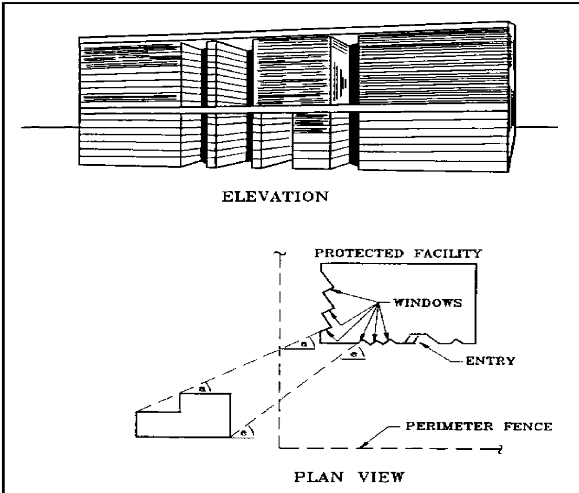
Figure 65 Oblique Window Openings
