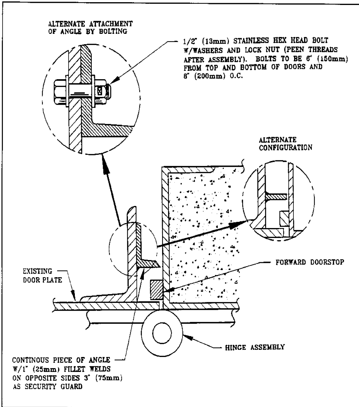
Figure 53 Hinge Side Protection for Doors Using a Forward Doorstop with Angle
