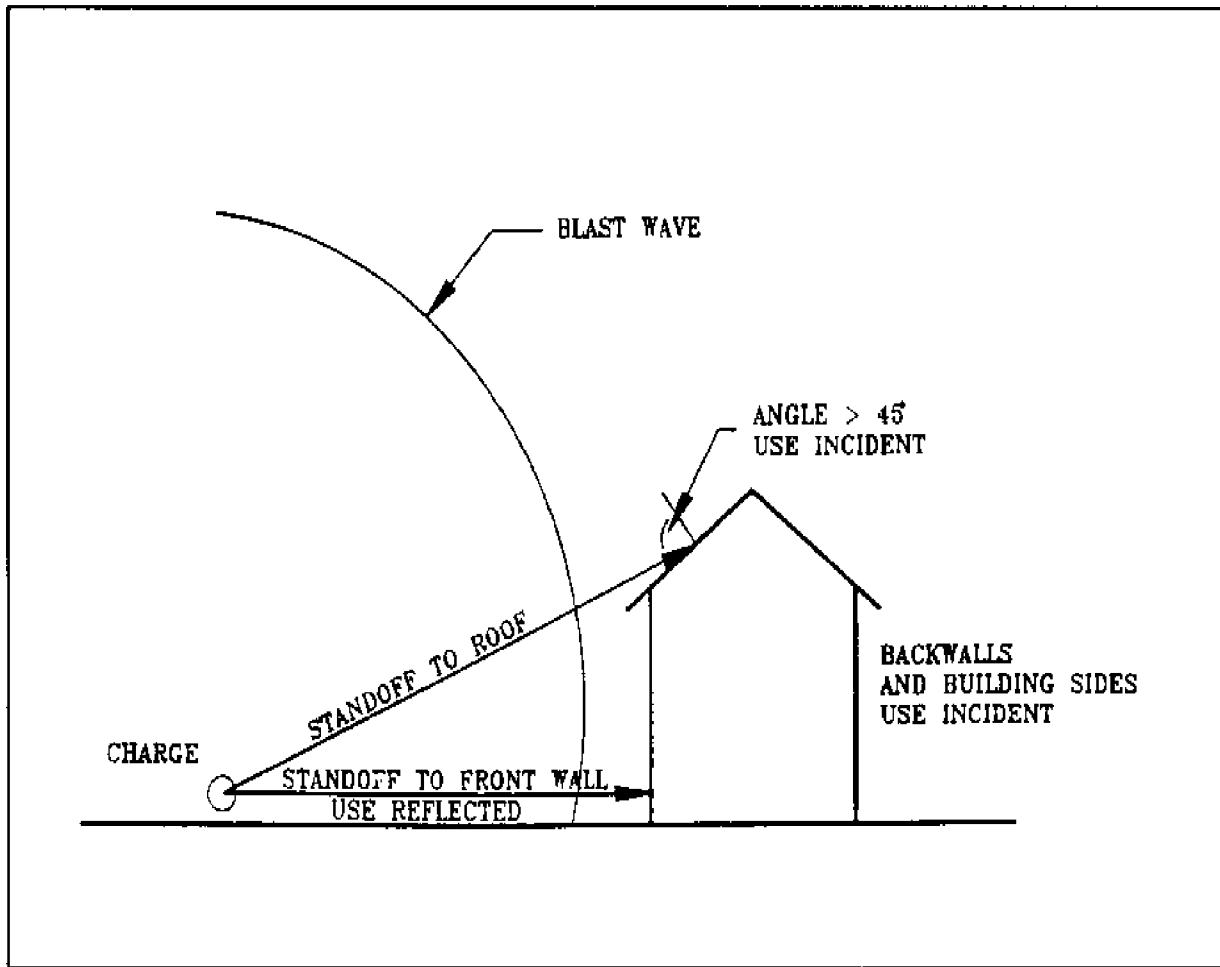
Figure 76 Blast Wave Geometry
