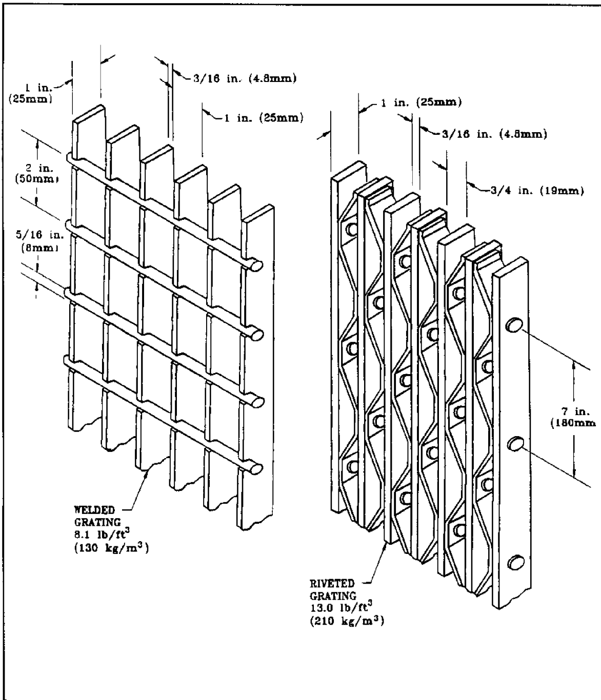
Figure 49 Typical Gratings (MIL-HDBK-1013/4)
