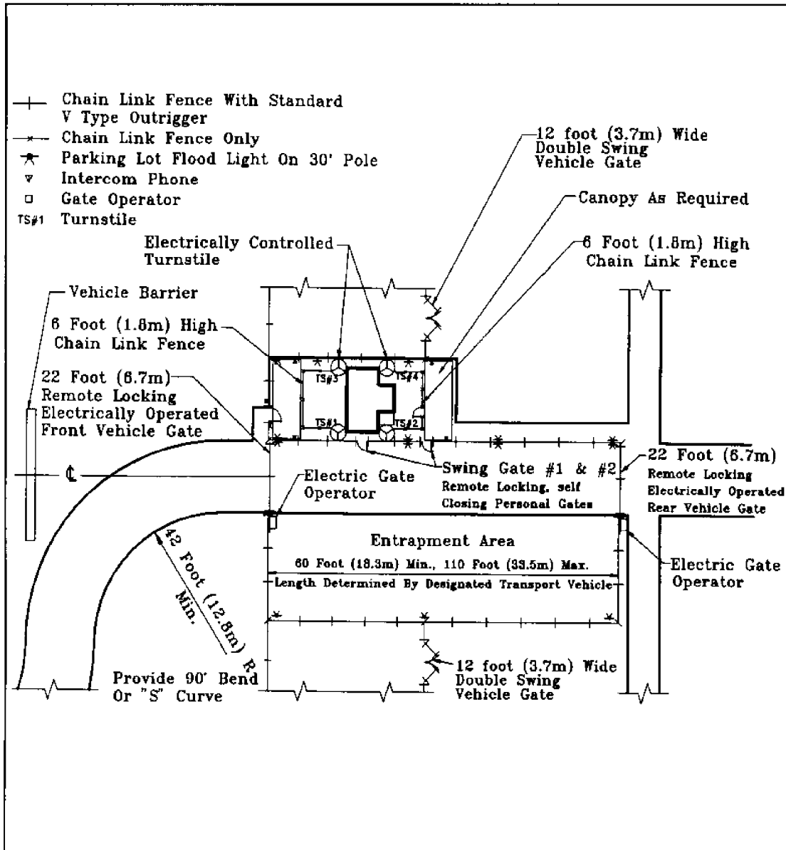
Figure 25 Nuclear Weapons Storage Site Entry Control Facility (MIL-HDBK 1013/10)
