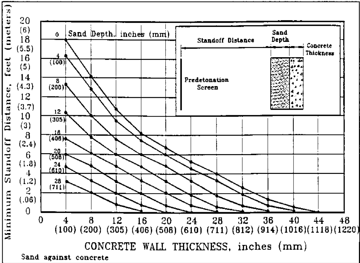
Figure 69 RPG Hardening-Concrete/Sand Thickness Verses Standoff Distance
