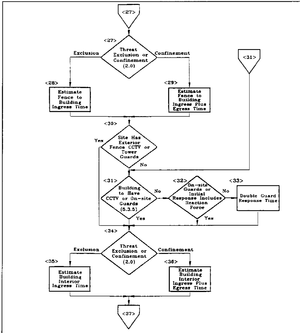
Figure 9 Detailed Design Flowchart (Continued)
