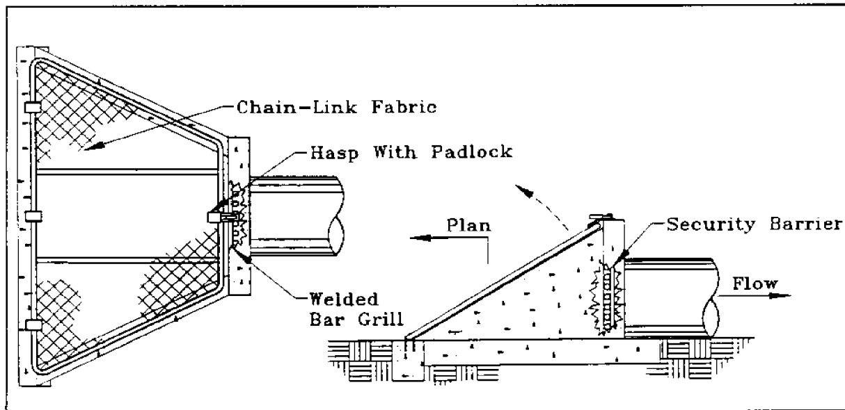
Figure 18 Removable Grating for Culverts (MIL-HDBK 1013/10)
