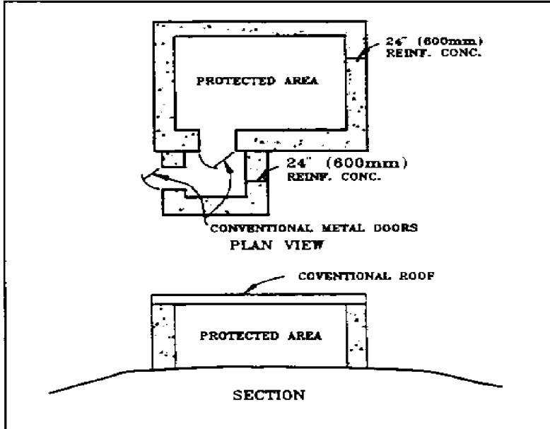
Figure 71 Building Layout Example
