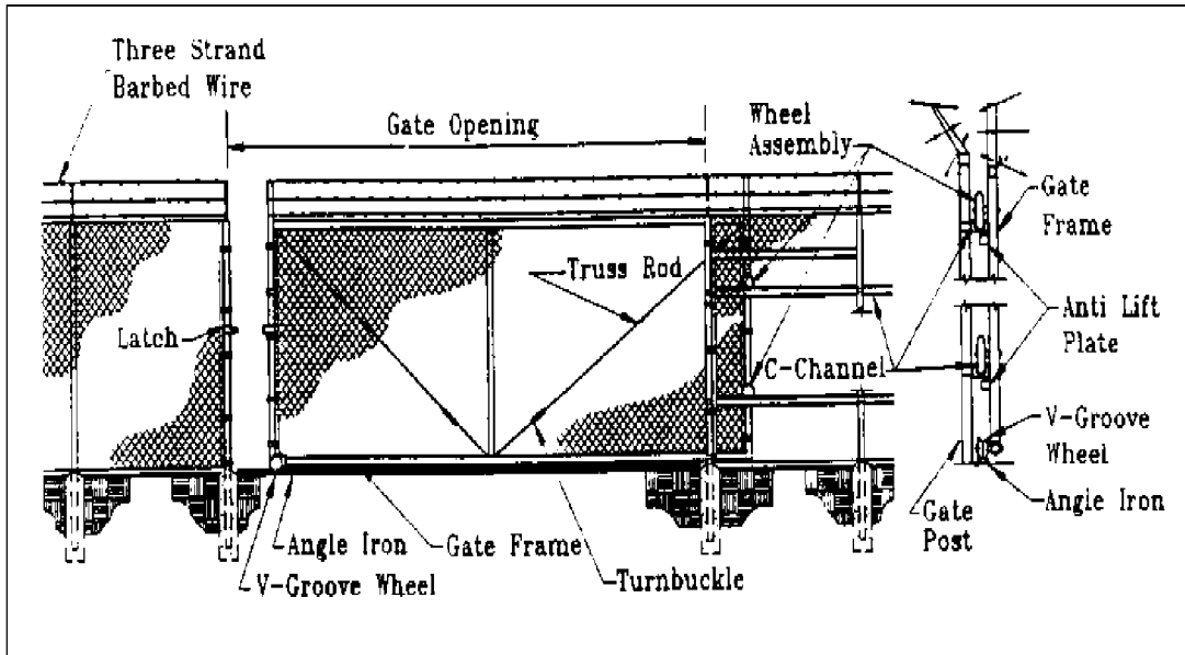
Figure 22 Single Wheel-Supported (V-Groove) Sliding Gate (MIL-HDBK 1013/10)
