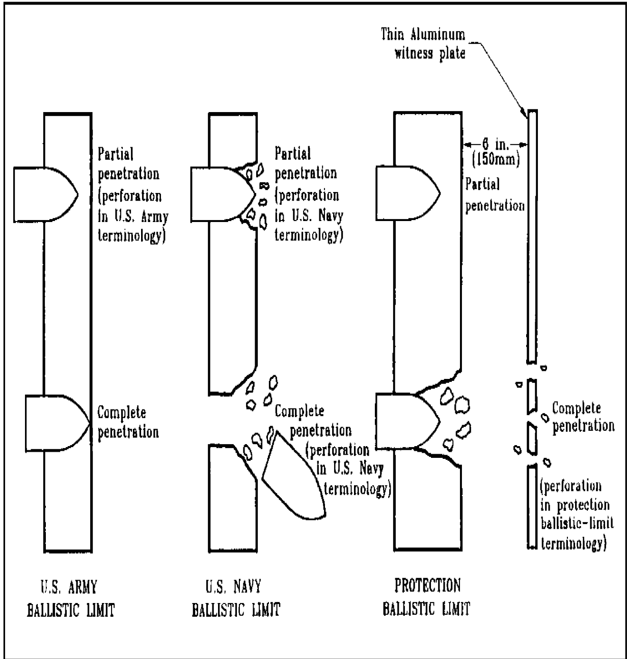
Figure 60 Ballistic Limit Criteria
