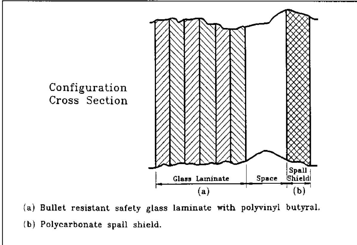
Figure 66 Example of High-Severity-Ballistic-Threat Bullet-Resistant Glass Cross Section
