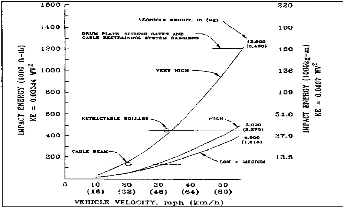
Figure 83 Moving Vehicle Impact Energy Versus Velocity (Active Barriers).
