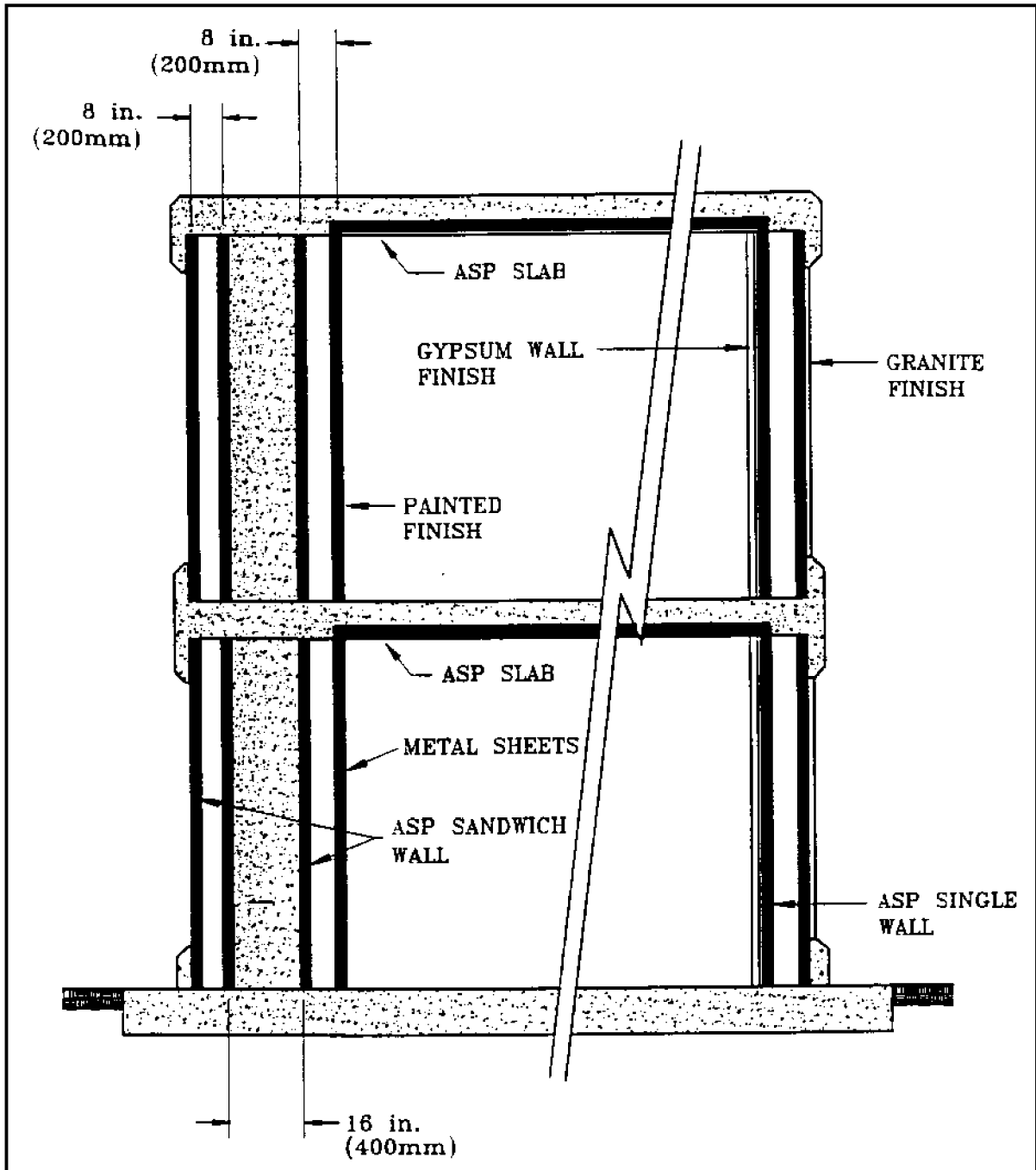
Figure 70 ASP Walling System
