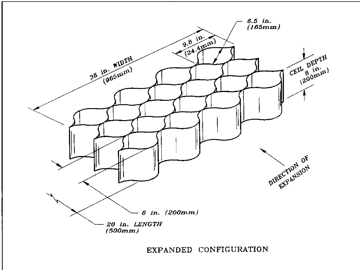
Figure 74 Standard Sand-Grid Materials (from Army Technical Report SL-88-39, Expedient Field Fortifications Using Sand-Grid Construction )
