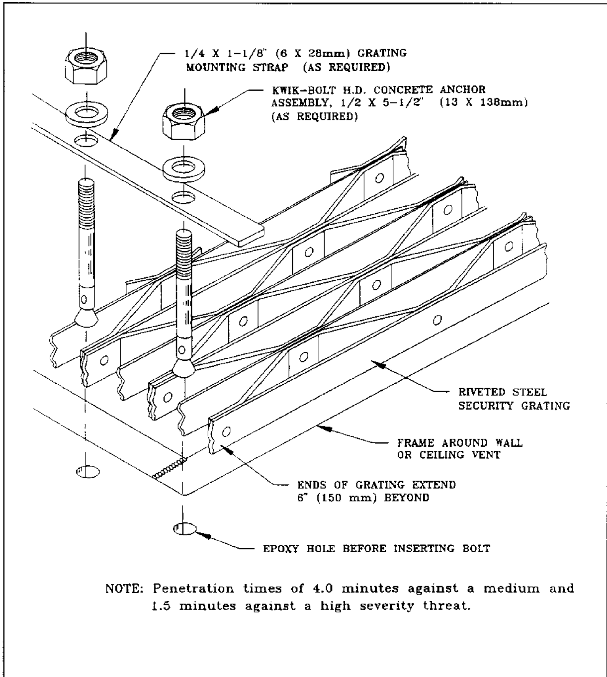
Figure 59 Security Intrusion Protection Plan for Hardening a Typical Wall or Ceiling
