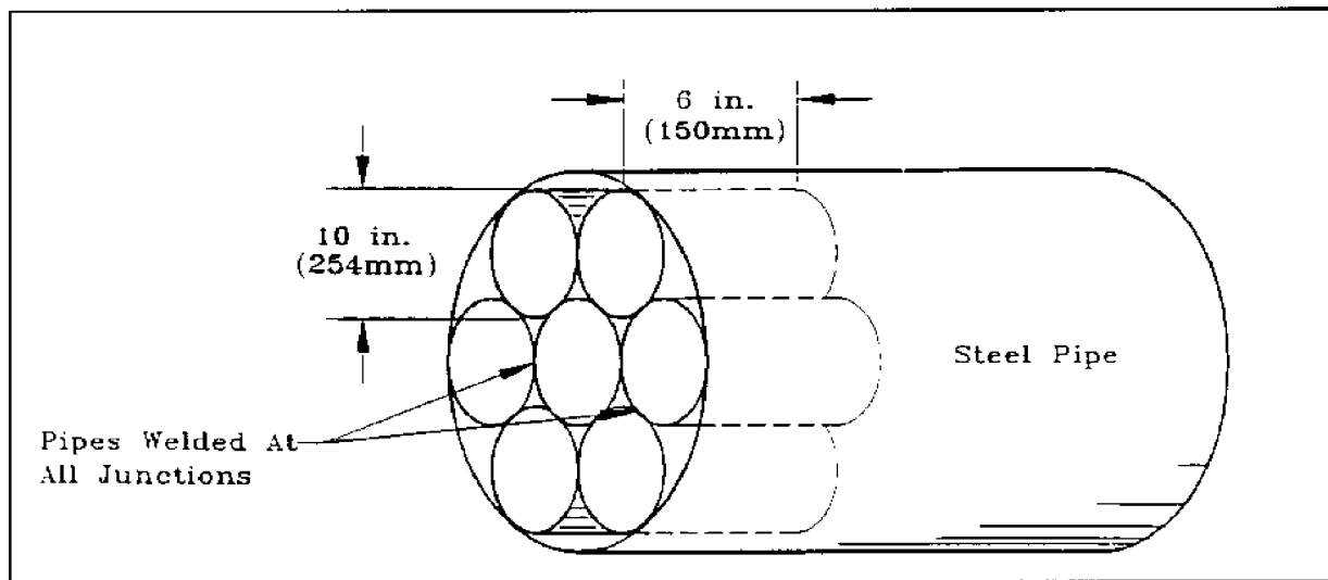
Figure 20 Large Culvert with Short Honeycomb Pipes (MIL-HDBK 1013/10)
