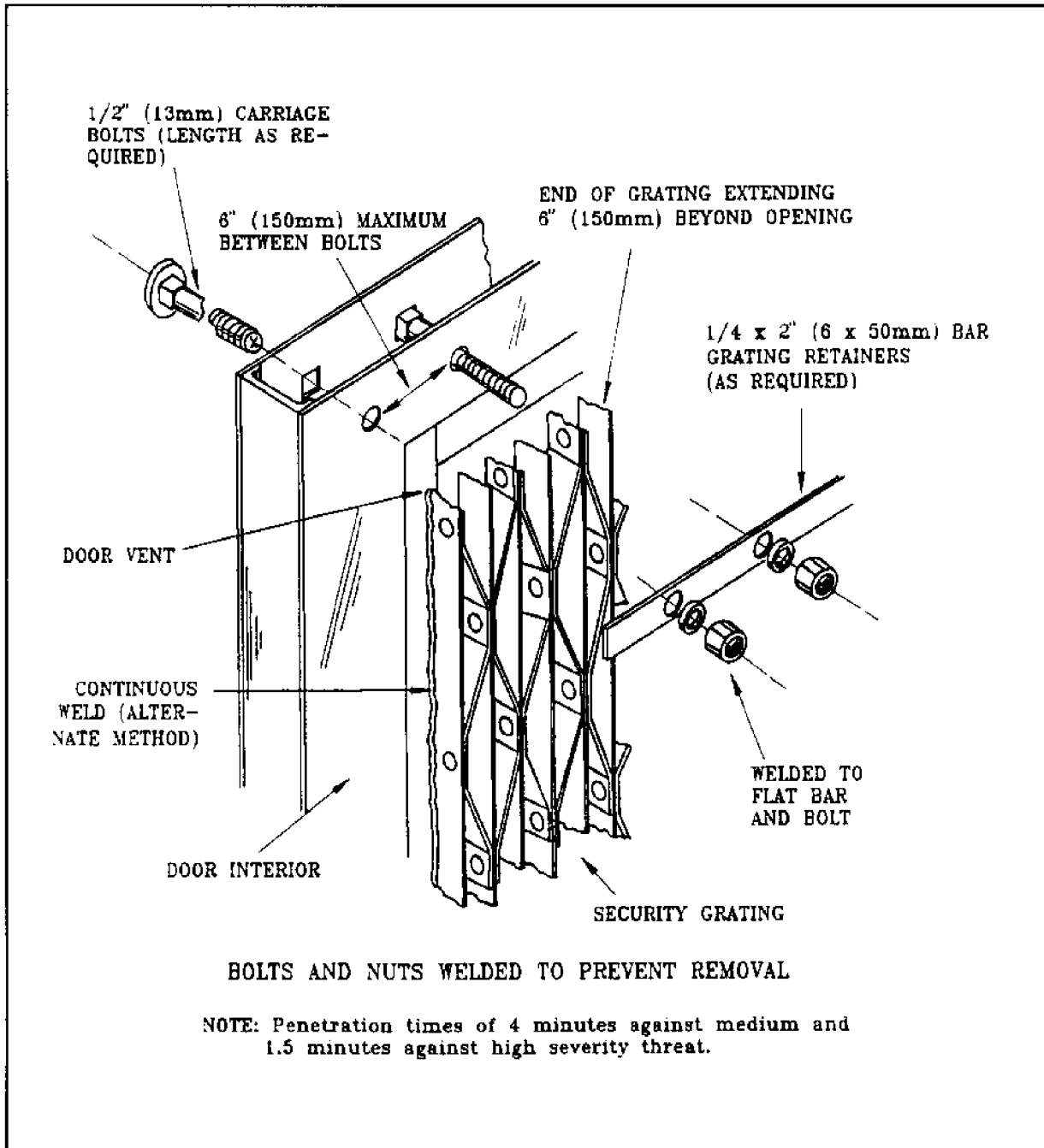
Figure 57 Security Intrusion Protection Plan for Hardening a Typical Door Ventilator
