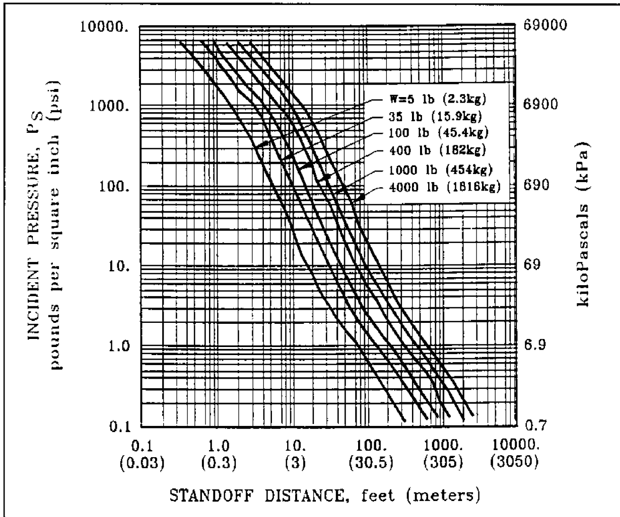
Figure 77 Pressure Levels Versus Standoff Distance
