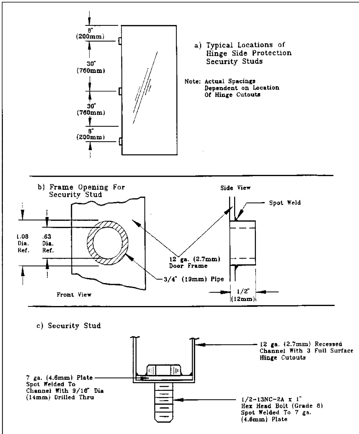
Figure 36 Personnel Door Hinge Side Protection for Low- and Medium-Severity Threat
