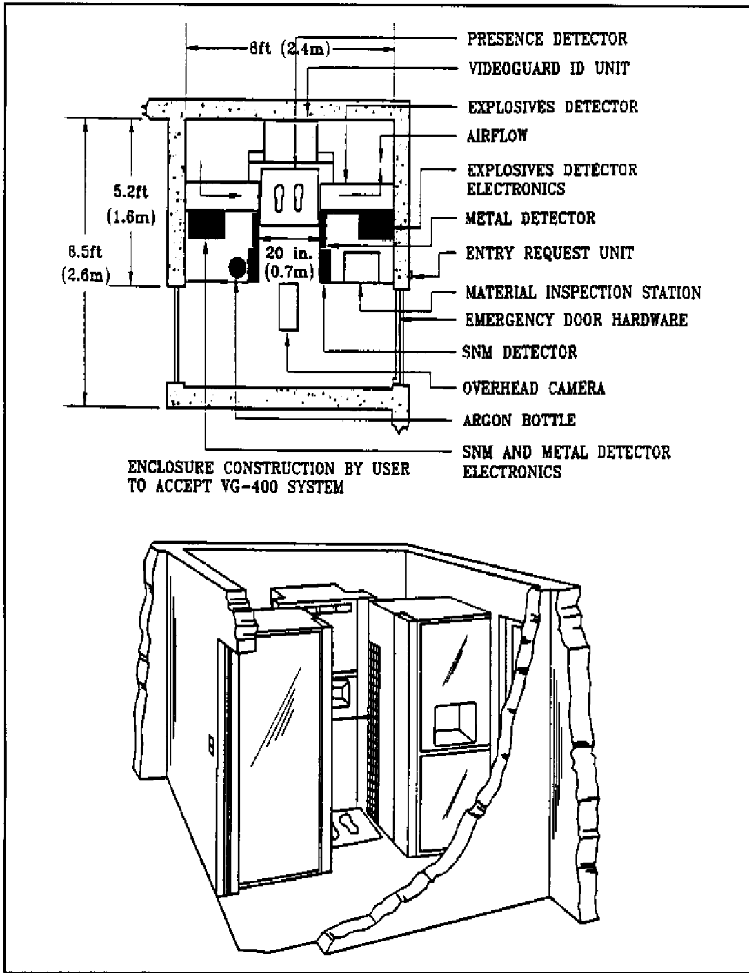
Figure 26 Example Portal Structure for Access Control
