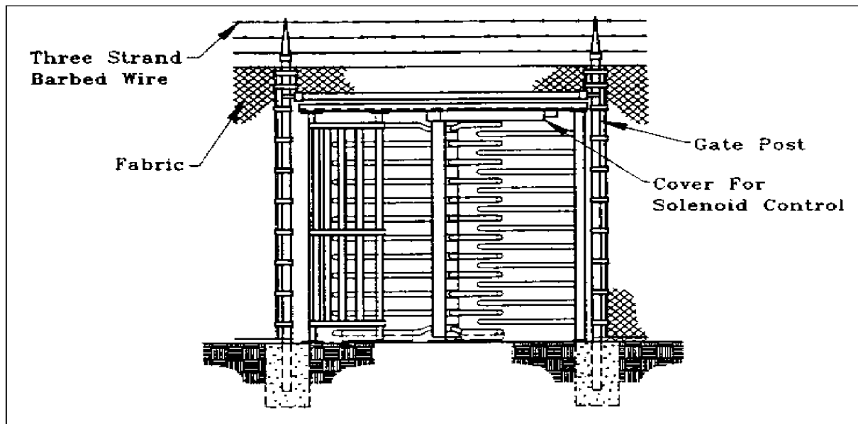
Figure 21 Turnstile (Rotational) Personnel Gate (MIL-HDBK 1013/10)
