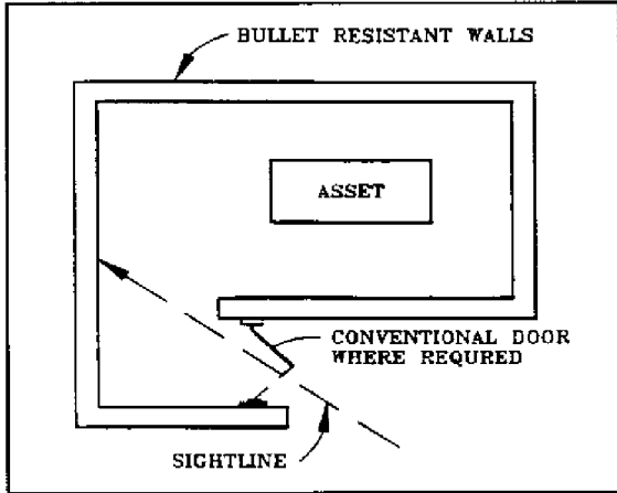
Figure 63 Wall Arrangement to Block Sightlines
