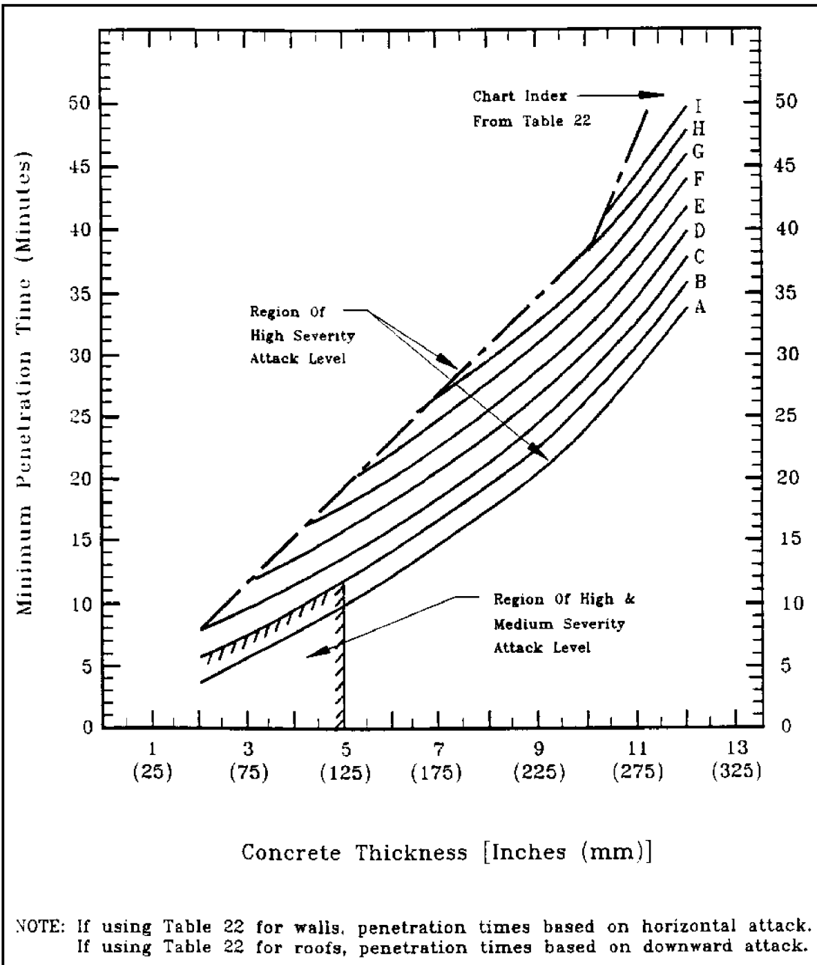
Figure 34 Penetration Times For Fibrous Reinforced Concrete Walls/Roofs
