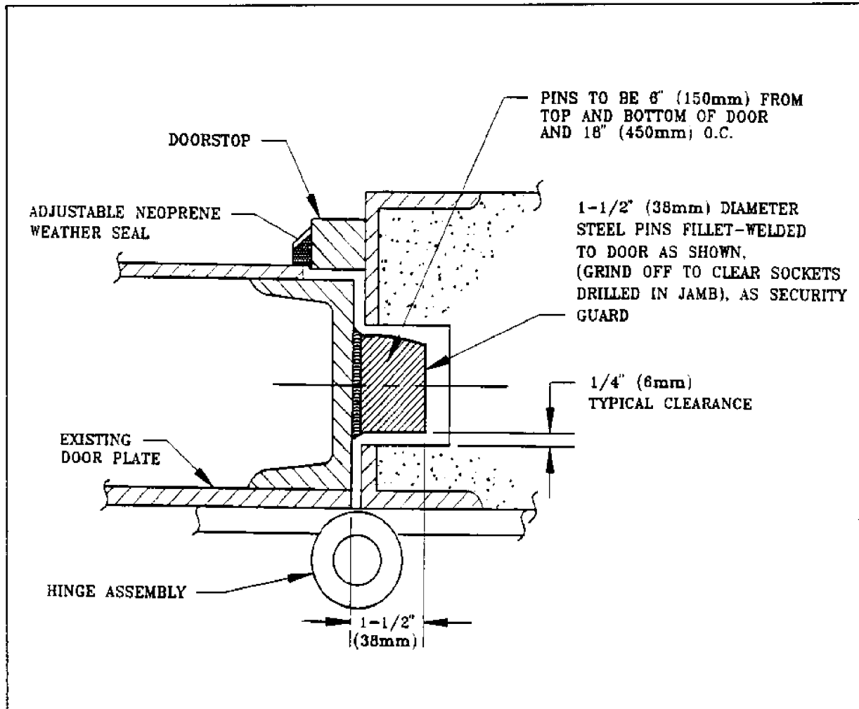
Figure 52 Hinge Side Protection Plan for Using a Pin-In-Socket Technique
