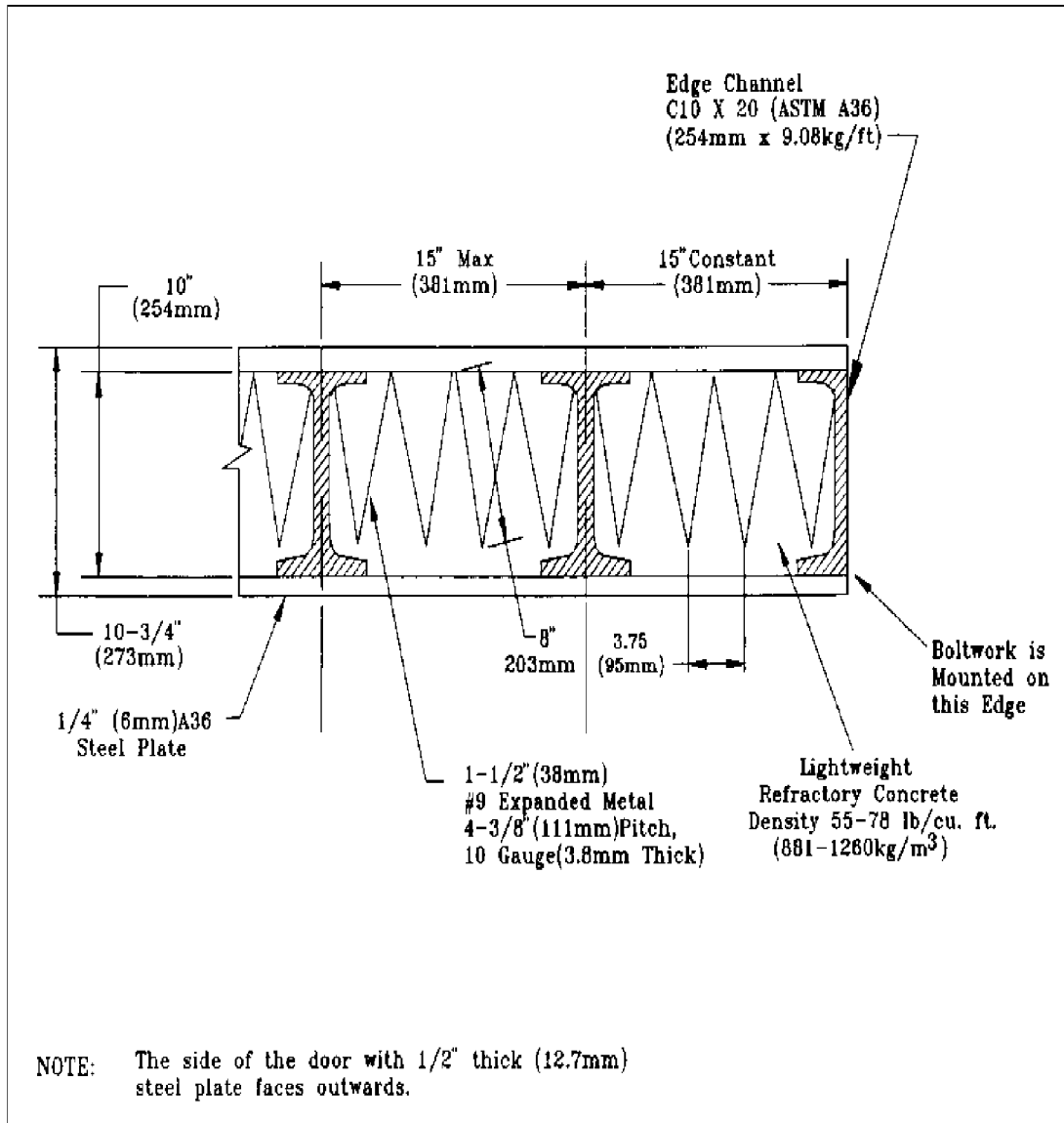
Figure 42 Magazine Door Panel Cross Section For Very High-Severity Threat
