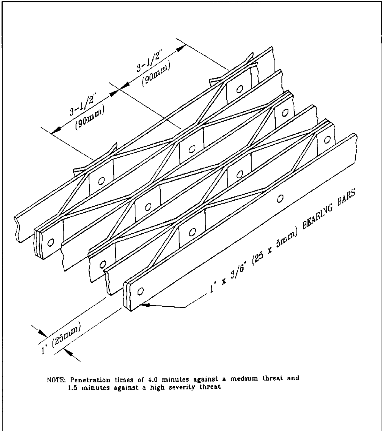
Figure 56 Riveted Steel Grating
