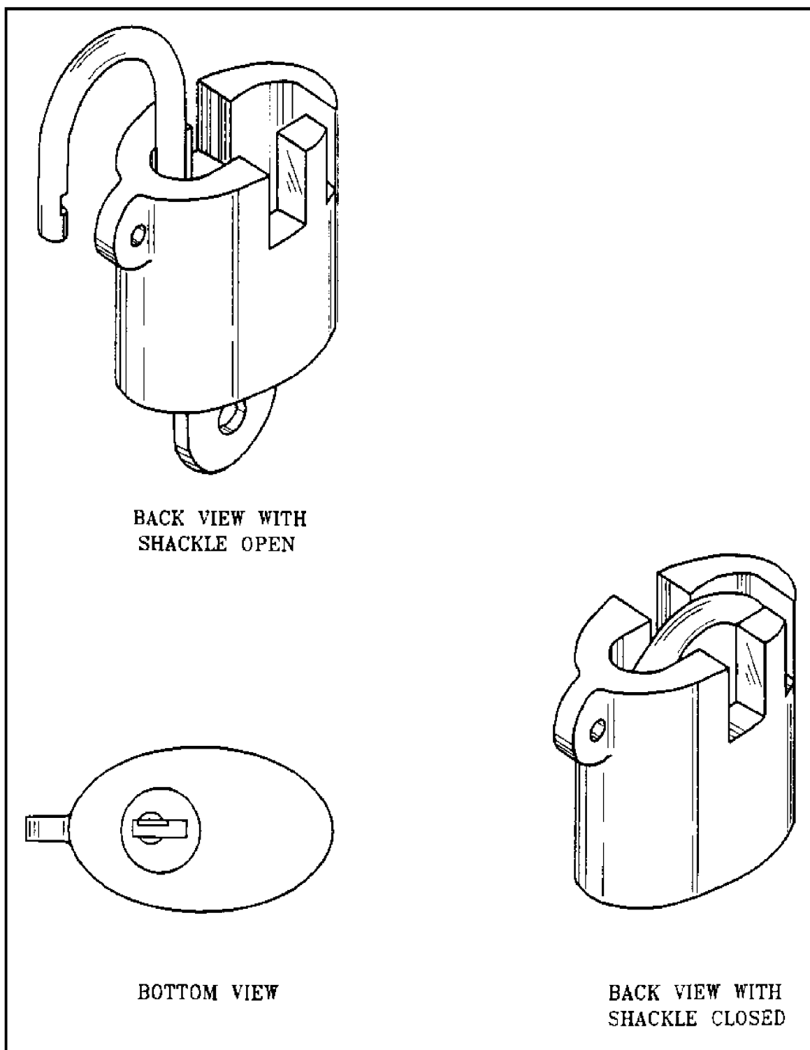
Figure 40 Shrouded Key Operated Shackle Padlock Per MIL-P-43607
