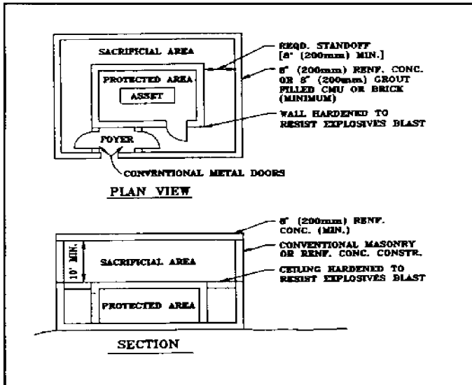
Figure 72 Building Layout Example
