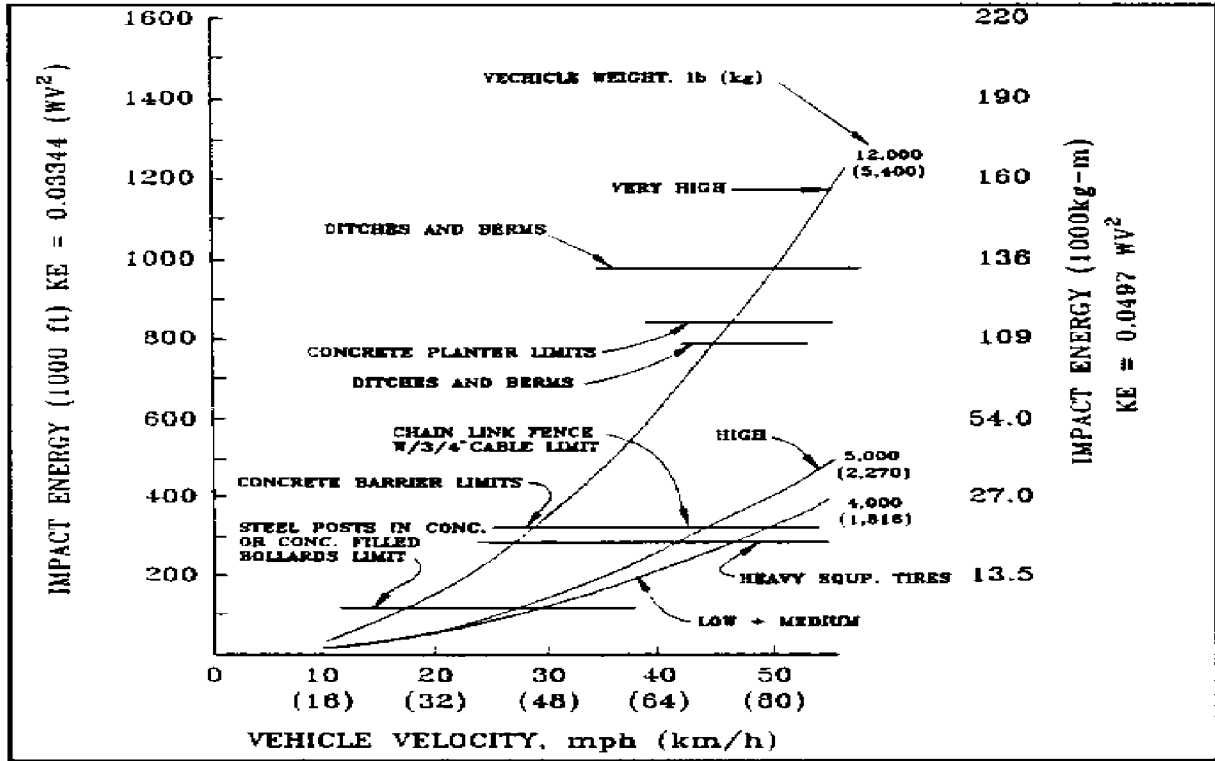
Figure 82 Moving Vehicle Impact Energy Versus Velocity (Passive Barriers)
