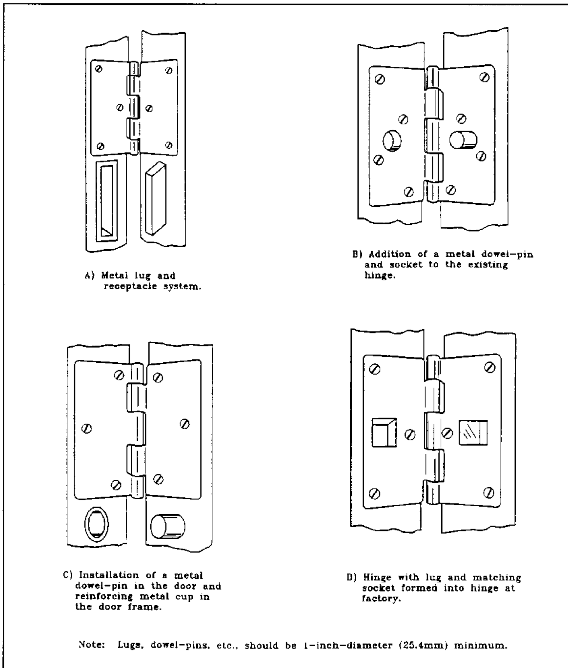
Figure 37 Personnel Door, Representative Medium-Security Hinge-Side Protection
