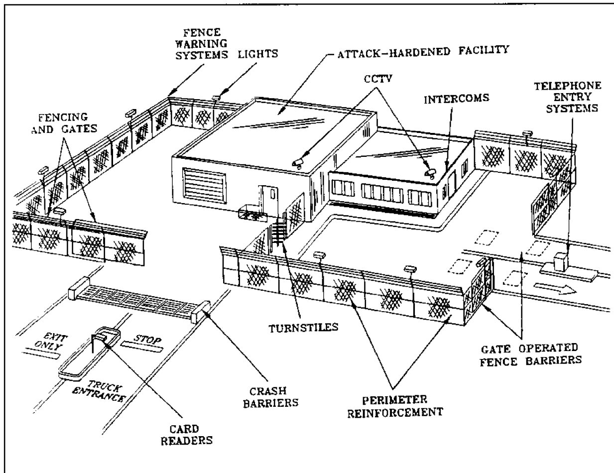
Figure 4 Integrated Physical Security System
