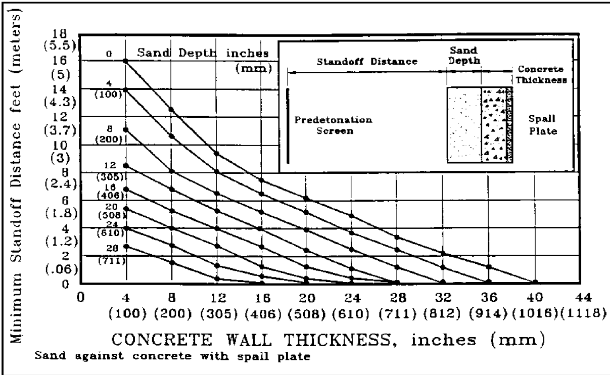
Figure 75 Retrofit Hardening—Concrete/Sand Thickness Versus Distance
