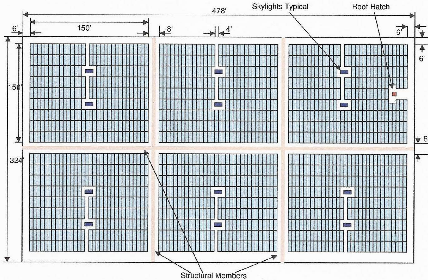
Figure 1. PV Array Example: Large Commercial Building (Axis > 250 ft.). 8 ft. walkways
