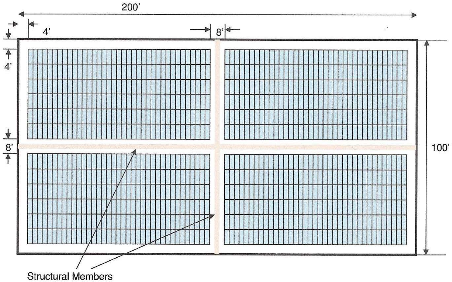
Figure3. PV Array Example: Small Commercial Building (Axis < 250 ft.). 8 ft. walkways
