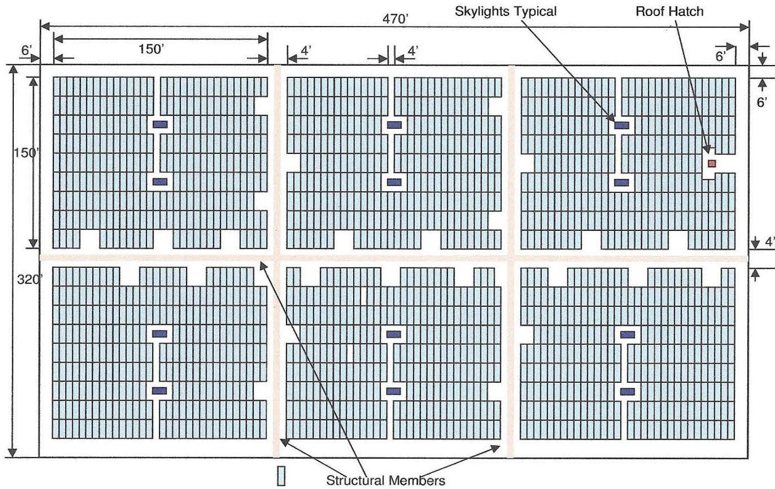
Figure 2. PV Array Example: Large Commercial Building (Axis > 250 ft.). 4 ft. walkways
