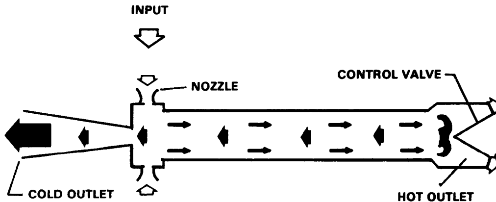
SCHEMATIC DRAWING OF A VORTEX TUBE
