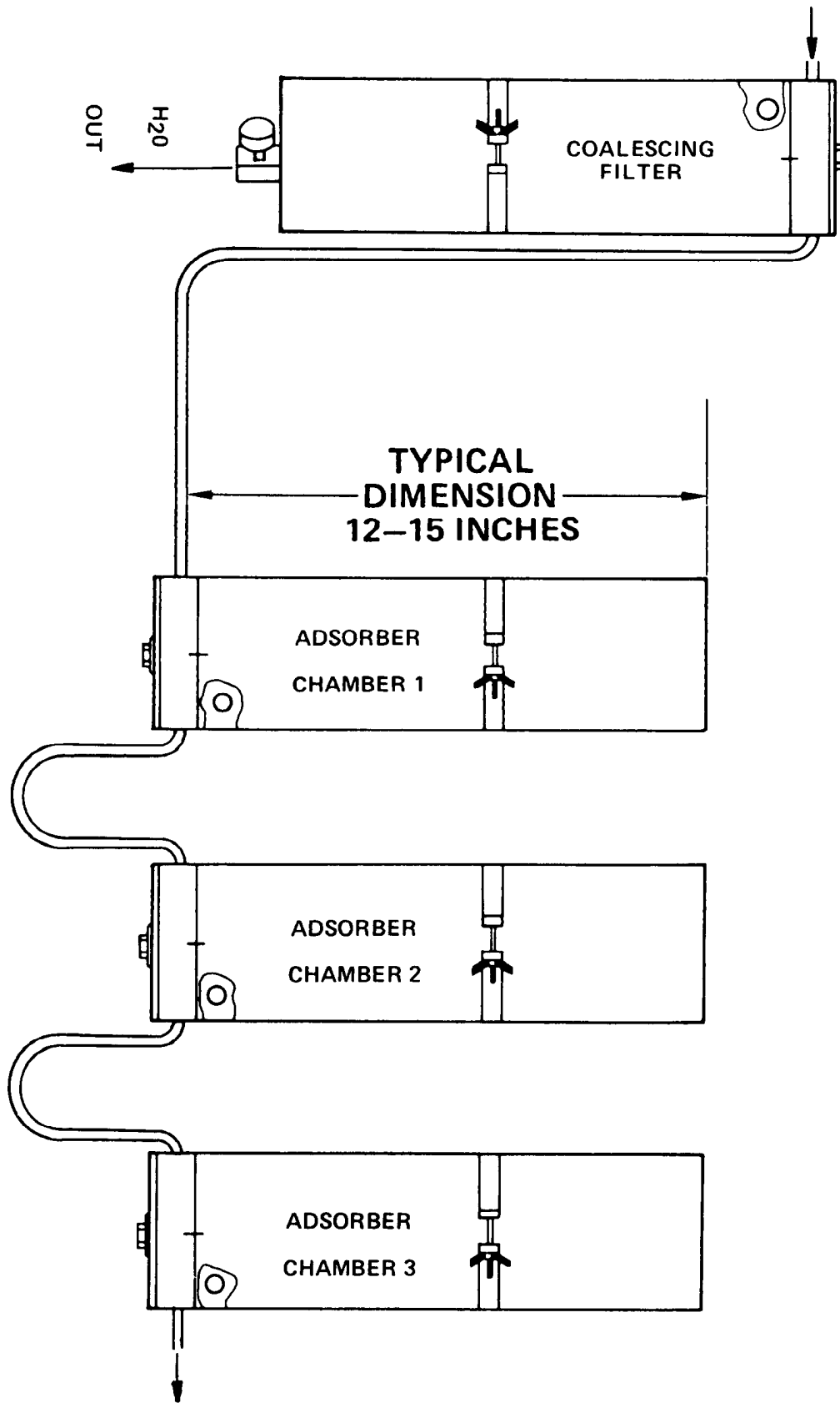
Figure F6. Typical High Pressure Purifier Assembly
