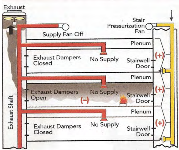
Figure 12.11. A diagram of an exhaust system (left) and a stair pressurization system (right).
