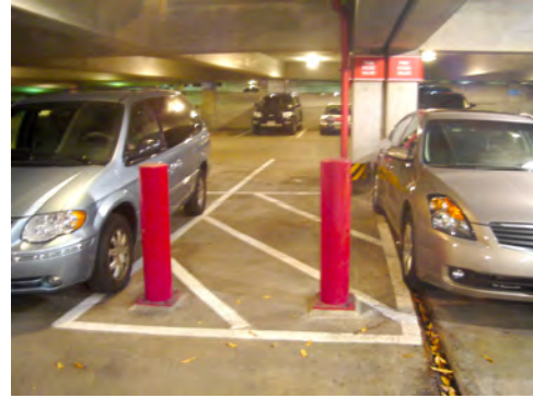
Figure 9.11. Floor striping indicates a FHC access path in a parking garage. Bollards provide vehicle impact protection. Bright signs at the top of the columns help firefighters locate the FHC.
