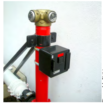
Figure 10.6. An FDC with locked plugs. The key is in the key box below the inlets.
