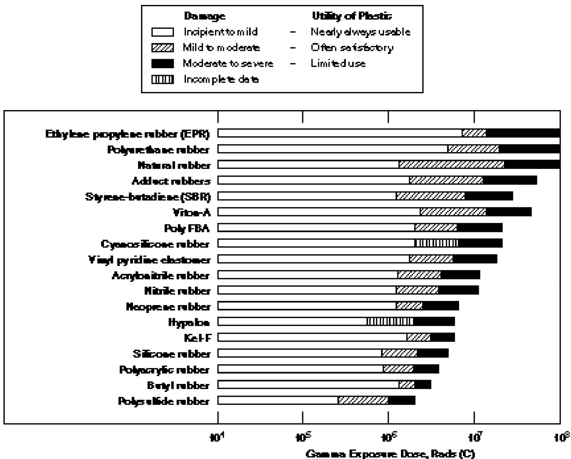
FIGURE 3. Relative radiation resistance of elastomers.
