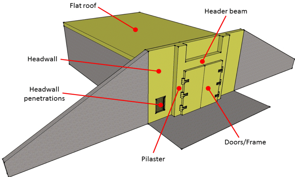
Figure 2-2: Typical ECM Blast Resisting Elements
