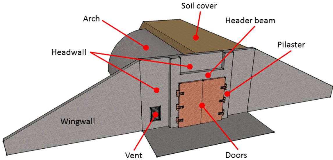
Figure 2-1: ECM Components
