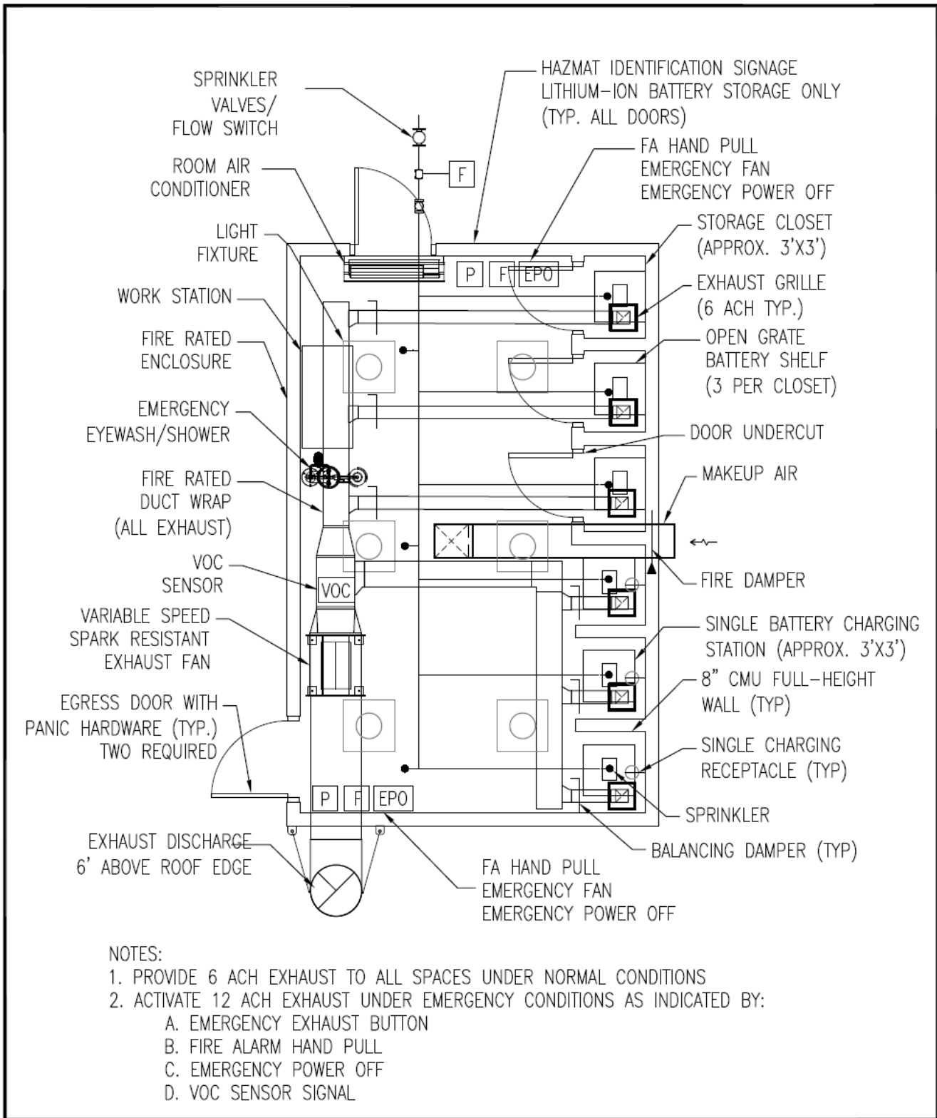
Figure 3-1 Concept Battery Storage and Charging Room Arrangement and Minimum Safety Features
