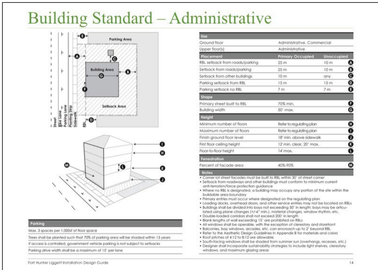
Figure A-7 Building Envelope Standards (BES) Graphic
