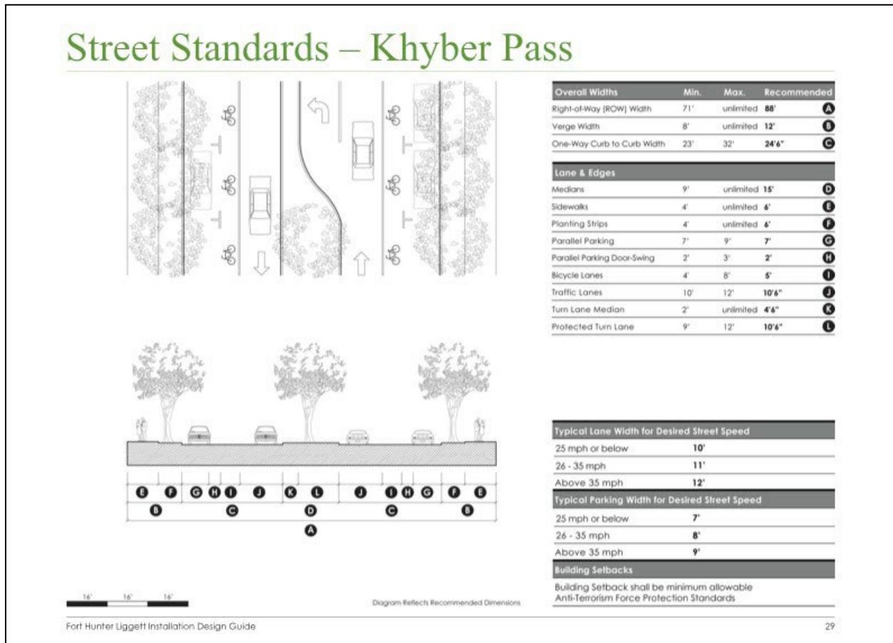
Figure A-8 Street Envelope Standards (SES) Graphic
