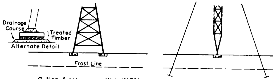
d. Non-frost-susceptible (NFS) foundation with shallow footings.
