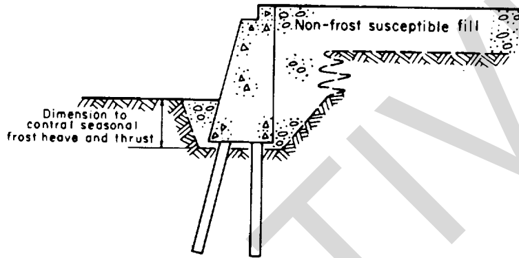
b. Pile-supported wall
