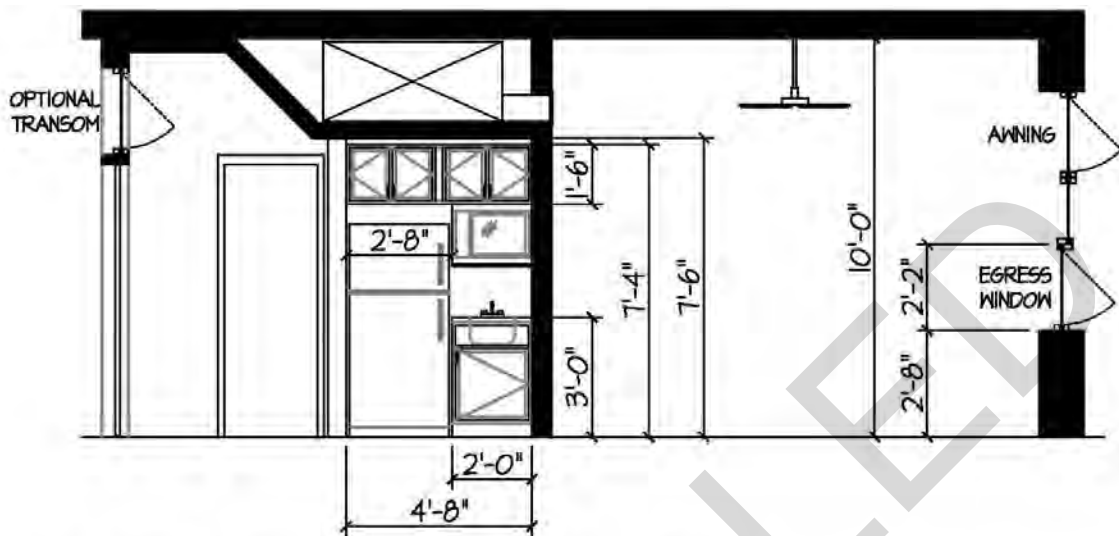
A SECTION THRU 2+ 0 ROOM NOT TO SCALE
