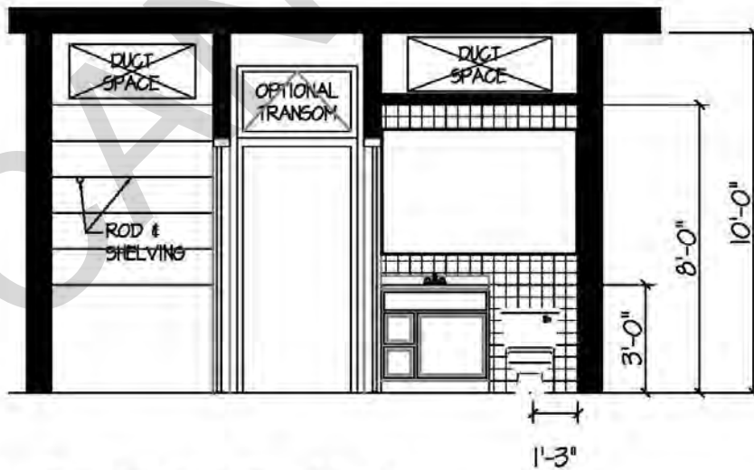
B SECTION @ ENTRY NOT TO SCALE
