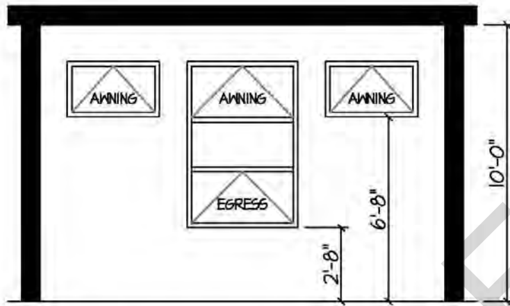
Figure B-14 – Section C of 2+0 Room Examples
