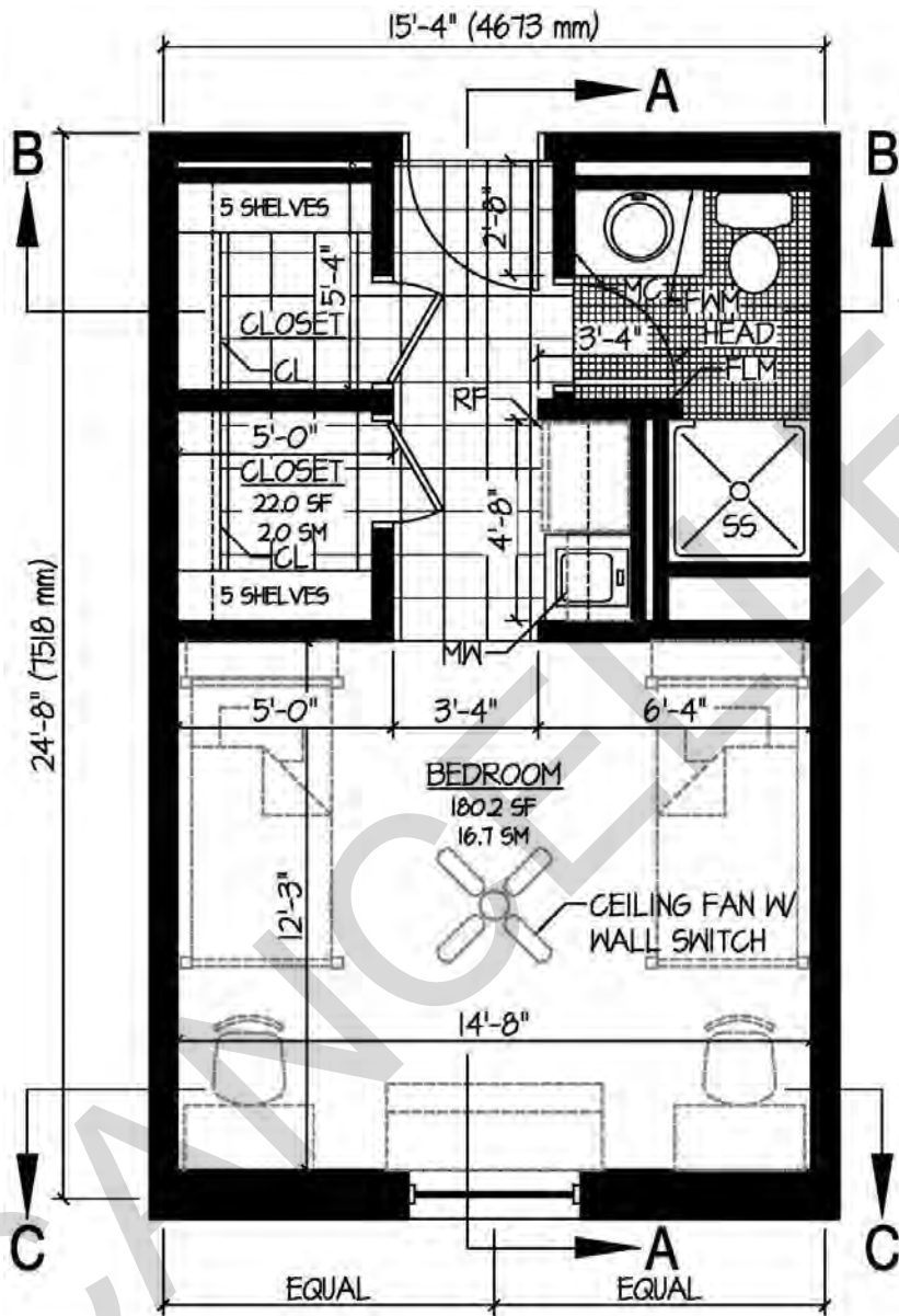
Figure B-5 – The Marine Corps 2+0 Room (Interior Access)
