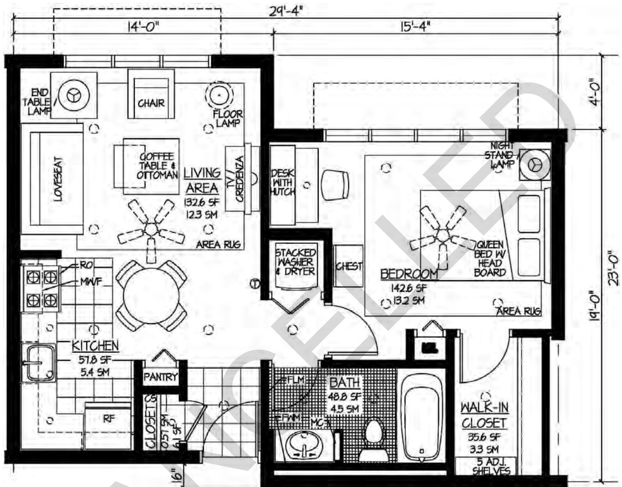
Figure B-7 – Marine Corps Officers Room Plan
