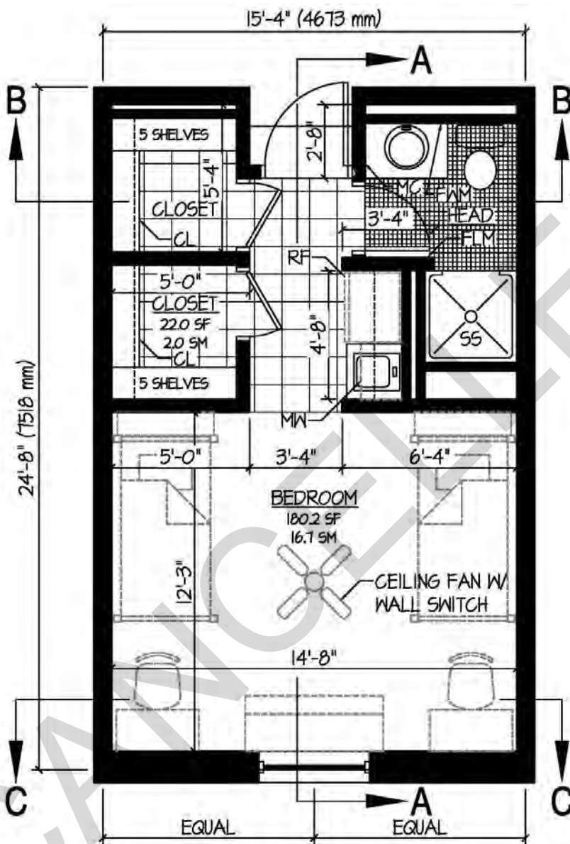
Figure B-6 – The Marine Corps 2+0 Room (Exterior Access)
