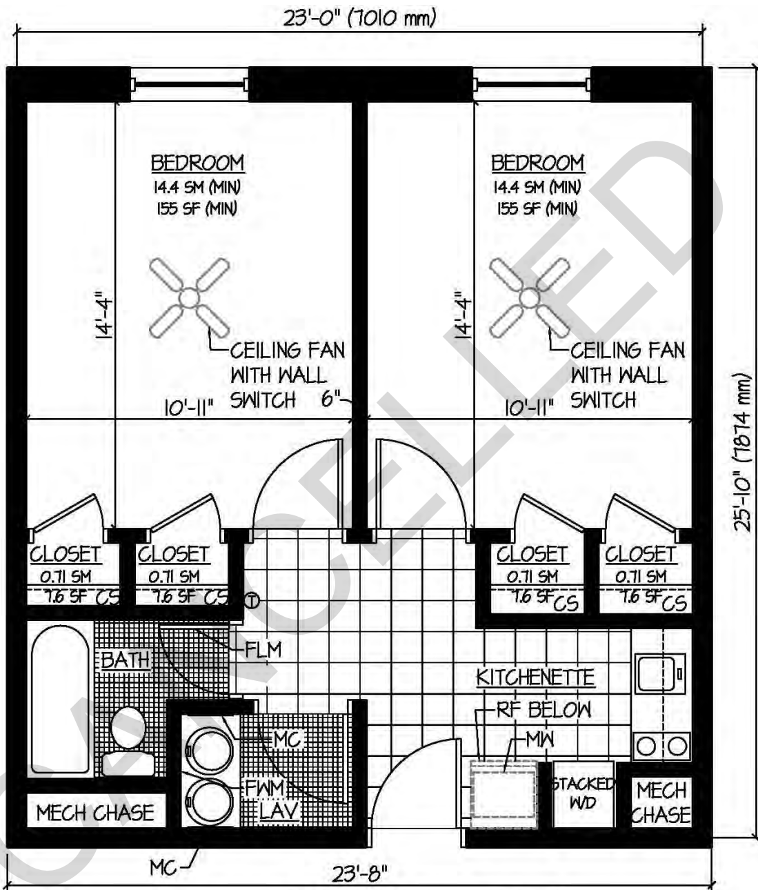
Figure B-2 – The 1+1E Square Apartment
