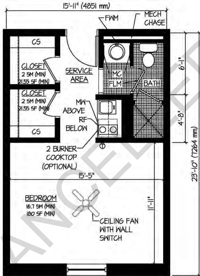
Figure B-4 – The Navy 2+0 Room
