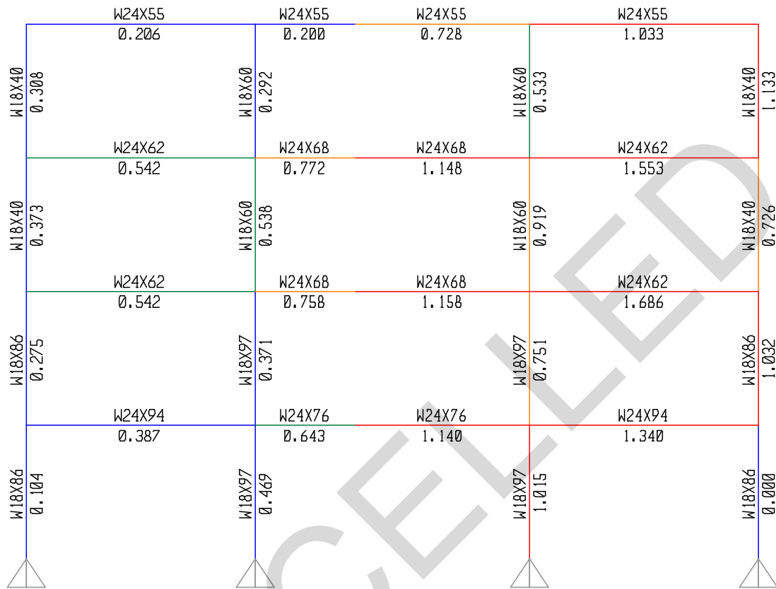
Figure E-10. Moment Ratios Due to Column 2 Removal with Redesign
