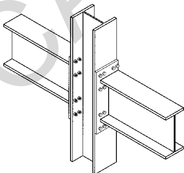
(c) End Plate (Unstiffened)
