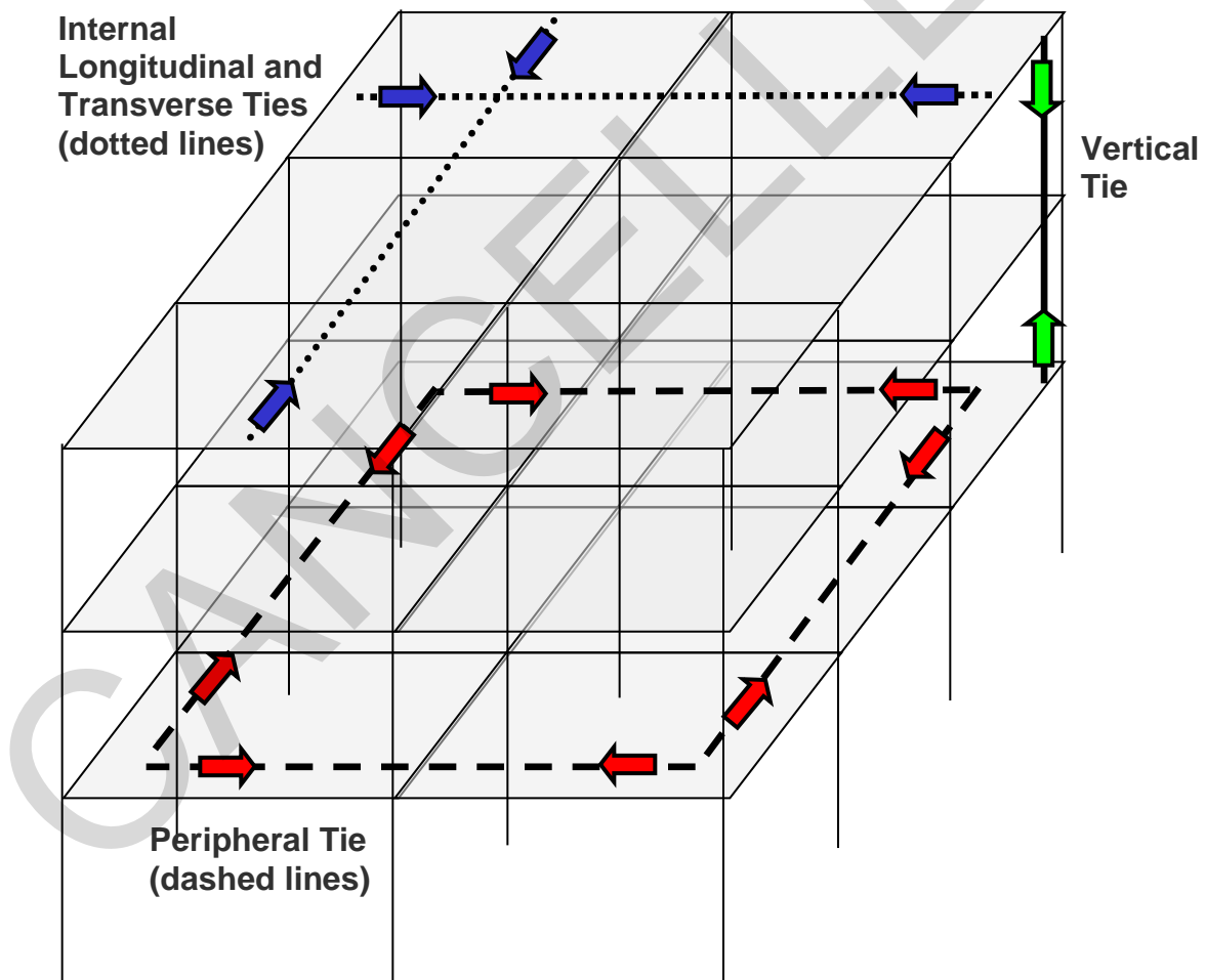
Figure 3-1. Tie Forces in a Frame Structure
