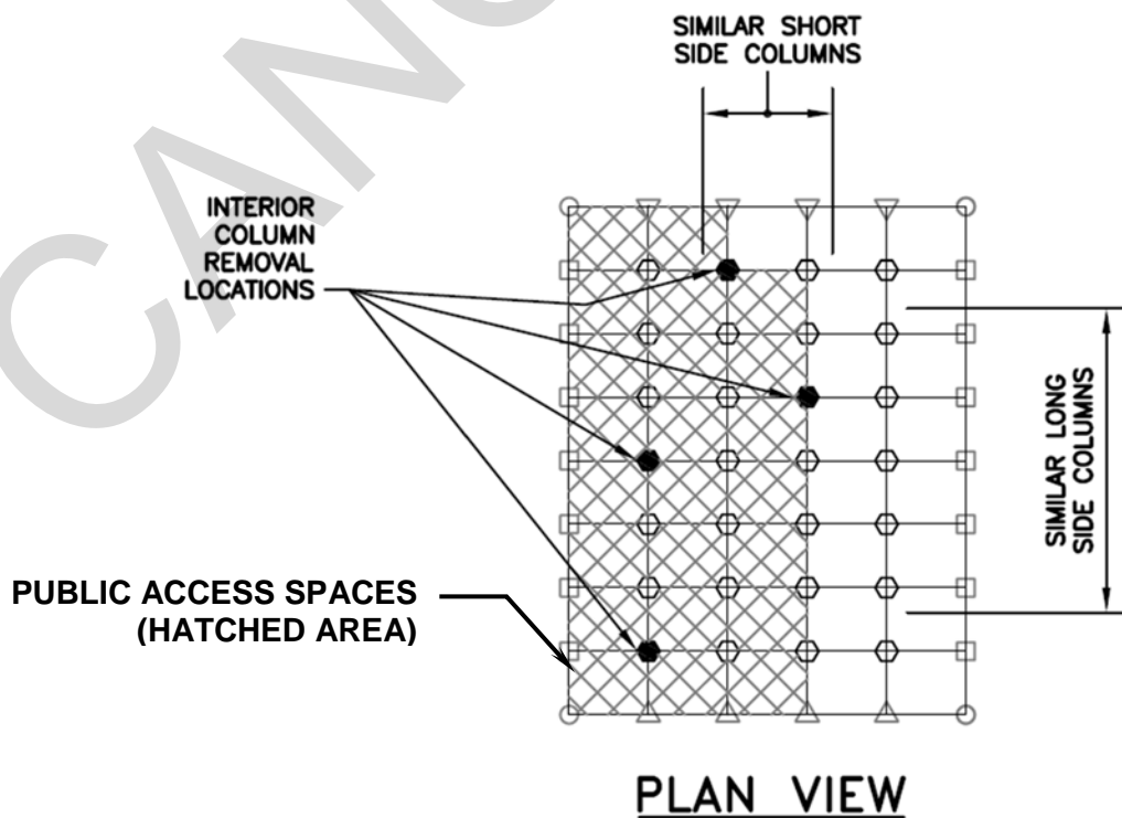
Figure 3-10. Location of Internal Column Removal for OC II Option 2, OC III and IV Structures
