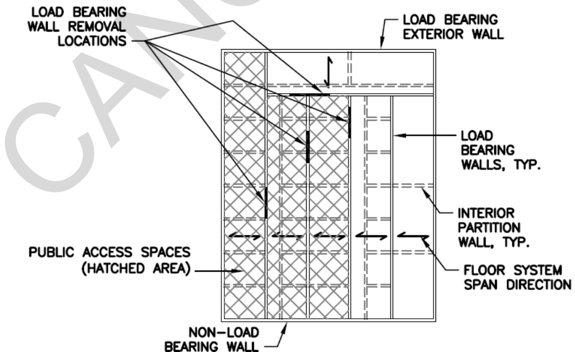
Figure 3-12. Location of Internal Load-Bearing Wall Removal for OC III and OC IV Structures
