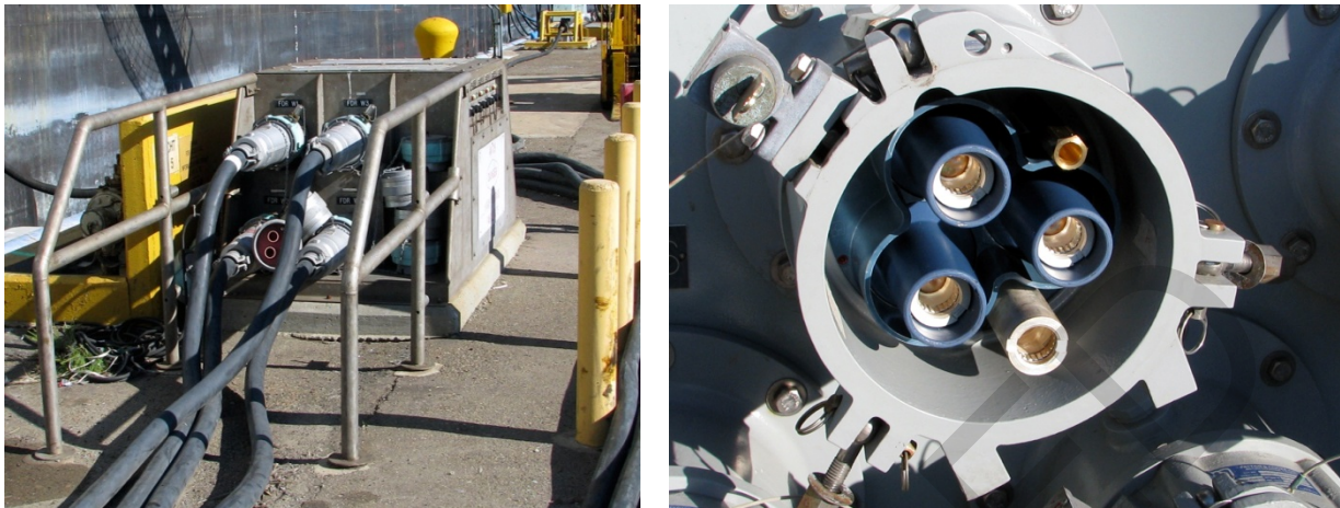
Figure 12-9. 4.16 kV Pier Electrical Outlet Assembly and Outlets – Newer Designs
