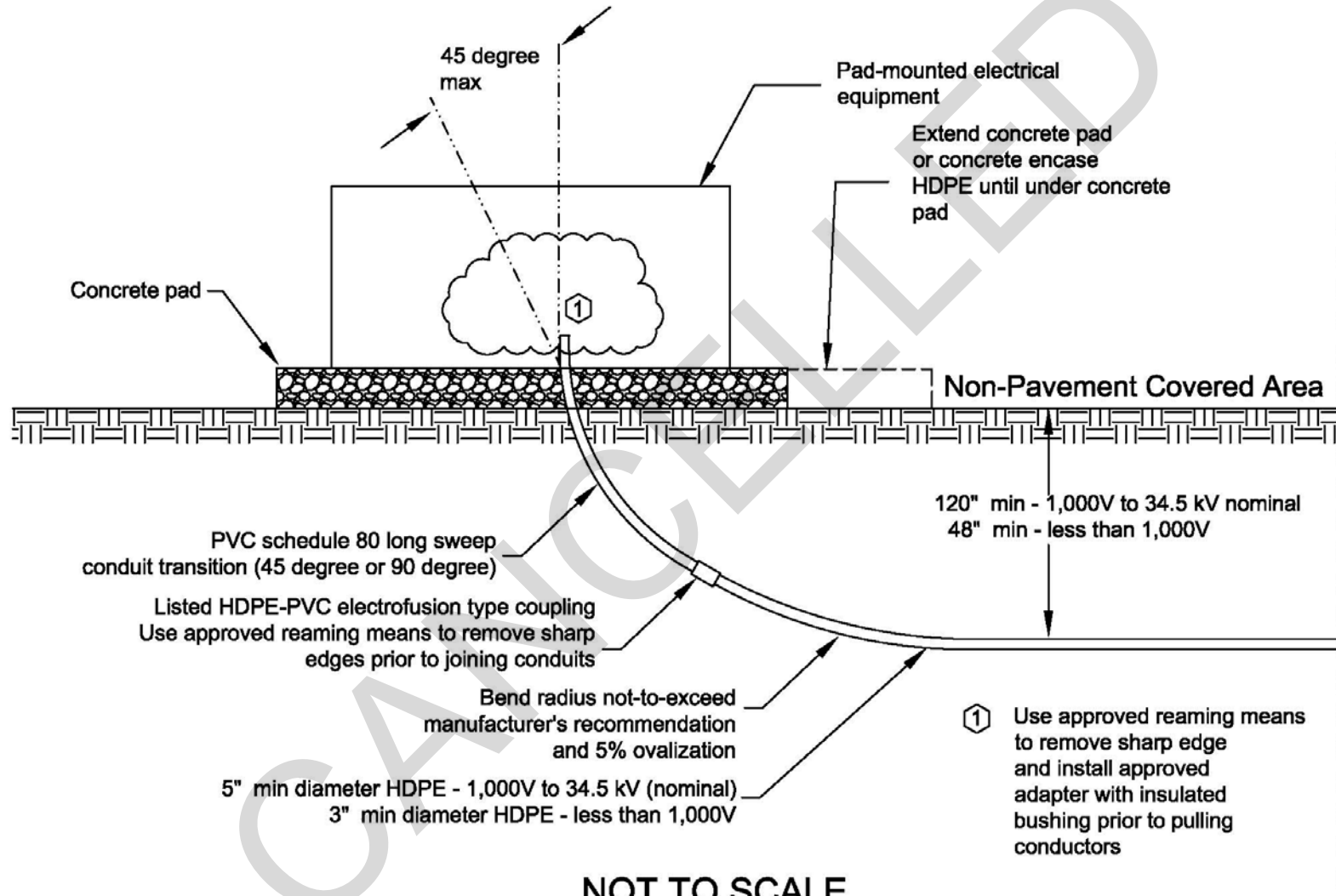
Figure B-4 Non-Pavement Covered Area to Electrical Equipment Transition – Rigid Conduit (45°–90°)
