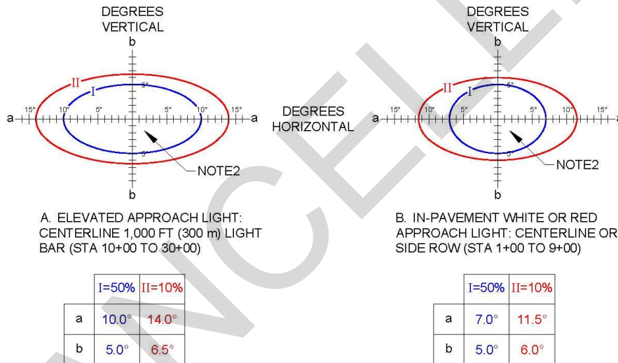
Figure 3-2 Approach Lighting Photometrics
