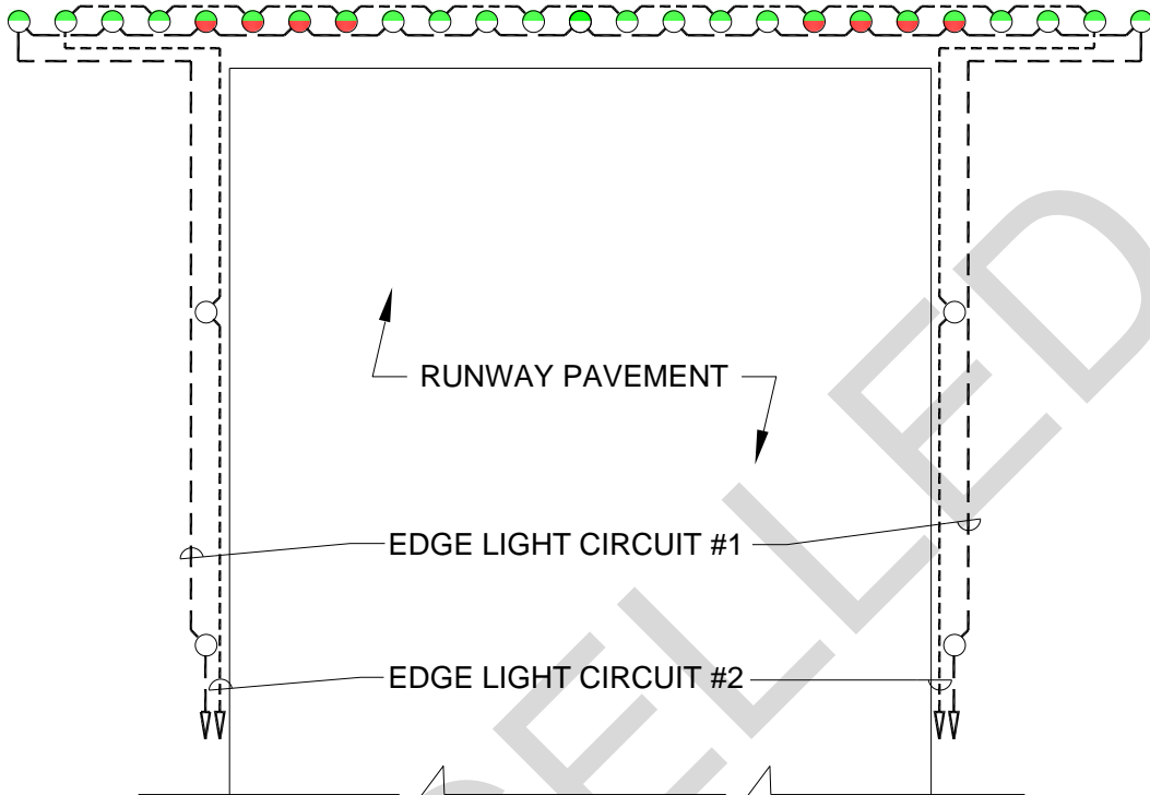
Figure 4-5C Threshold Light Circuiting for Army (interleaved)
