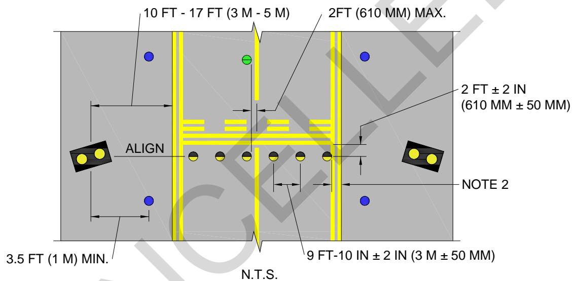
Figure 5-8 Runway Guard Light Configuration
