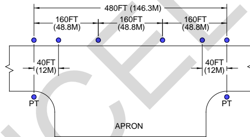
EXAMPLE C TYPICAL SINGLE STRAIGHT EDGES MORE THAN 400FT (120M) MAXIMUM SPACING = 200FT (60M)
