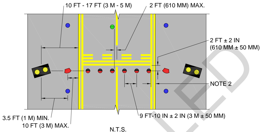
Figure 5-10 Runway Stop Bar Configuration
