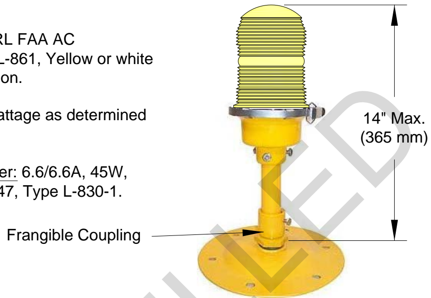
Figure 13-11 FAA L-861, Elevated, Omnidirectional
