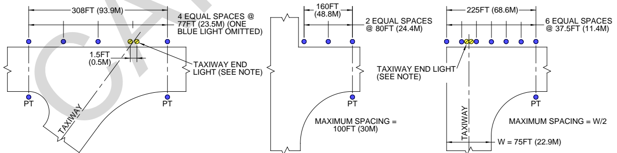
EXAMPLE D TYPICAL SINGLE STRAIGHT EDGES 400FT (120M) OR LESS MAXIMUM SPACING = 100FT (30M) (FOR SECTIONS 100FT (30M) OR LESS MAXIMUM SPACING = 50FT (15M)
