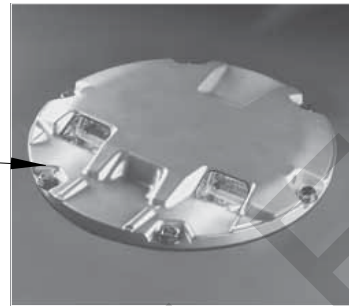
Figure 13-13 FAA-L-850D, In-pavement, Bidirectional
