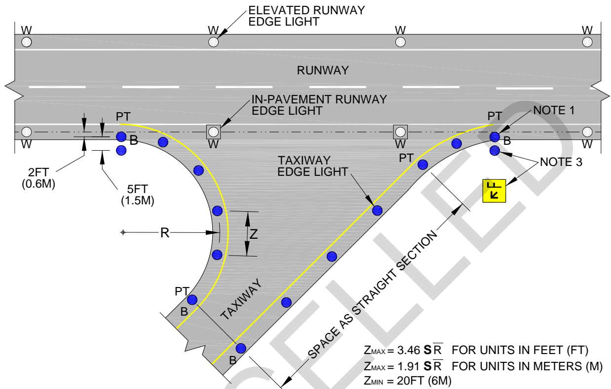
Figure 5-3 Taxiway Edge Lighting Configuration Entrance/Exit
