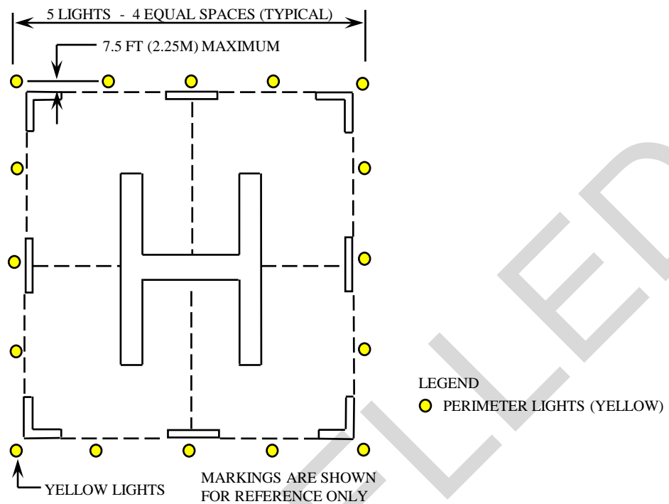
Figure 7-1 Helipad Perimeter Lights, Standard Configuration
