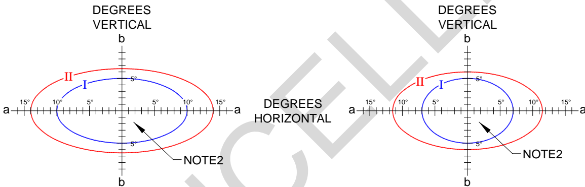
Figure 3-2 Approach Lighting Photometrics
