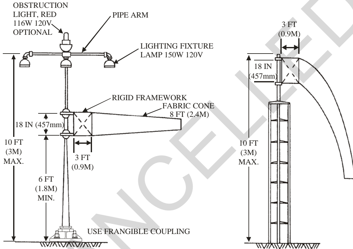
Figure 13-25 FAA L-806, Windcone, 8 Foot (2.4 Meter)
