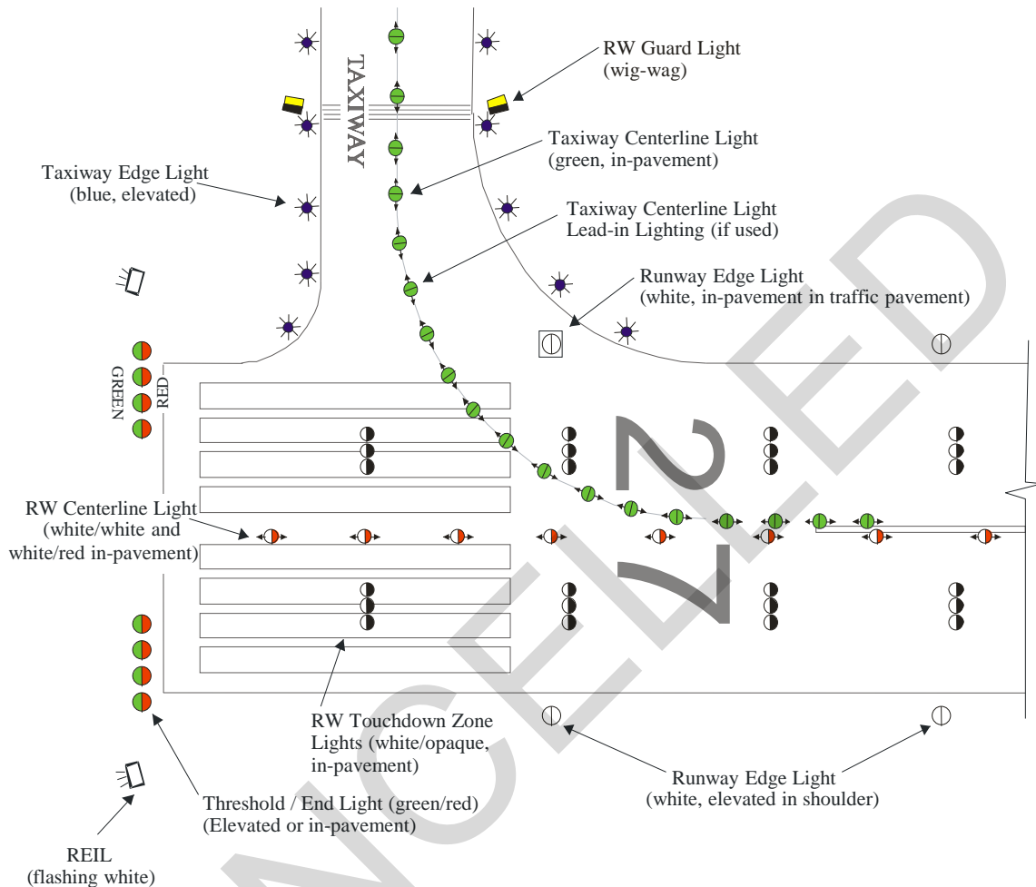
Figure 15-1 Typical AGL Layout
