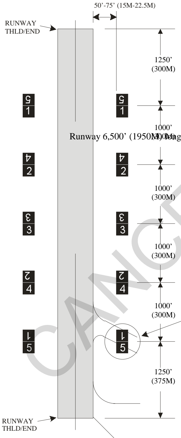
Figure 9-9 RDR Sign Layout Configuration
