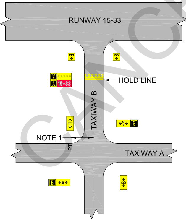
TYPICAL SIGNAGE LAYOUT
