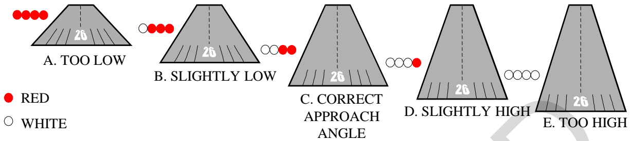
Figure 3-11 PAPI Configuration
