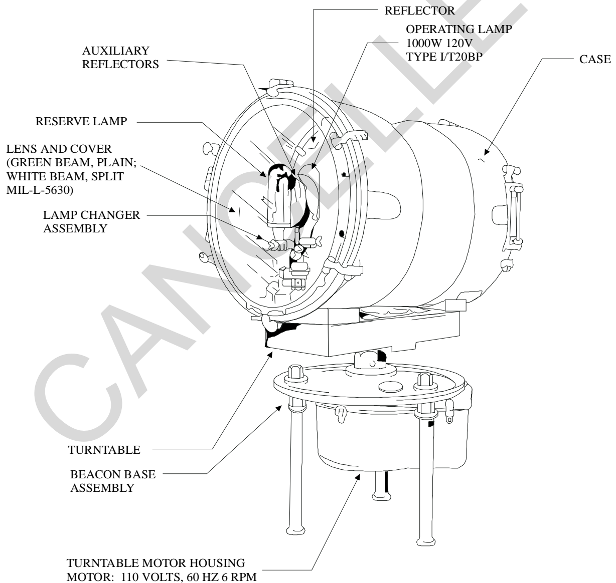
Figure 13-24 MIL-L-7158, Airfield Beacon, Rotating
