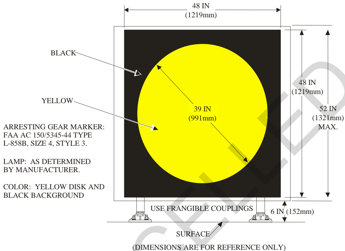
Figure 13-18 FAA L-858B, Sign, Elevated, AGM
