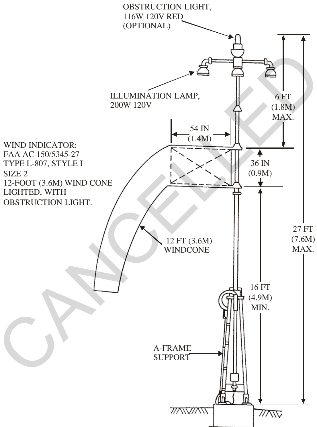
Figure 13-26 FAA L-807, Windcone, 12 Foot (3.6 Meter)
