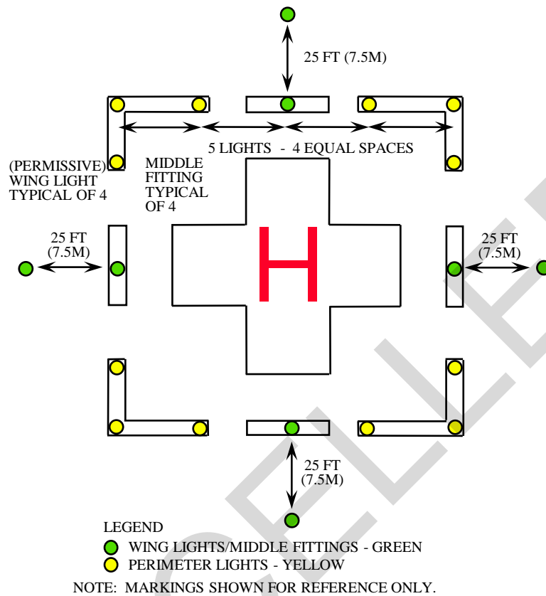
Figure 7-2 Helipad Perimeter Lights, Hospital Configuration
