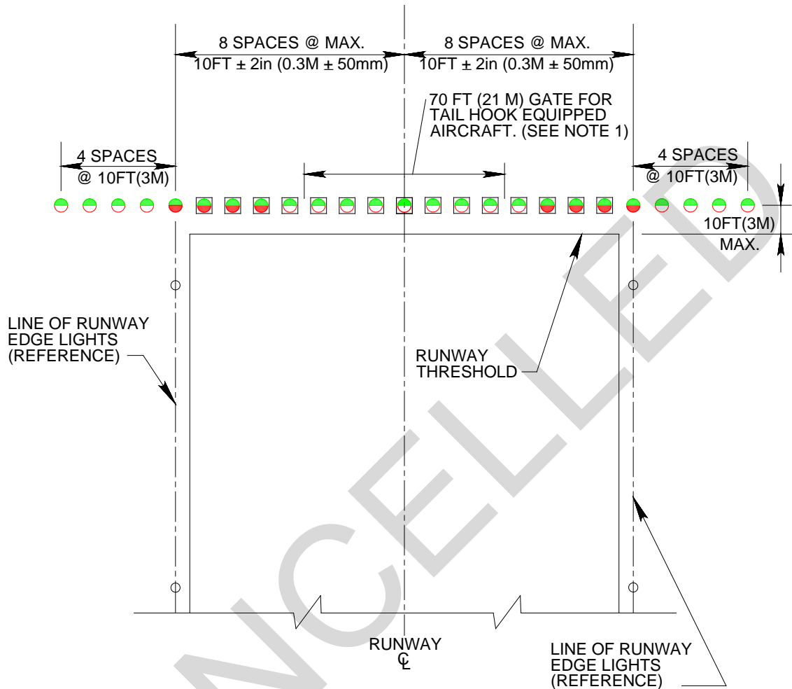
Figure 4-4B Threshold Light Configuration for Army
