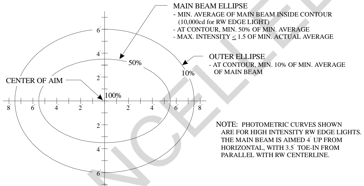
Figure 15-7 Photometric Isocandela Curves
