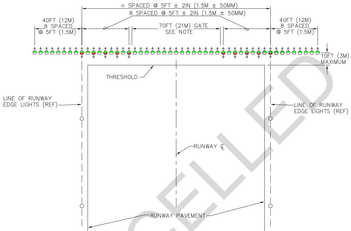
Figure 4-4A Threshold Light Configuration for Air Force
