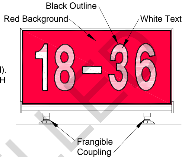
Figure 13-22 FAA L-858(L), Sign, Taxiway, Mandatory Note: These signs represent the bulk of existing signs and comply with previous edition of FAA AC 150/5345-44. These signs do not require replacement until the end of their economic lives or with a major renovation to the airfield. See current edition of FAA AC for new sign message elements.
