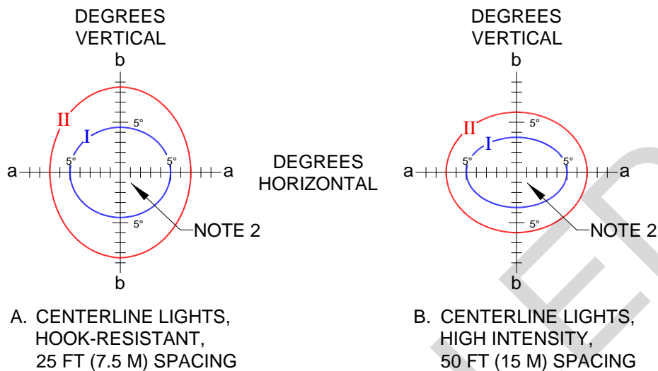
Figure 4-13 Runway Centerline Light Photometric Configuration
