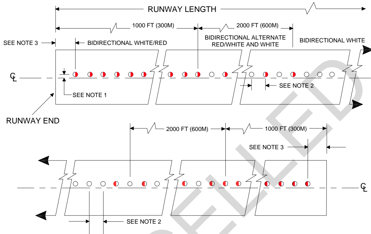
Figure 4-12 Runway Centerline Light Configuration
