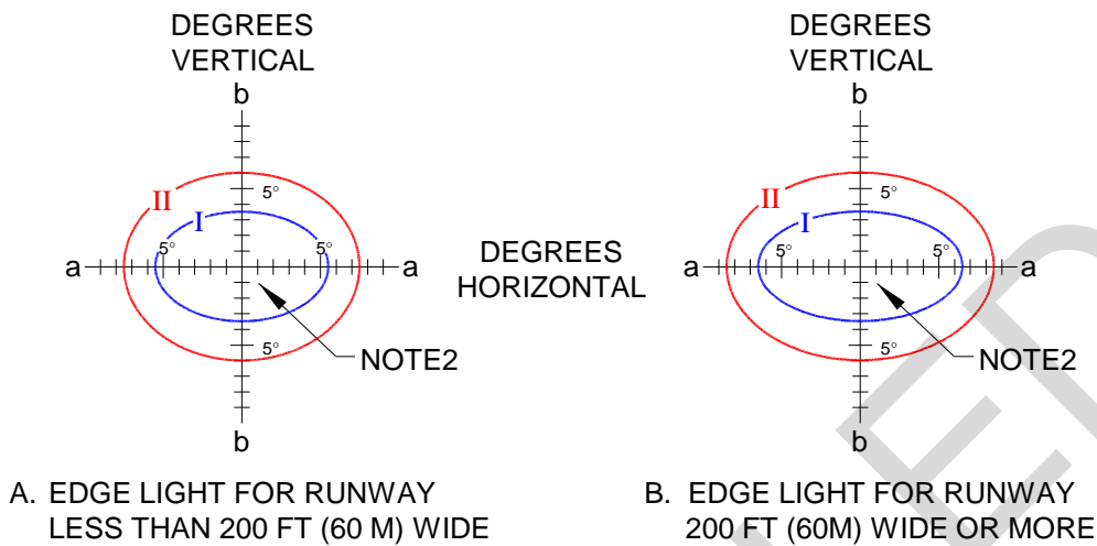
Figure 15-6 Runway Edge Light Photometric Requirements
