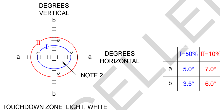
Figure 4-15 Touchdown Zone Light Photometric Requirements
