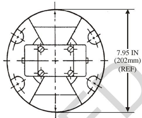
Figure 13-12 FAA L-852, (A, B, C, D), In-pavement, Bidirectional
