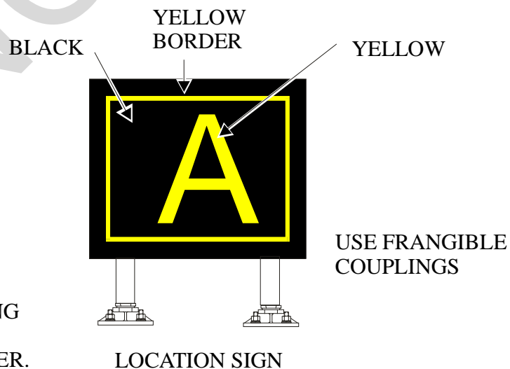
Figure 13-23 FAA L-858L, Sign, Taxiway, Location
