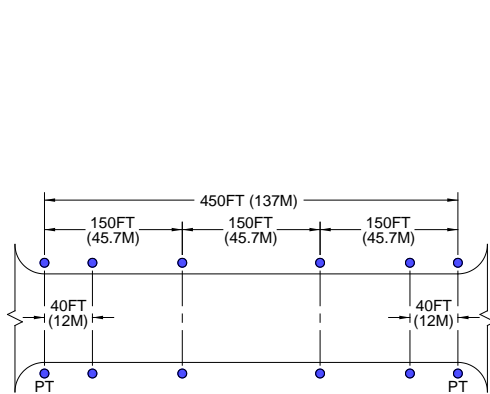
EXAMPLE A TYPICAL STRAIGHT SECTIONS MORE THAN 400FT (120M) MAXIMUM SPACING = 200FT (60M)
