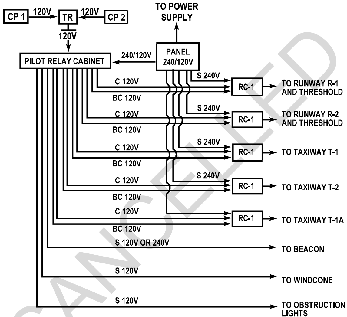
Figure 8-5 Block Diagram Typical System
