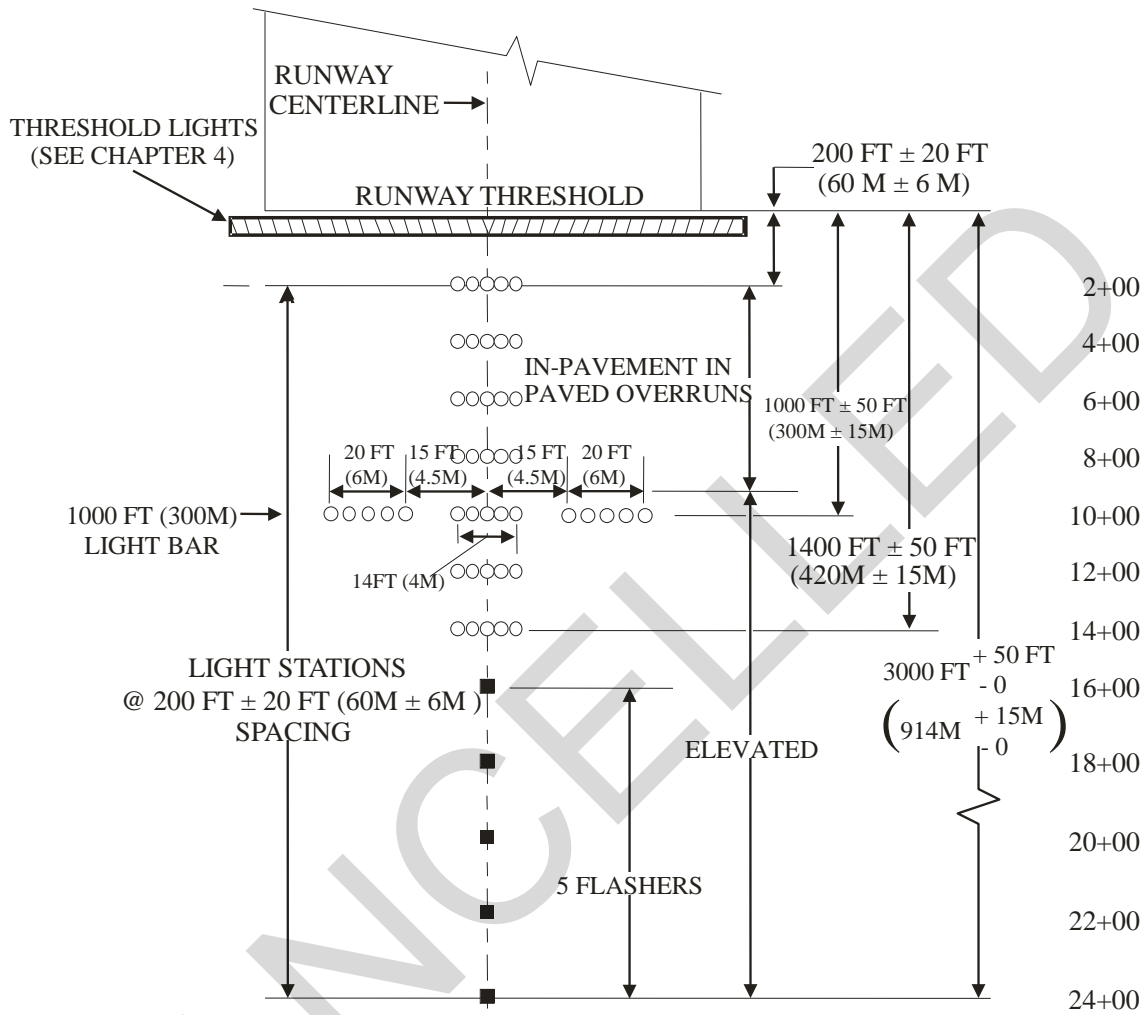
Figure 3-8 SSALR Configuration
