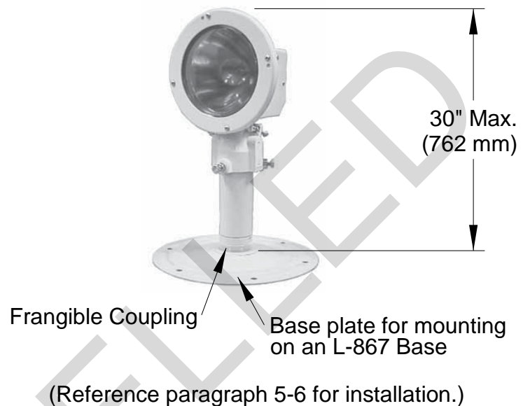
Figure 5-12 FAA L-862S, Elevated Stop Bar Light
