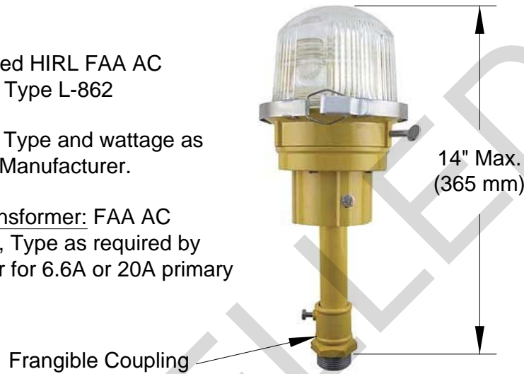
Figure 13-9 FAA L-862, Elevated, Bidirectional
