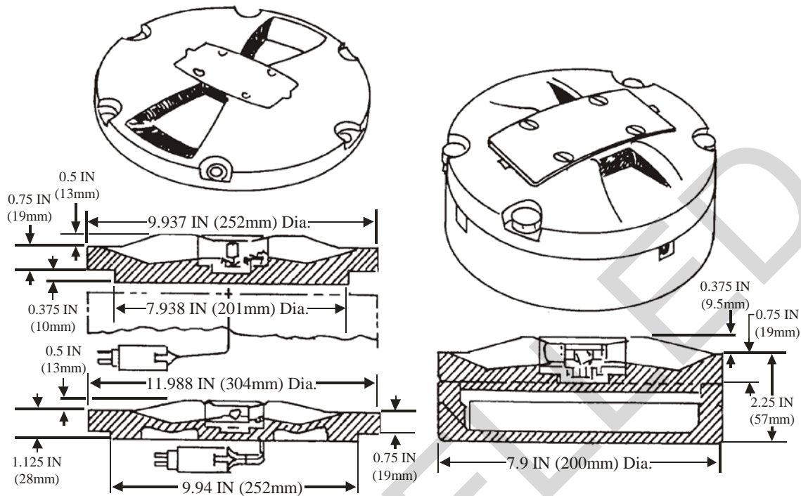
Figure 13-16 FAA L-852N, In-pavement, Bidirectional (Hook-resistant)
