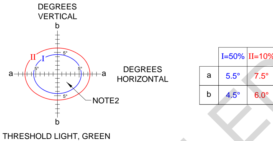
Figure 4-6 Threshold Light Photometric Requirements
