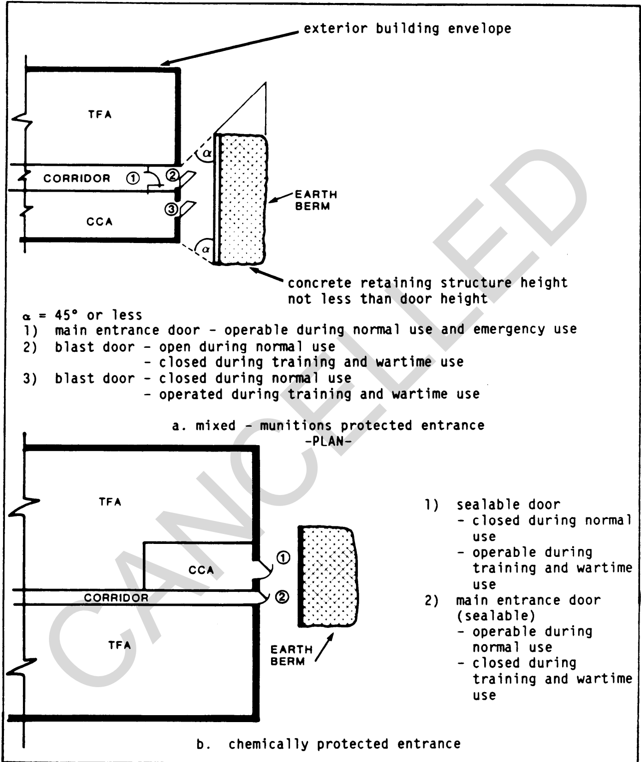
Figure 2 Entrance Arrangements
