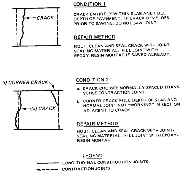
Figure 1. Approved methods for repair of uncontrolled cracks and spalls in rigid pavements.
