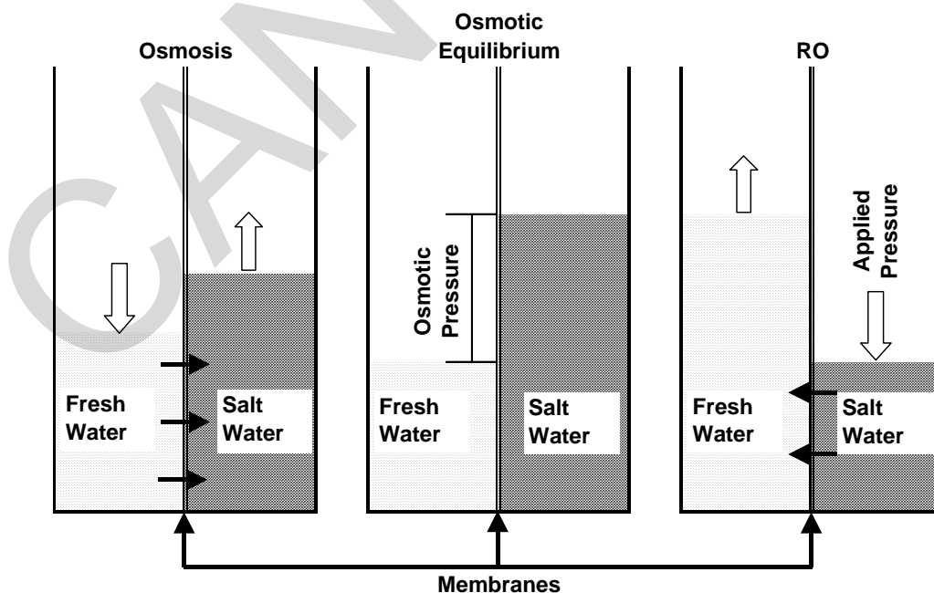
Figure 2-7. RO Schematic
