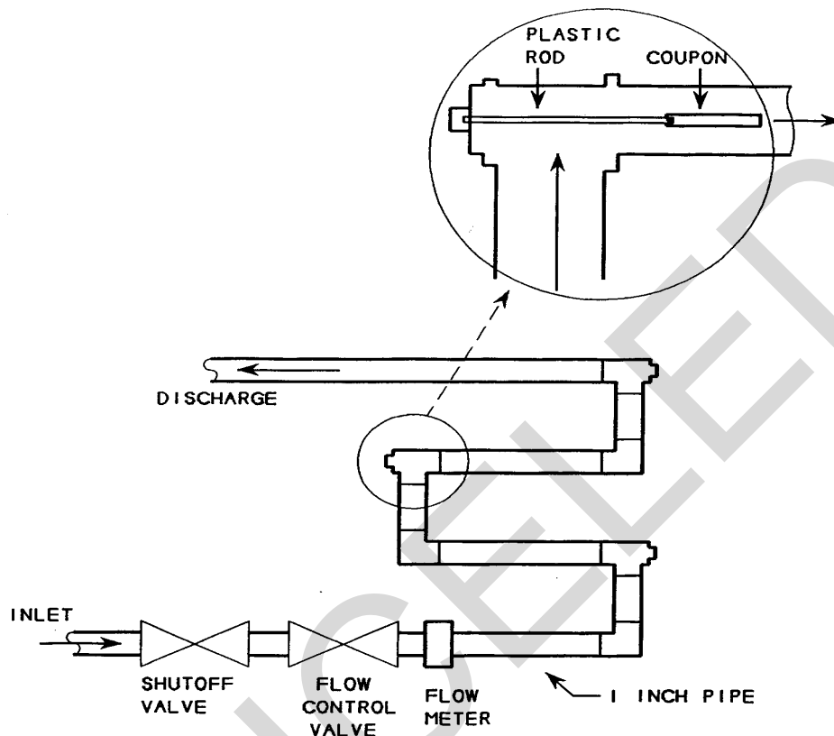
FIGURE C-1. Bypass Piping for Corrosion Testing Cooling Water and Condensate Systems
