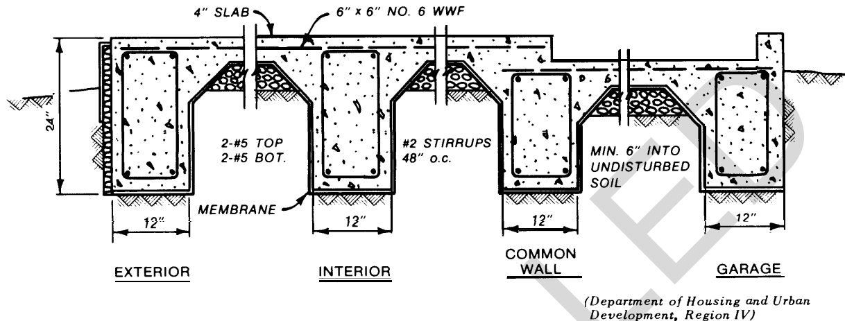
Figure 6-5. Typical conventional rebar slab in Little Rock, Arkansas, for single-family, single-story, minimally loaded frame residence with 11- to 12-foot wall spacing.
