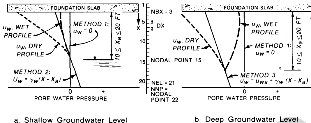
a. Shallow Groundwater Level
