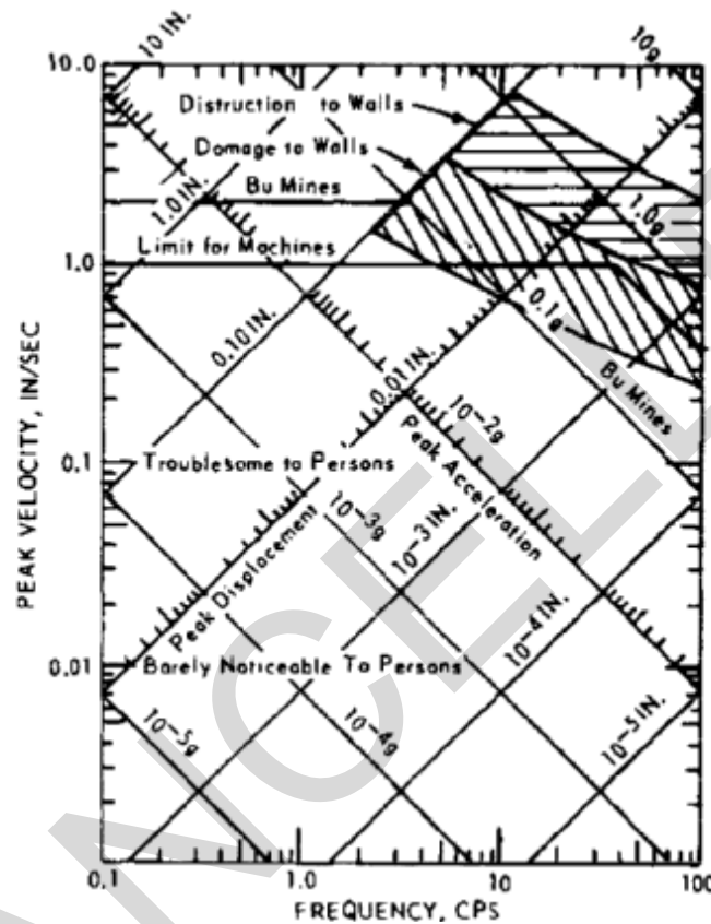
Figure 12-1 Response Spectra for Vibration Limits
