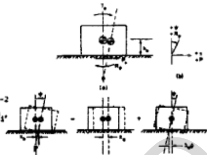
Figure 12-6 Coupled Rocking and Sliding Motion of Foundation
