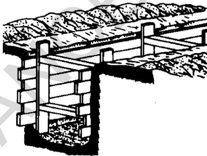
Figure 8-1.5 Telescopic Shoring
