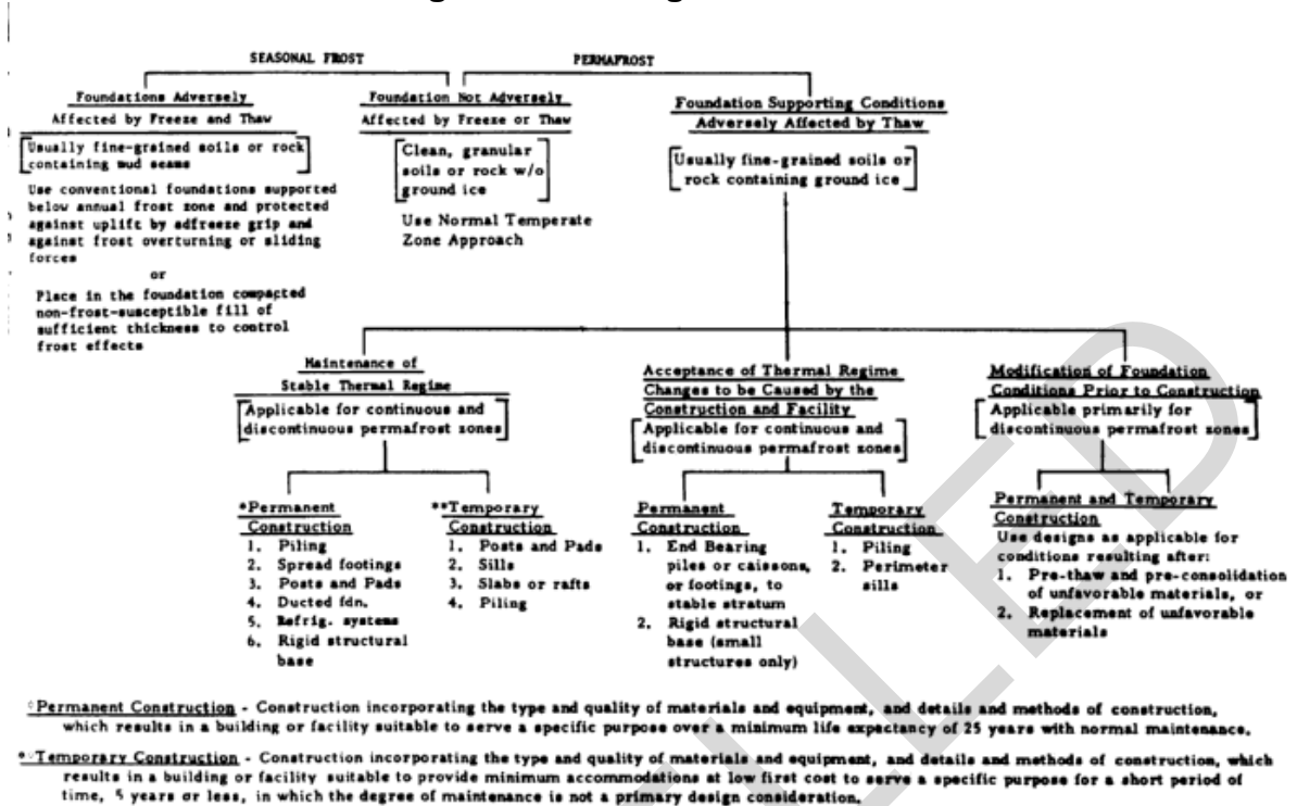
Figure 11-4 Design Alternatives
