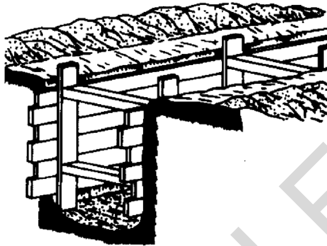
Figure 8-1.5 Telescopic Shoring
