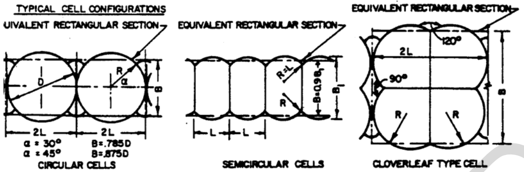
Figure 6-1 Design Criteria for Cellular Cofferdams
