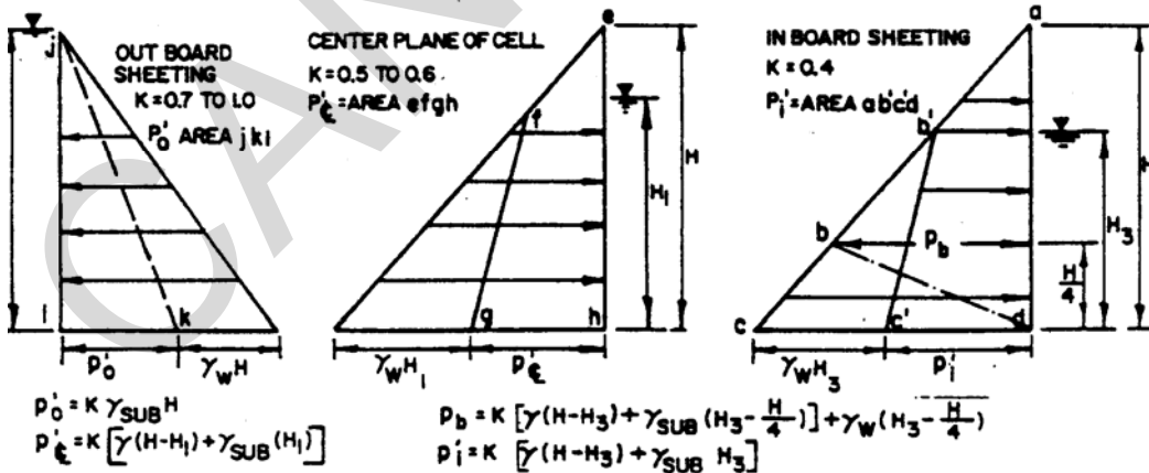
HORIZONTAL STRESS DIAGRAMS IN CELL FILL
