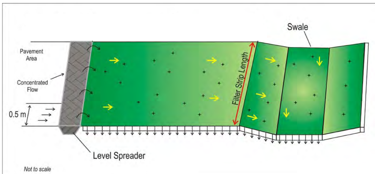
Figure 8-4. Filter Strip
