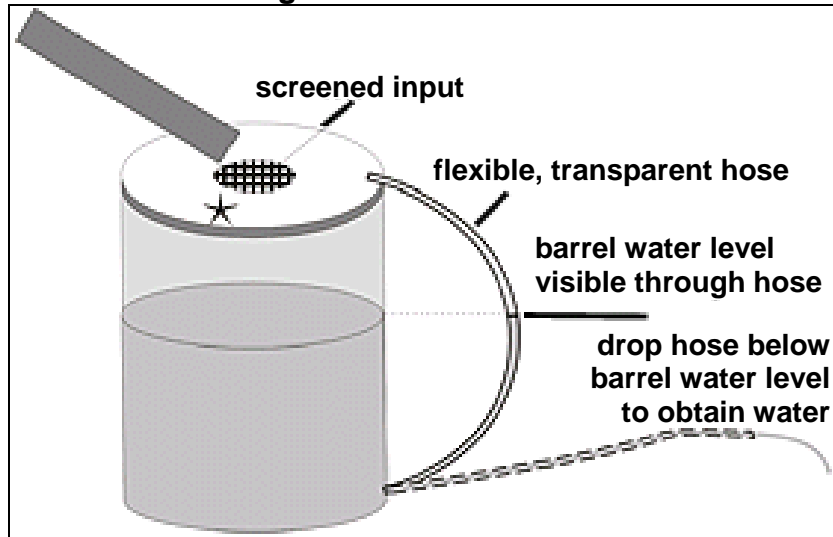
Figure 8-9. Rain Barrel
