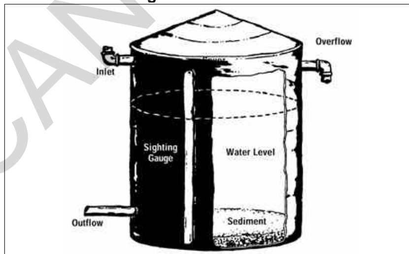
Figure 8-10. Cistern
