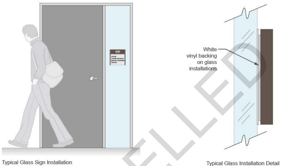
Figure 4-8 Typical Sign Installations on Glass.
