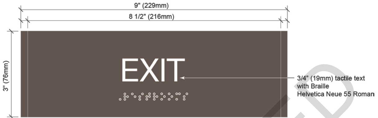
Figure 4-10 Tactile Exit Signs. /1/
