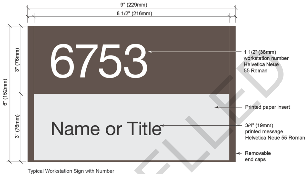
Figure 4-3 Workstation Identification Signs. /1/
