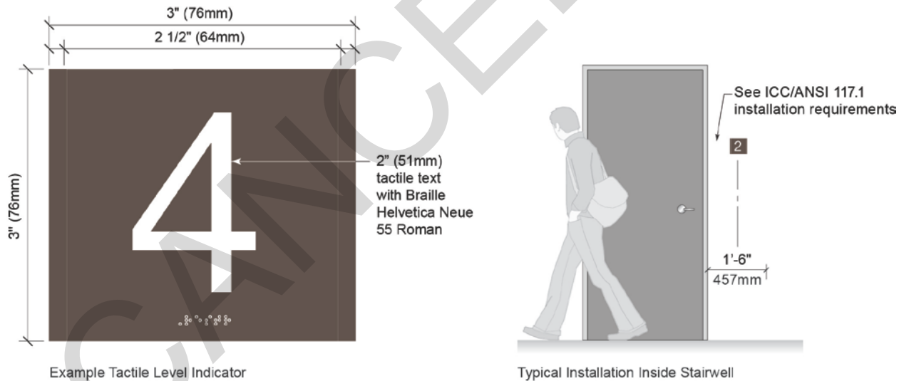
Figure 4-11 Tactile Stairway Level Indicators. /1/
