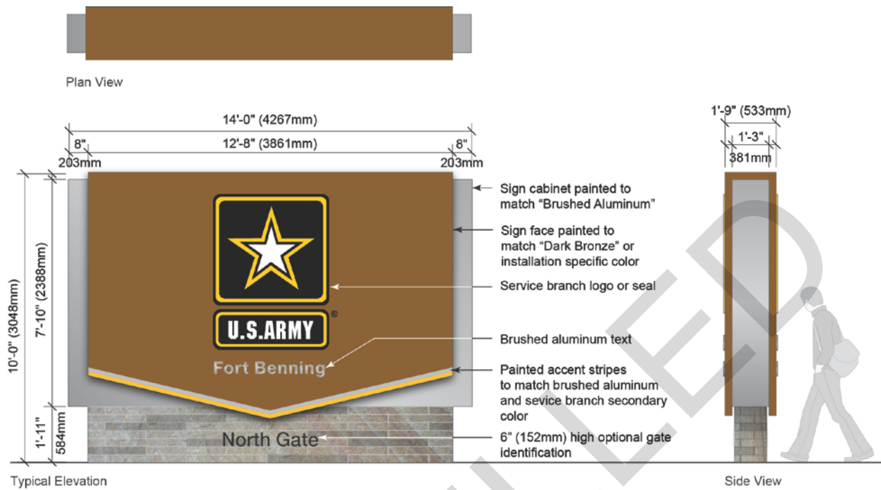
Figure 3-3 Primary Installation and Gate Identification Signs.
