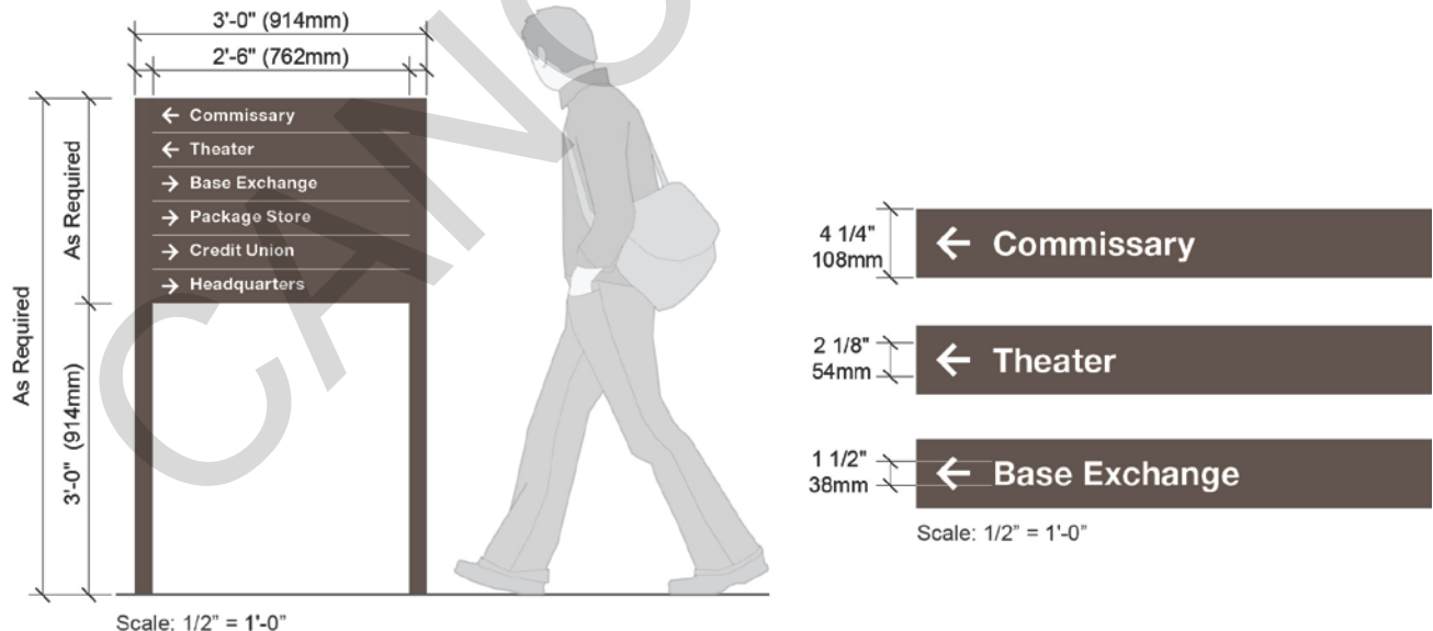
Figure 3-18 Pedestrian Directional Signs.
