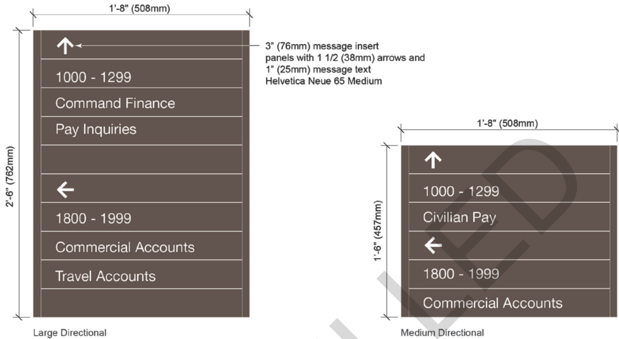
Figure 4-15 Interior Wall-Mounted Directional Signs.
