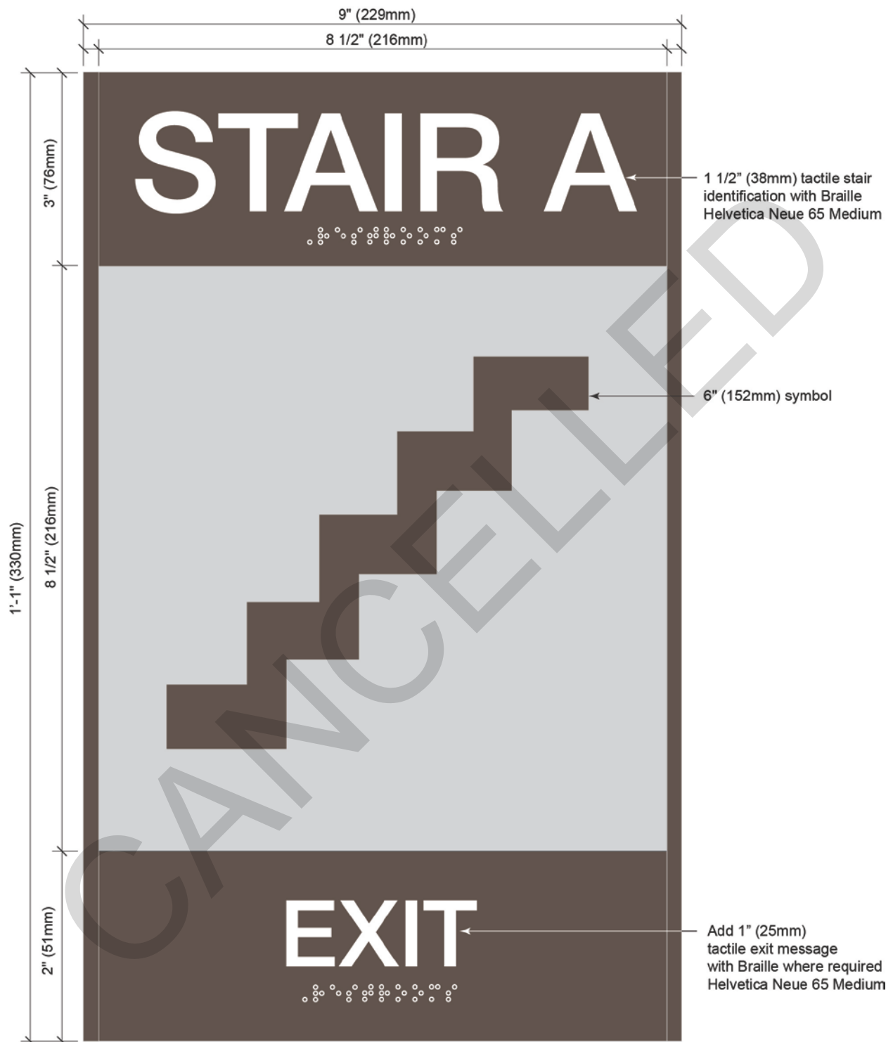
Figure 4-6 Stair Identification Signs.
