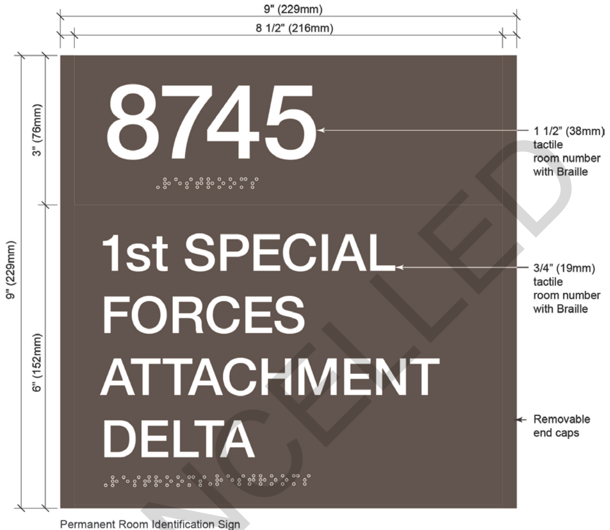
Figure 4-2 Permanent Room Identification Signs.
