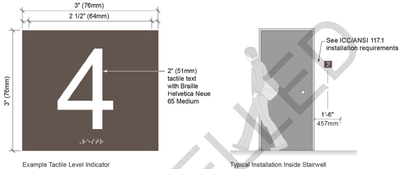
Figure 4-11 Tactile Stairway Level Indicators.
