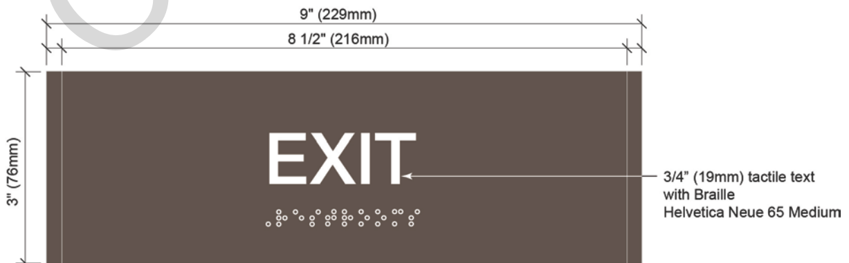
Figure 4-10 Tactile Exit Signs.
