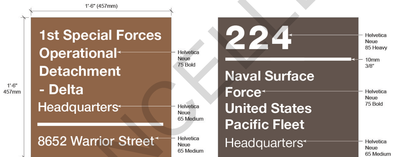
Figure 3-12 Building Entrance Signs.
