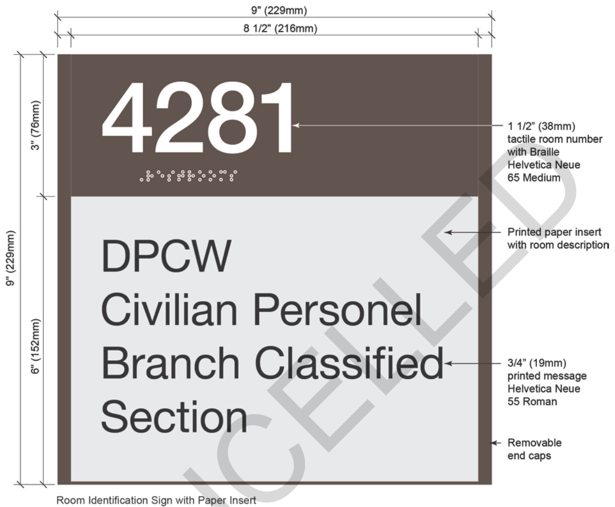
Figure 4-1 Room Identification Signs.
