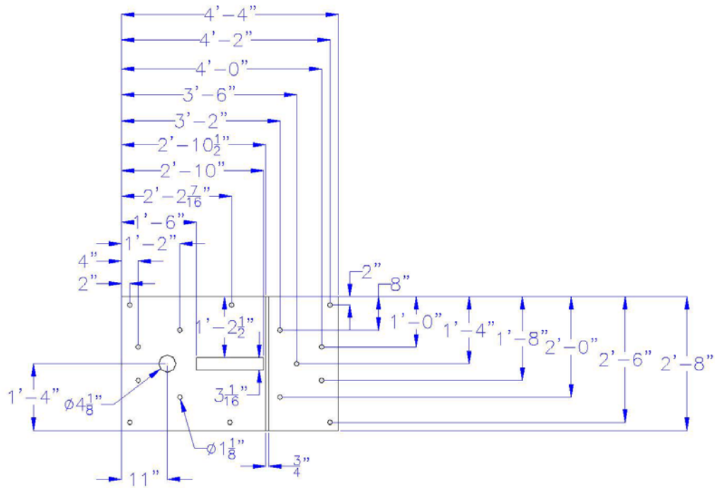
Figure A1.3. Expedient Anchor Plate Plan View with Dimensions for Bolt and Steel Anchor Post Holes (Pour Holes Not Shown)
