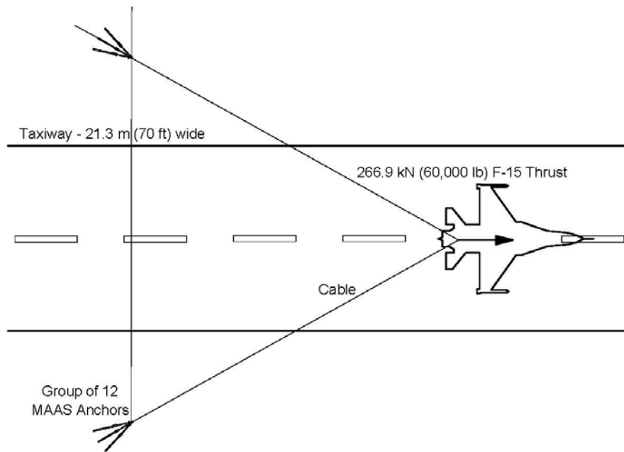
Figure 1. Expedient Trim Pad Schematic
