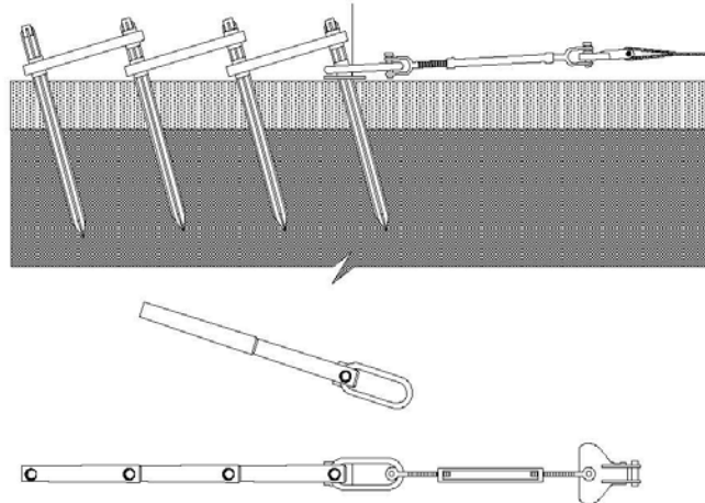
Figure 6. Reference Line for Monitoring Anchors
