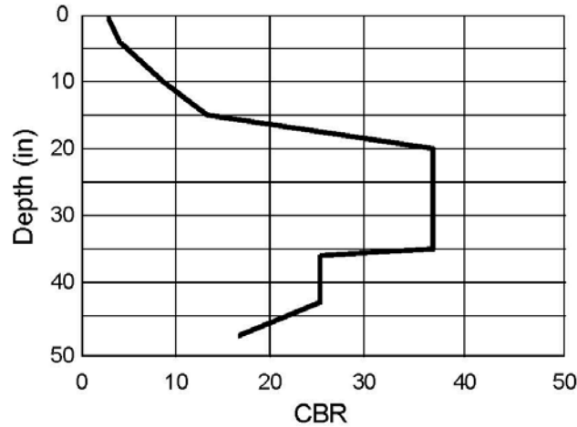
Figure 3. CBR Profile for Test Locations
