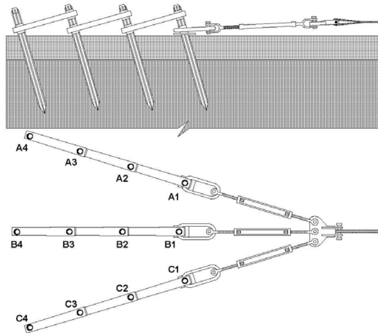
Figure 2. 12-Stake Anchor Group Schematic
