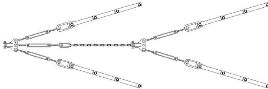
Figure 4. 16-Stake Anchor Group Schematic
