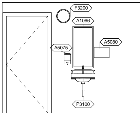
NMUR1 - SOUTH ELEVATION
