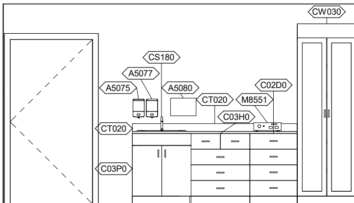
DNTS1 - SOUTH ELEVATION
