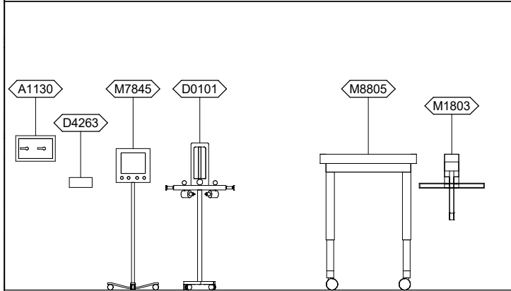
DNTS1 - NORTH ELEVATION
