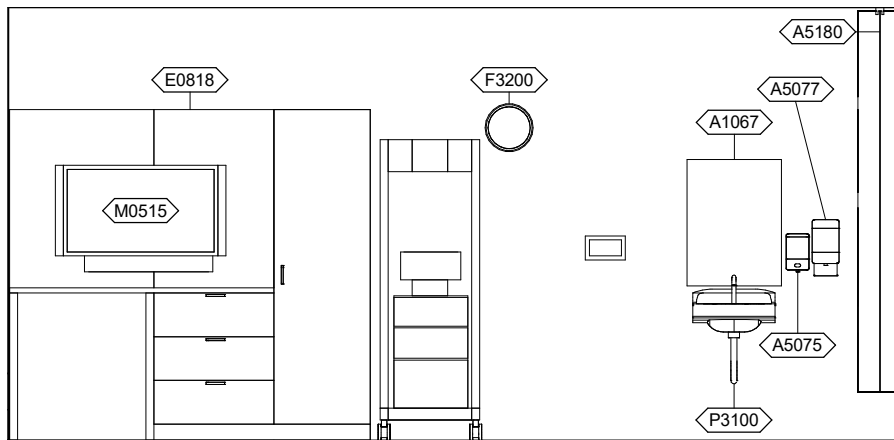
NYIR1 - EAST ELEVATION
