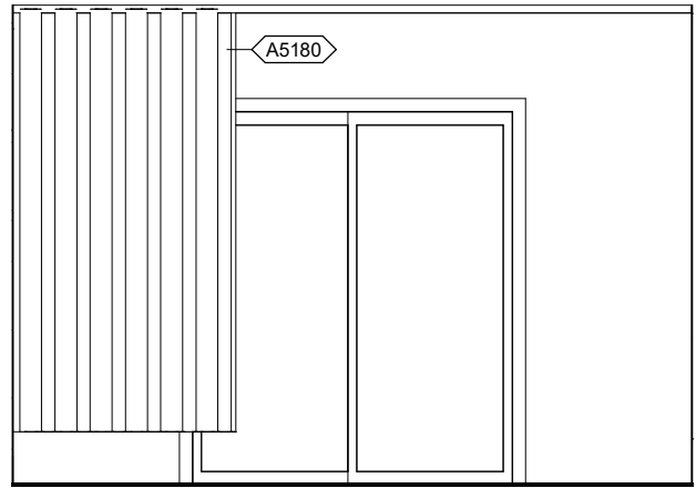
NYIR1 - SOUTH ELEVATION
