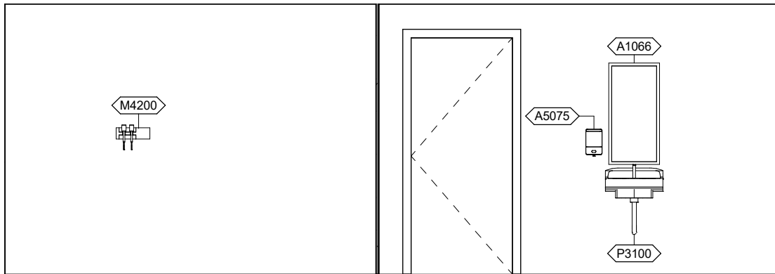
EYEL1 - SOUTH ELEVATION
