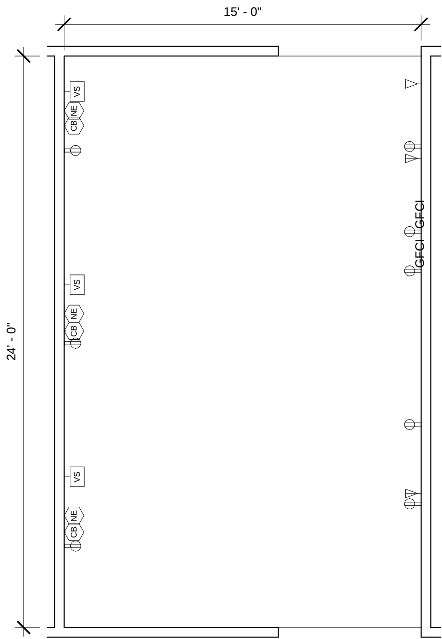
LBVP2 - FLOOR PLAN
