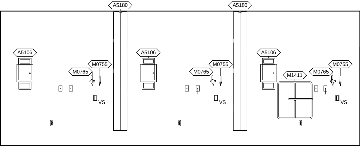
LBVP2 - WEST ELEVATION
