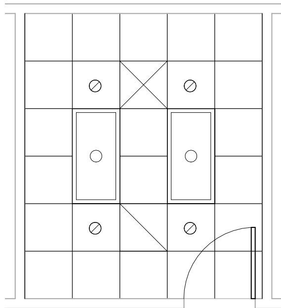
EYVF1 - CEILING PLAN
