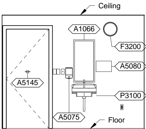
EYVF1 - PLAN SOUTH
