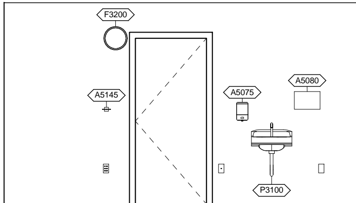
DN5C5 - SOUTH ELEVATION
