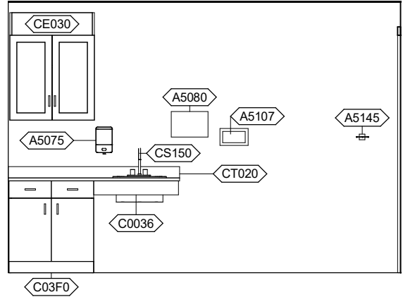
XDUS1 - EAST ELEVATION
