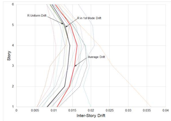
Drift Results for 6 Story Moment Frame
