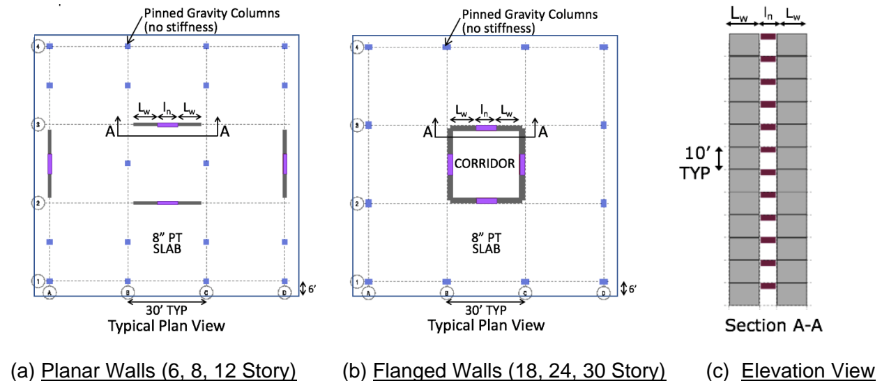
Figure 3.9-1 Archetype floor plans and typical wall elevation view
