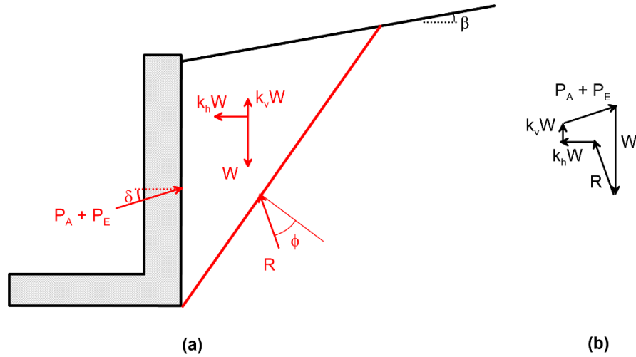
Figure 1 (a) Retaining wall with horizontal and vertical pseudo-accelerations applied to backfill wedge; (b) force polygon showing the effect of inertial forces from pseudo-acceleration on the wall-soil interaction force.
