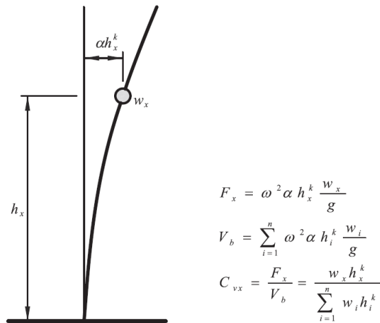
FIGURE C12.8-3 Basis of Eq. (12.8-12)
