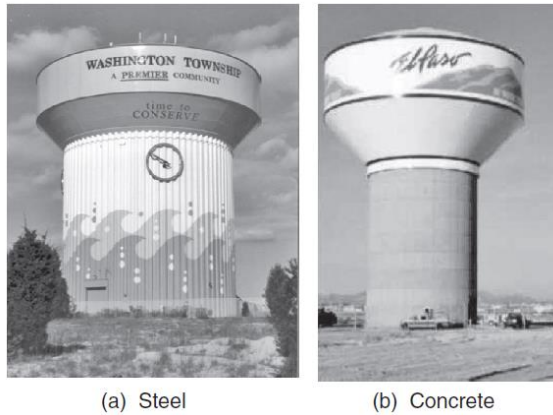
FIGURE C15.7-3 Large-diameter, single-pedestal tank
