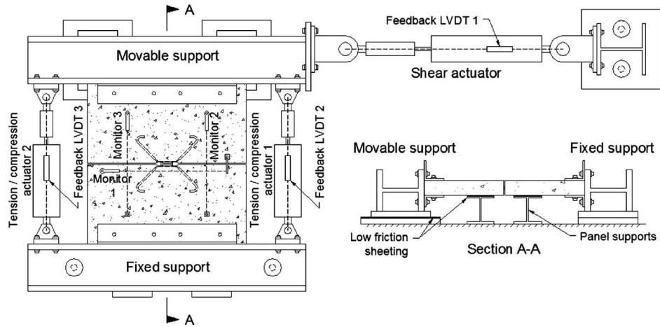
FIGURE C14.2-5 Possible Test Setup
