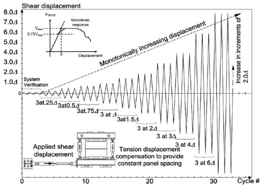
FIGURE C14.2-6 Shear Loading Protocol
