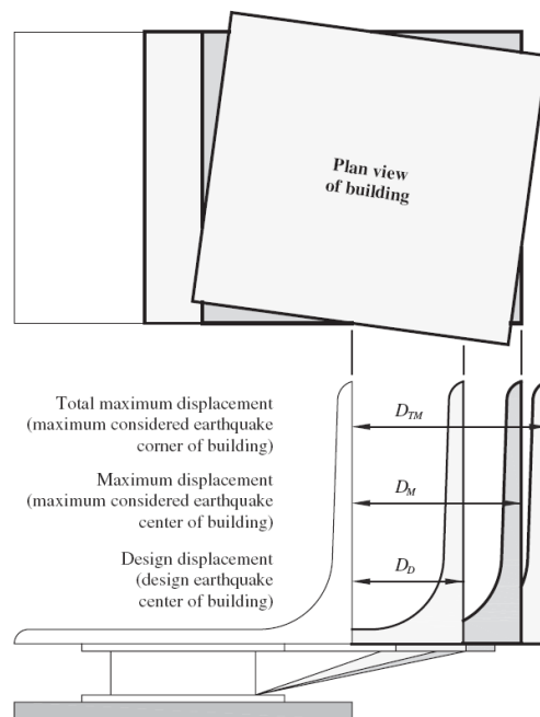
FIGURE C17.5-1 Displacement Terminology
