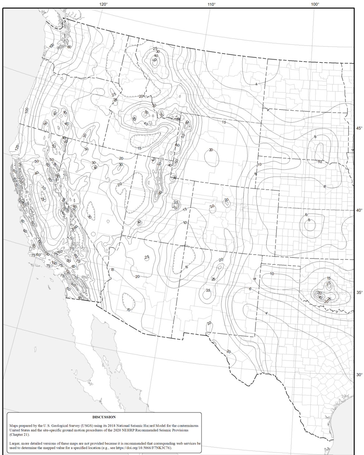
Figure 22-9 PGA_M for the Default Site Class, for the conterminous United States
