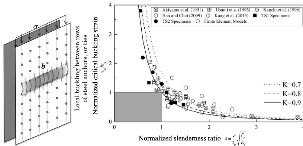
Figure C14.3.5- 6 Local buckling of steel plates, and plot of normalized critical buckling strain vs. slenderness ratio (Zhang et al. 2014, 2019)
