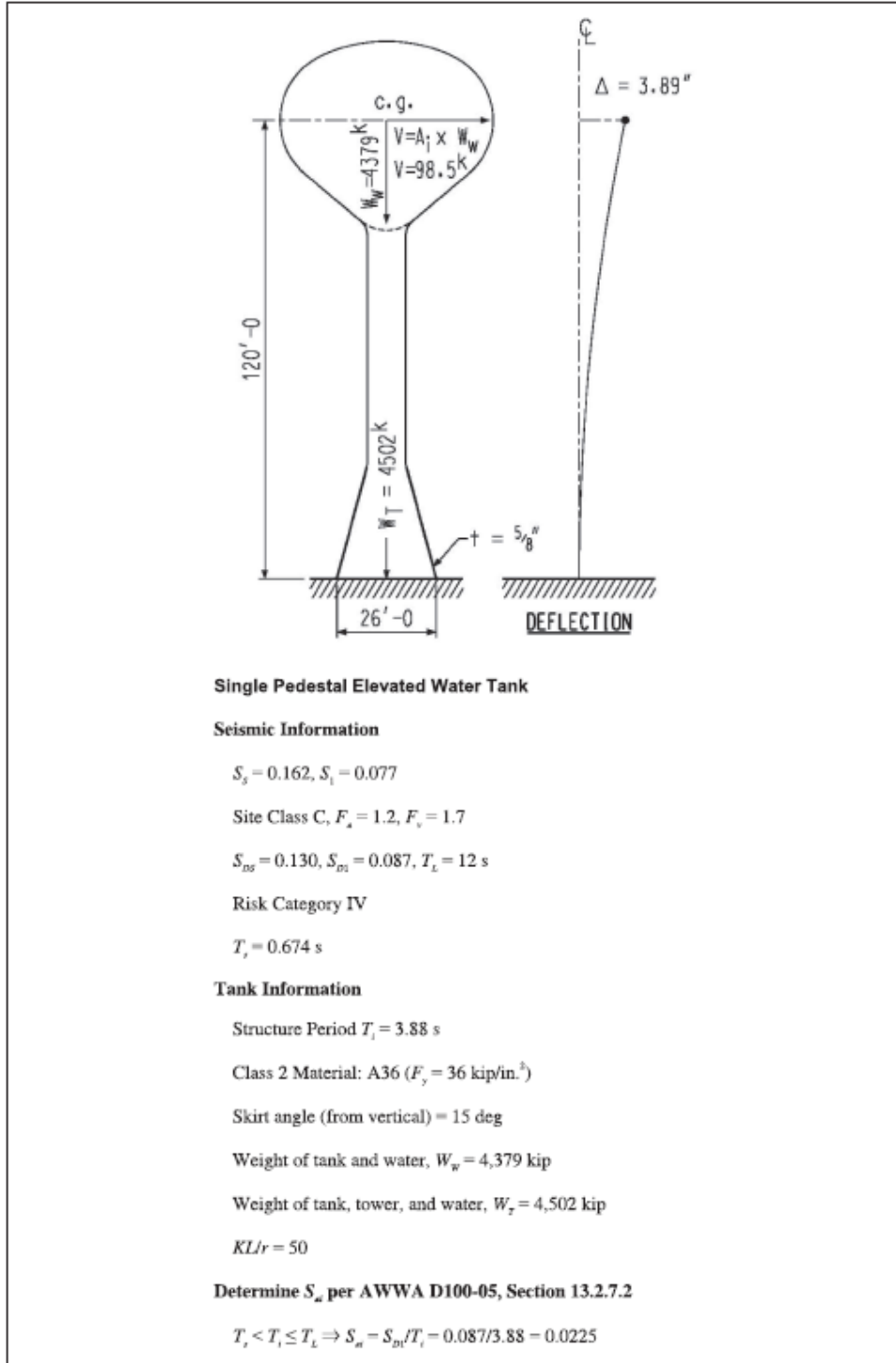
FIGURE C15.7-5 Example Problem Using AWWA D100-05, Section 13.4.3.4
