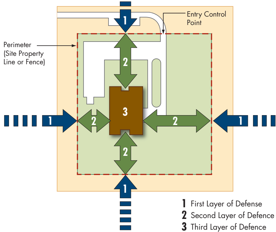
Figure 2-20: Protective barrier located on the property line to provide required standoff and onsite parking within the protected area
