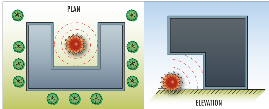
Figure 3-12: Blast waves related to building configuration
