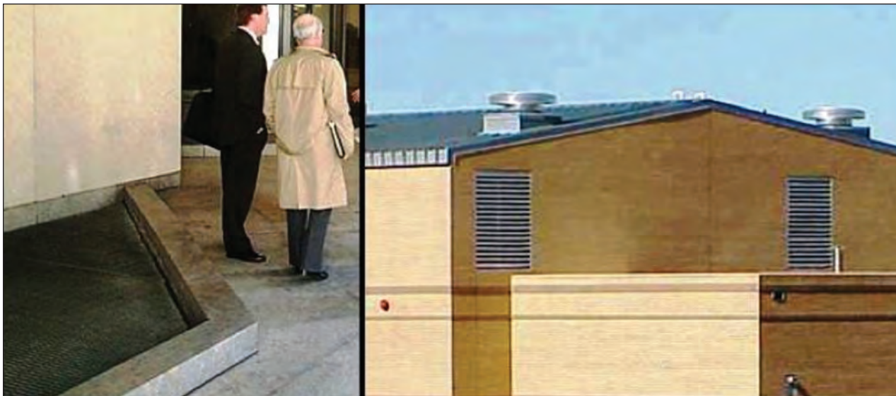
Figure 4-2: A vulnerable, ground-level intake (left); an intake elevated to the second story (right)
