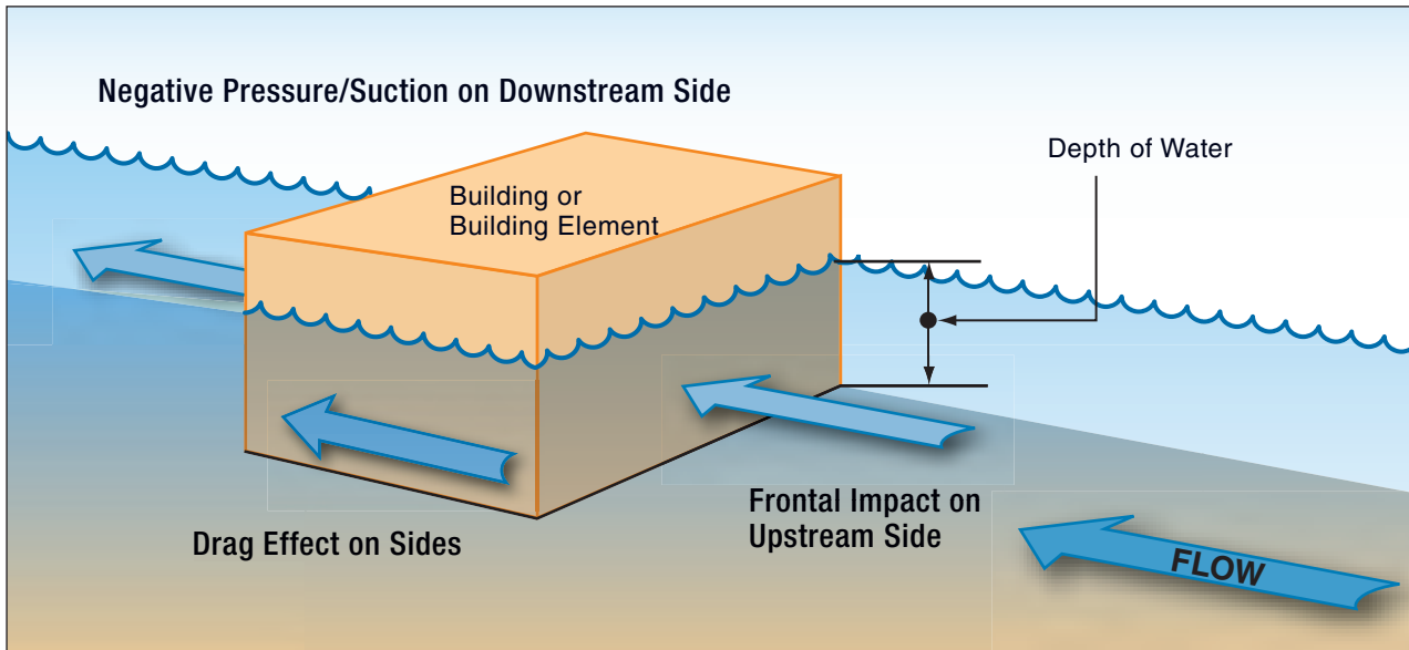
Figure 1-11: Hydrodynamic loads on a building or building element from flooding (FEMA, 2007a)
