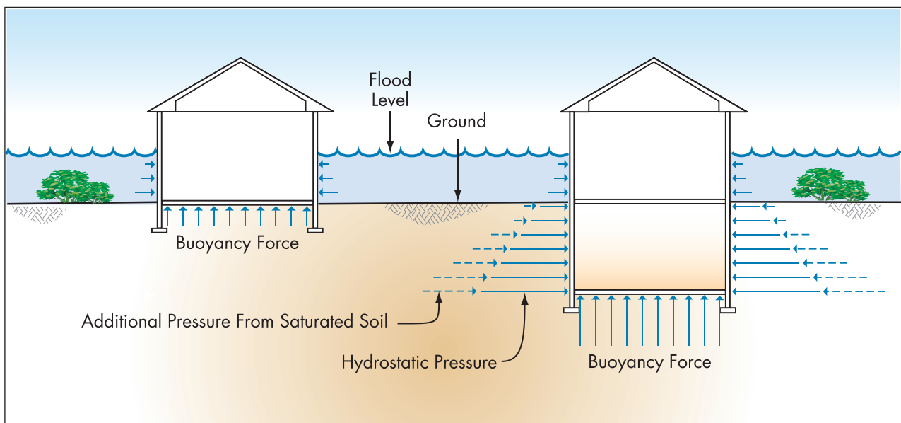
Figure 1-10. Hydrostatic loads on buildings from flooding (FEMA, 2007a)
