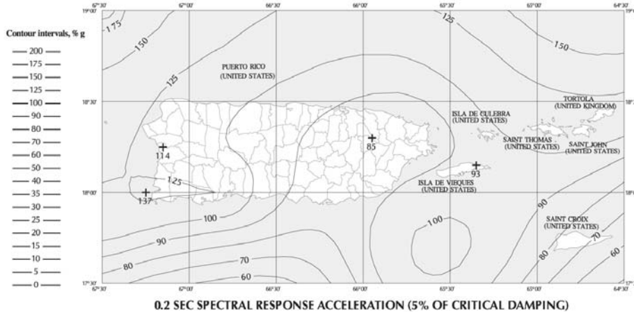
0.2 SEC SPECTRAL RESPONSE ACCELERATION (5% OF CRITICAL DAMPING)
