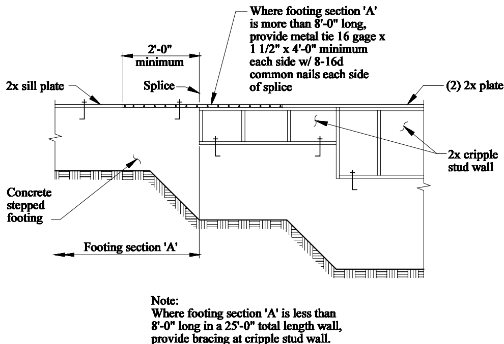
Figure 12.4-10 Detail for Stepped Foundation.
