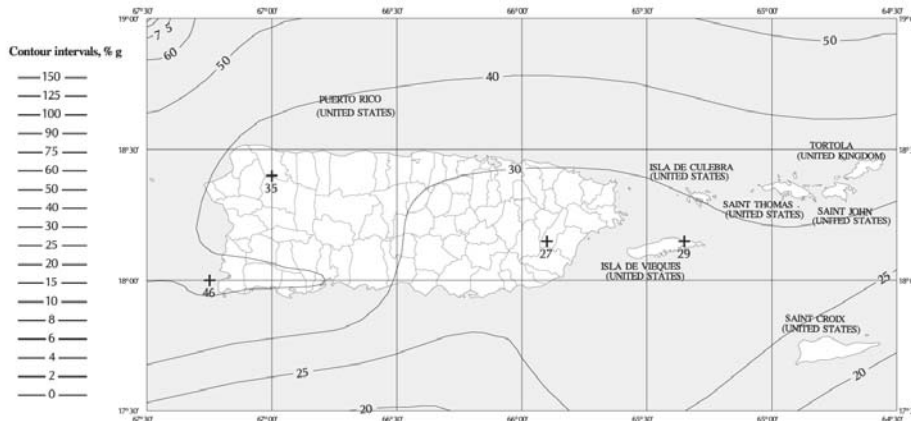
1.0 SEC SPECTRAL RESPONSE ACCELERATION (5% OF CRITICAL DAMPING)
