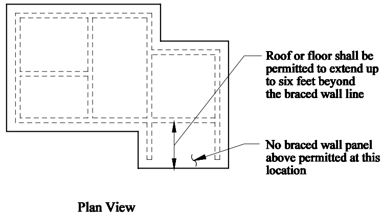
Figure 12.4-5 Permitted Diaphragm Extension.
