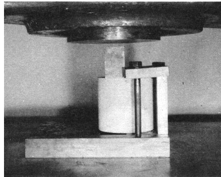
Fig. 2. Shear device in use, end view
