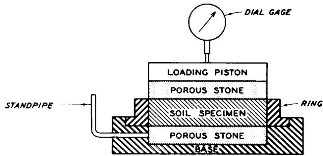
CONSOLIDATION APPARATUS
