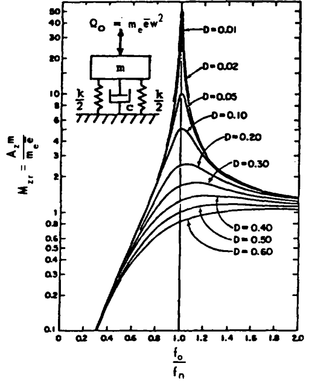
(b) ROTATING MASS EXCITATION Q = m_e e \omega^2 \sin \omega t
