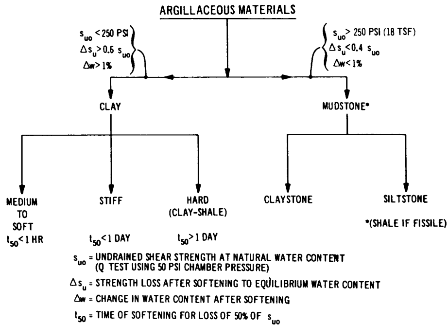
a. ENGINEERING CLASSIFICATION OF ARGILLACEOUS MATERIALS
