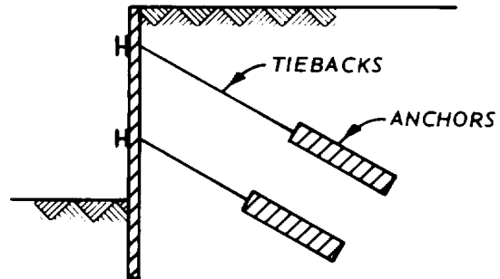
d. ANCHOR OR TIEBACK WALL
