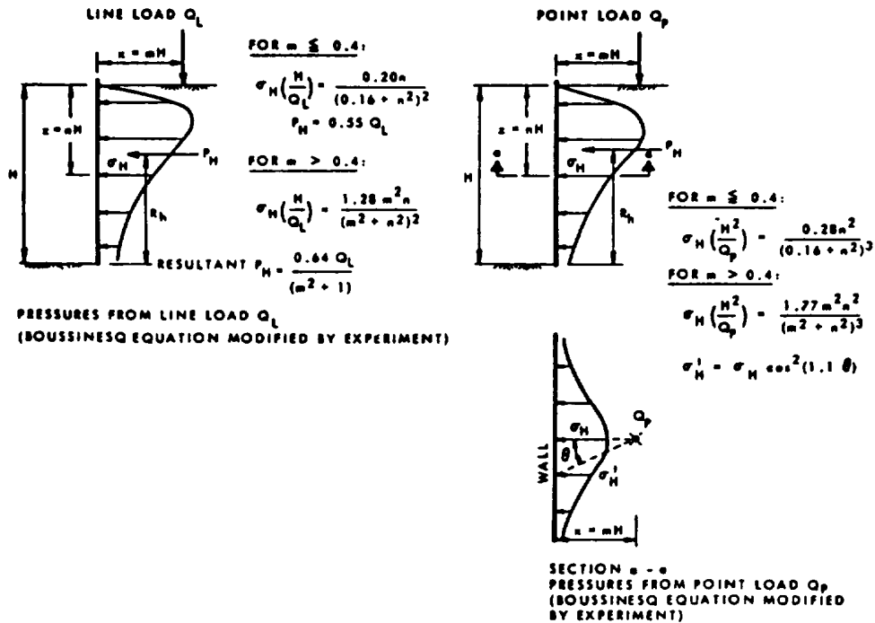
Figure 14-5. Horizontal pressures on walls due to surcharge.
