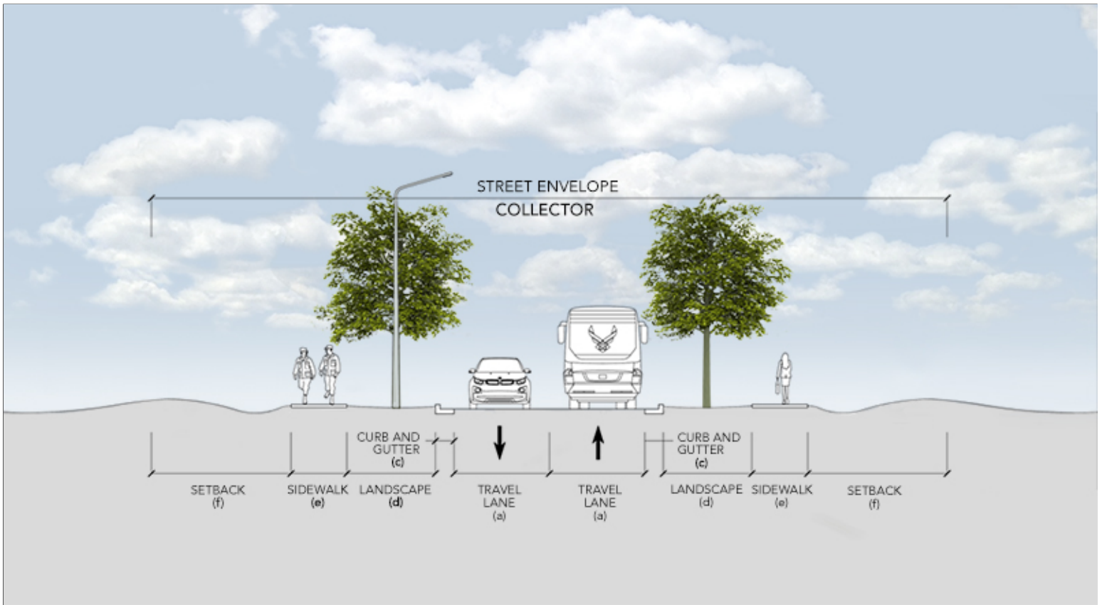
Travel Lane (a): 12' Median (b): N/A Curb and Gutter (c): 2' Landscape (d): 10' Sidewalk (e): 6' Setback (f): 15' or per AFTP requirements
