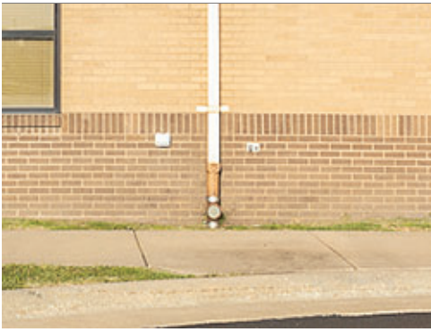
Roof Leader Connection to Storm Drainage
