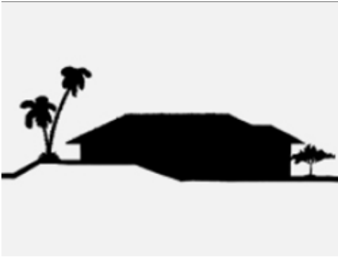
Contouring Landforms
