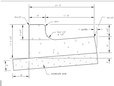
Vertical Curb and Gutter
