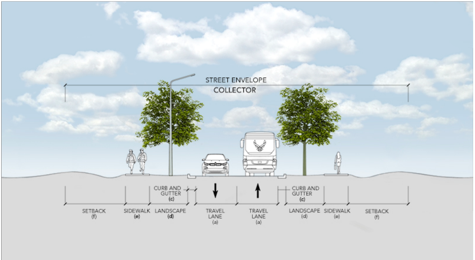
Travel Lane (a): 12'; Median (b): Not used; Curb and Gutter (c): 2'; Landscape (d): 10'; Sidewalk (e): 6'; Setback (f): Min. 15' or per AT
