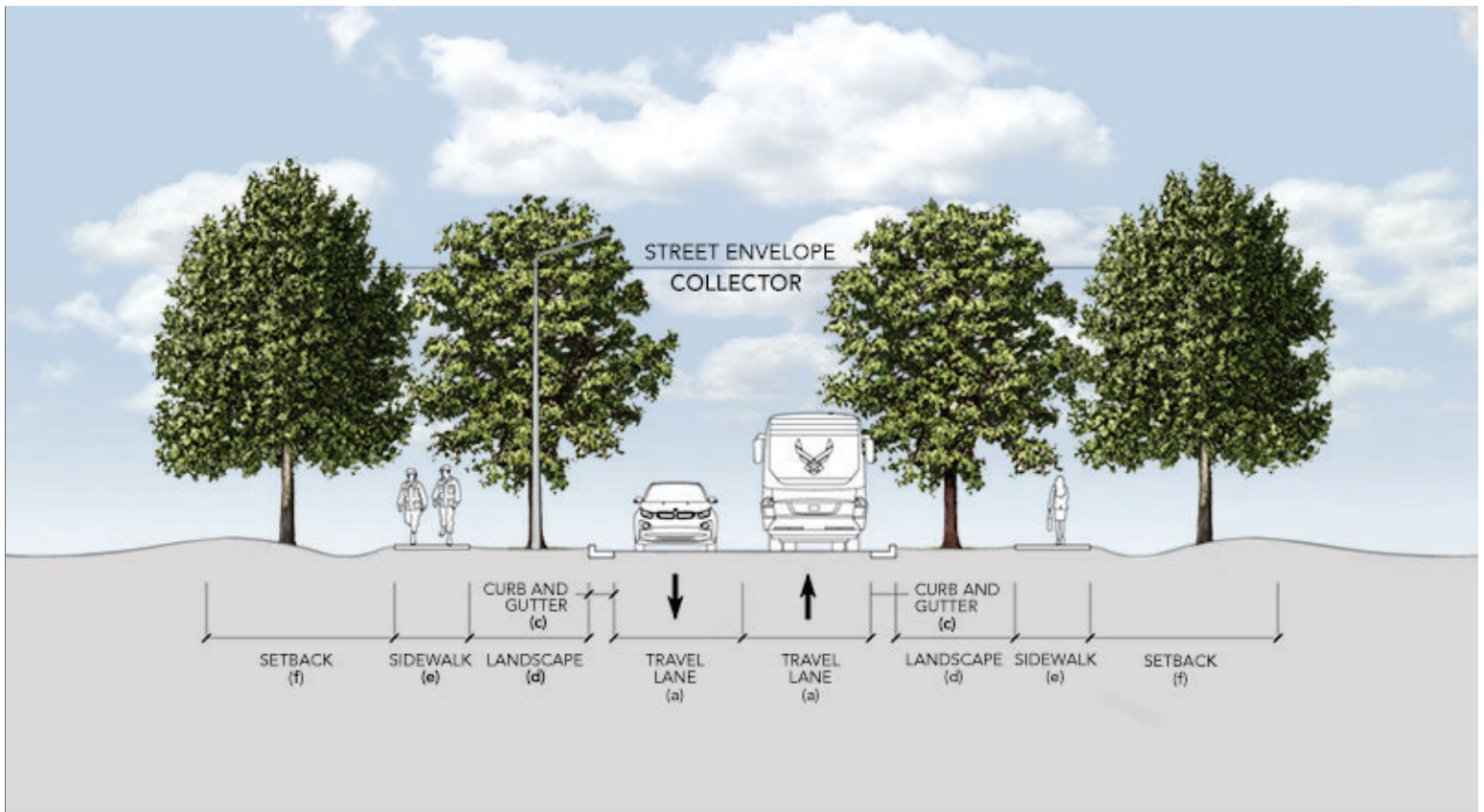
Travel Lane (a): 12' Median (b): N/A Curb and Gutter (c): 2' Landscape (d): 10' Sidewalk (e): 6' Setback (f): Min. 35' or per ATRP
