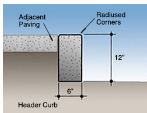
Header Curb
