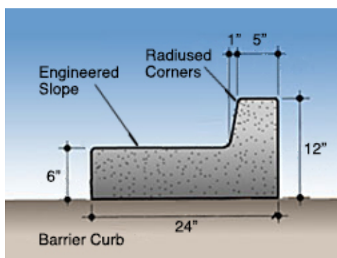
"Barrier" Curb
